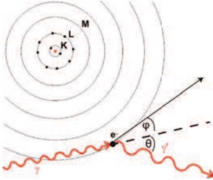
FIGURE 1.2: Effet Compton
