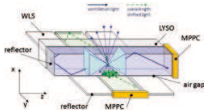
FIGURE 1.14: Concept axial de AX-PET (P. Beltrame et al. 2011 [78])
