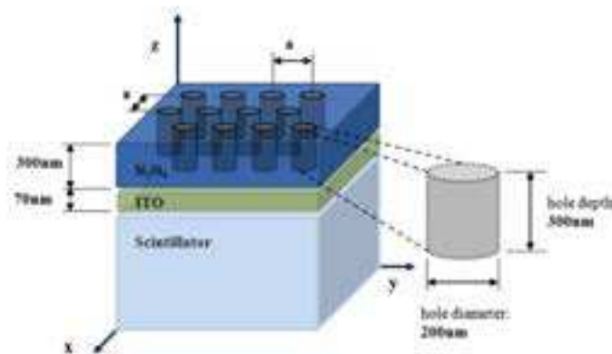
FIGURE 6.1: Exemple de structure de cristal photonique (A. Knapitsch et coll. [266])
