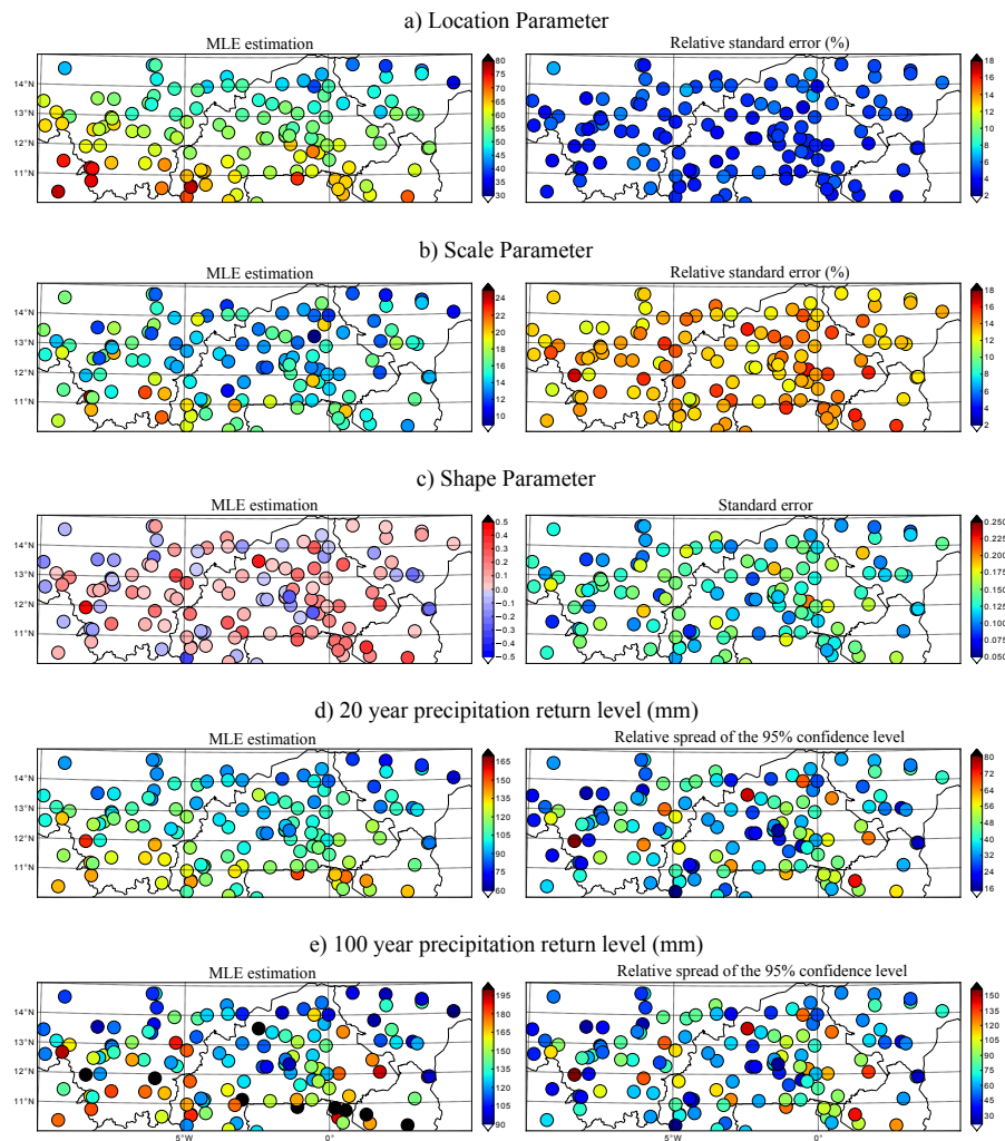
Figure 3: Point-wise estimates and standard errors of the three GEV parameters. Point-wise estimate and relative spread of the 95 % confidence level of the 20-year and 100-year return levels
