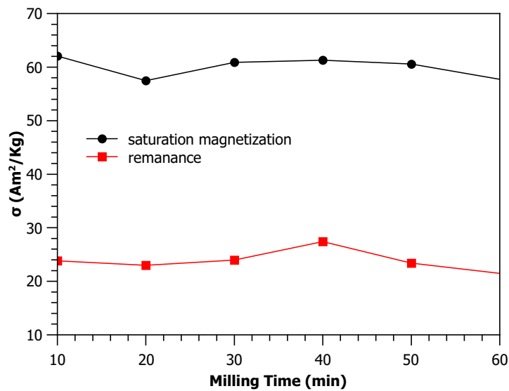
Figure 3.15: Variation in saturation magnetization and remanence for N2H800 series with milling time.
