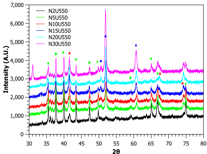
Figure 3.20: Analyzed diffraction pattern of ultrasonic mixed samples, NXU550 series, sintered 550^\circ\text{C} . The circles in green represent BaM phase; blue circles indicate permalloy phase and red show maghemite phase.
