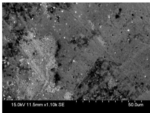
Figure 3.11: Microscope image of N10H800 – 45min , resolved to the scale of 50 micrometer. Distribution and agglomeration of permalloy particles can be seen in the image.
