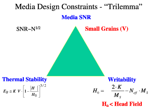
Figure 1.13: Demonstrates the 3 prominent challenges in recording technology interconnected to one another.
