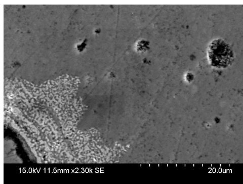
Figure 3.9: Microscope image of N2H800 , resolved to the scale of 20 micrometer. Agglomeration of FeNi particles can be seen in the image.
