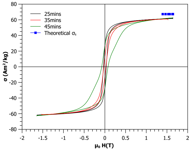
Figure 3.16: Hysteresis curve with variable milling time for N5H800 series as indicated in the label.
