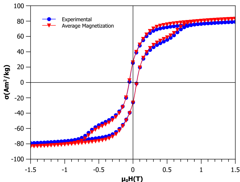
Figure 2.23: Magnetic properties of the mix of the nanopowder of Barium ferrite and Iron-Nickel . In blue, the experimentally measured curve and in red, the calculated magnetization.
