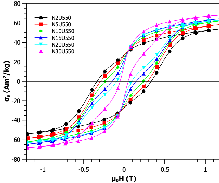
Figure 3.23: Hysteresis loop for different volume fraction X of Fe_{25}Ni_{75} in the NXU550 series, where X = 2, 5, 10, 15, 20 .
