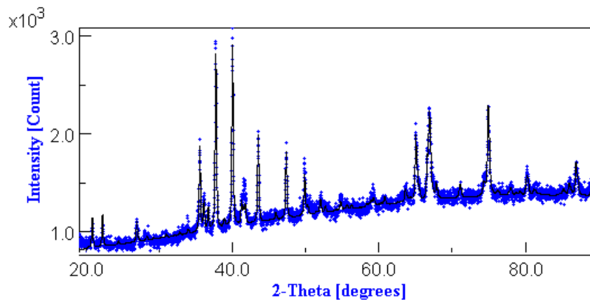
Figure 3.19: Analyzed diffraction pattern of ultrasonic mixed sintered bulk N2U550 .
