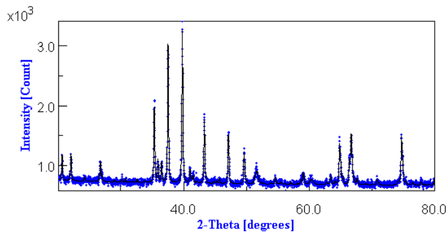
Figure 2.16: Diffraction pattern for N5H - 35min powders; after milling for 35 minutes.
