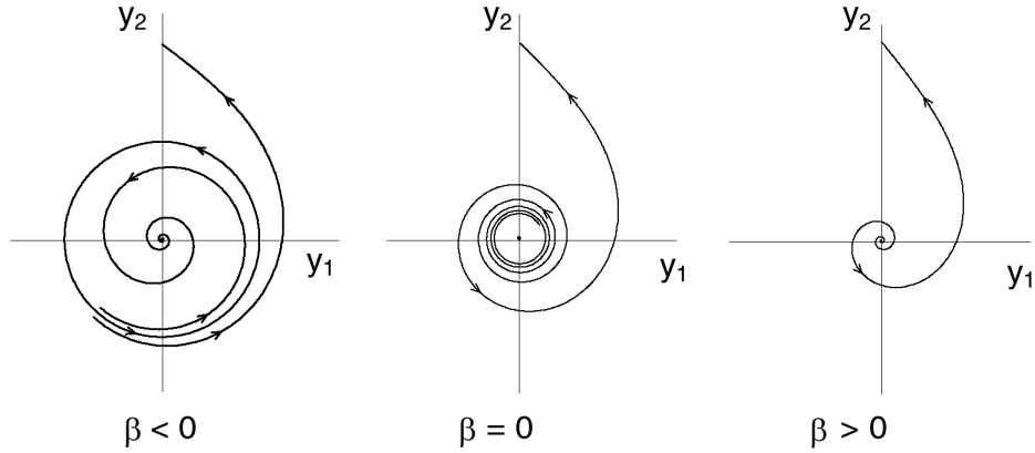
Figure 6.5: Graphical representation of the sub-critical hopf-bifurcation.
