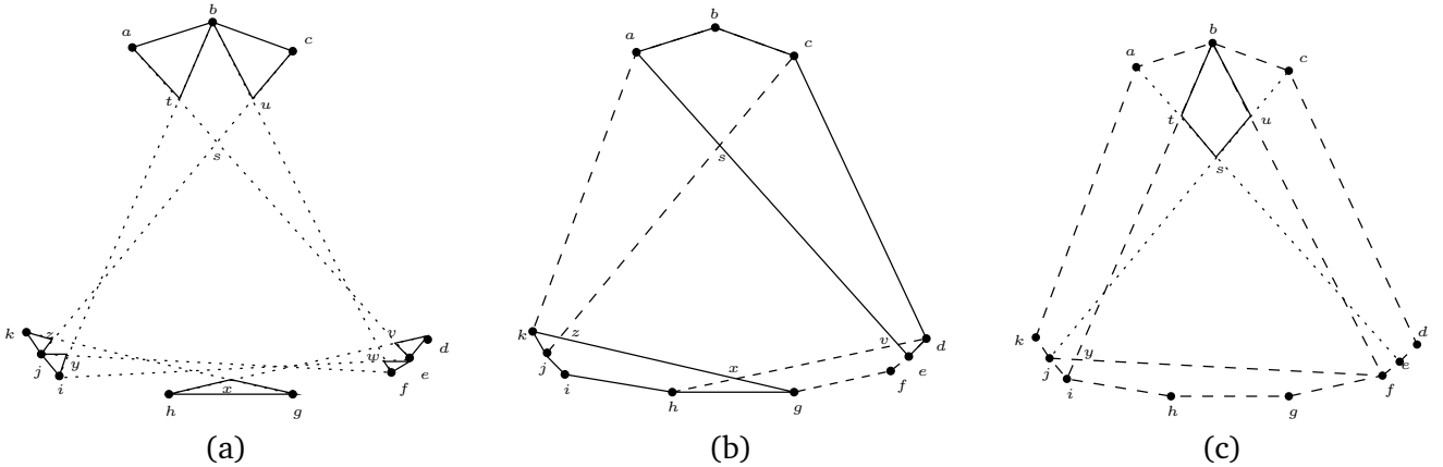
Figure 7.2: (a) One of the seven (bold) triangles contains a point of the weak \epsilon -net (b) One of the four triangles jzk , gxh , dve or asc contains a point of the weak \epsilon -net (c) jyi contains a point of the weak \epsilon -net
