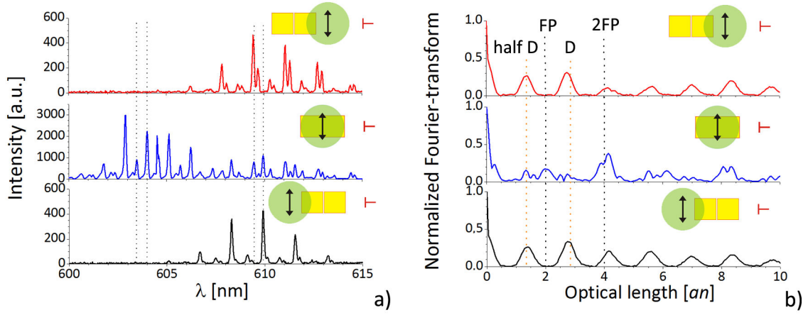
Figure I.7: Emission of the system of two closely placed micro-lasers ( 1 \mu\text{m} gap) with excitation geometry varied (indicated by the scheme next to each plot): a) emission spectra; b) normalized Fourier-transform (lengths of periodic orbits are indicated with FP and D: Fabry-Perot FP = 2an ; diamond D = 2\sqrt{2}an ). Excitation was made with the intensity of 38.5 \text{ MWcm}^{-2} with polarization orthogonal to the emission direction ( \alpha = 90^\circ ).
