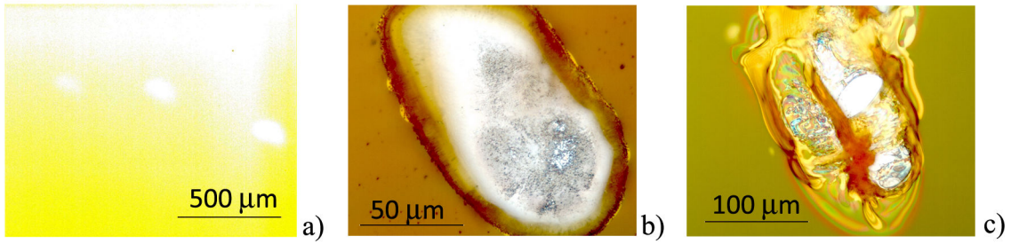
Figure 4.8: Degradation process during ASE measurements on the PMMA layer doped with 5 wt% of DCM: a) bleaching, b) beginning of polymer melting, c) propagation of polymer melting. Pump intensity about 150 \text{ MW cm}^{-2} .
