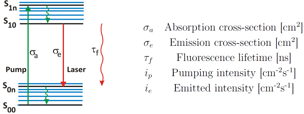
Figure 1.11: Dye molecule as a 4-level lasing system.
