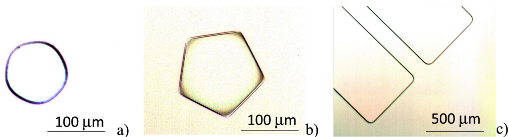
Figure A.2: Optical microscope photographs of defects caused by electron-beam lithography in the polymer layers containing Alq_3 : a,b) “pentagon” micro-cavity; c) ribbon micro-cavity. (a) was obtained with first trials and (b,c) with smaller radiation dose.
