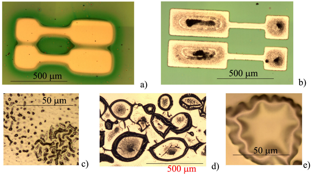
Figure J.8: Optical microscope photographs on the top contacts: a) Au deposited on the PEPI film fabricated at LPQM; b)-d) Al deposited on PEPI fabricated in glove-box. c) and e) are represent a zoom of respectively b) and d). A separation between contacts is absent on (a) due to fabrication problems with this sample, still the photograph evidences the absence of degradation on the surface of the contacts.
