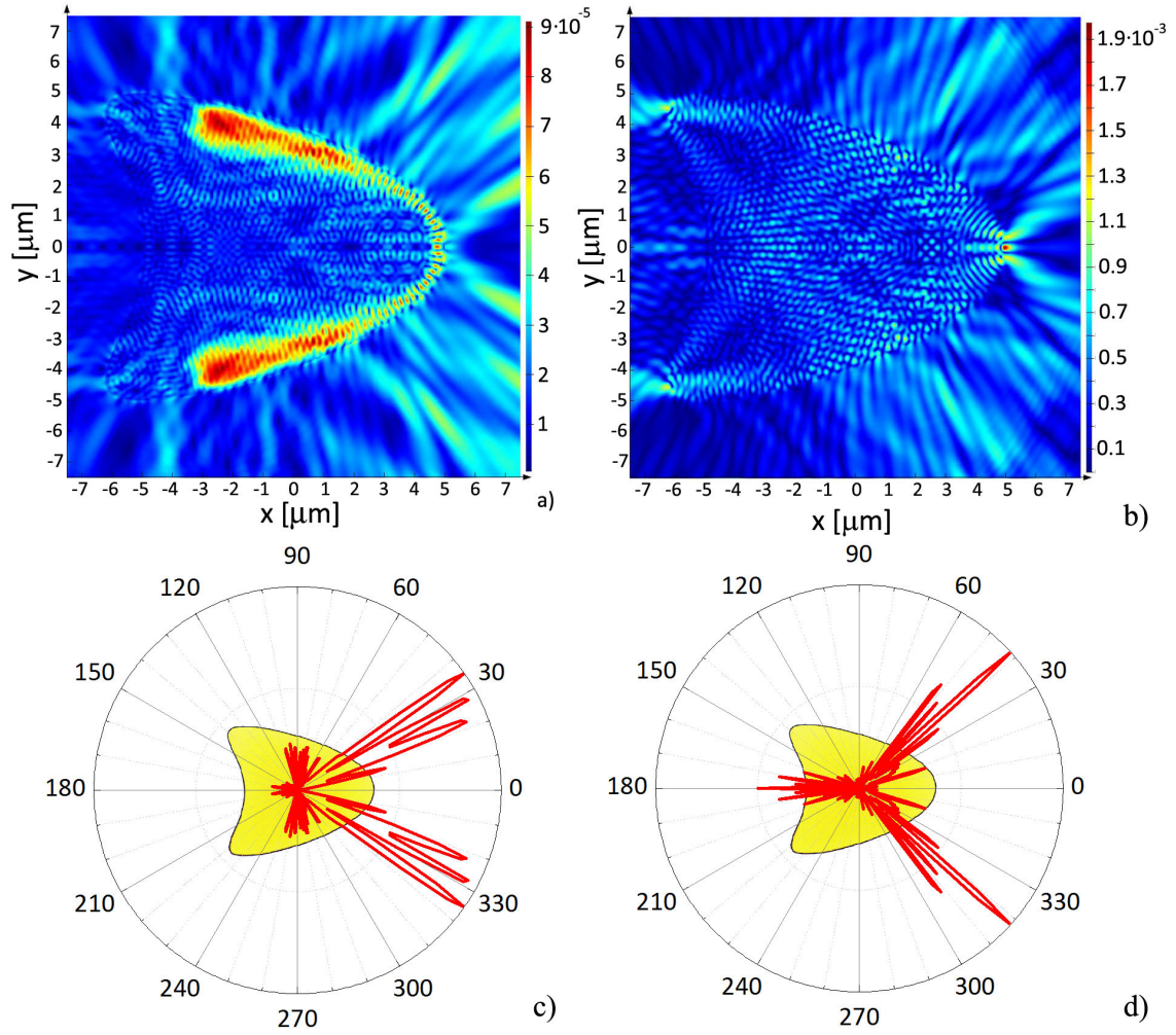
Figure G.1: FDTD simulations on 5 \mu\text{m} radius kite with \delta = 0.5 : field patterns (a,b) and emission diagrams (c,d) for TE-polarized at 611 \text{ nm} (a,c) and TM-polarized emission at 614 \text{ nm} (b,d).
