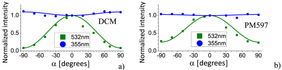
Figure 4.6: Influence of the linear pumping beam polarization on the output emission (with polarization state fixed by the Brewster plate) of a VEC SOL cavity with the gain medium provided by dye molecules: a) DCM, b) PM597; pumped at 532nm (square) or 355nm (circle). The laser emission is normalized by its value at \alpha' = 0 .
