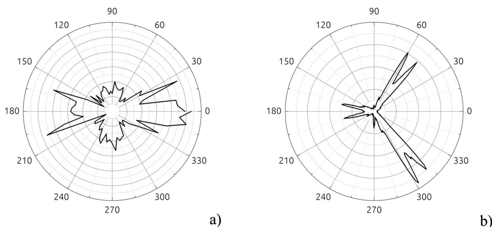
Figure 6.29: Experimental emission diagram of a 70 \mu\text{m} radius MD7-based micro-laser: a) Fabry-Perot mode; b) WGM mode.
