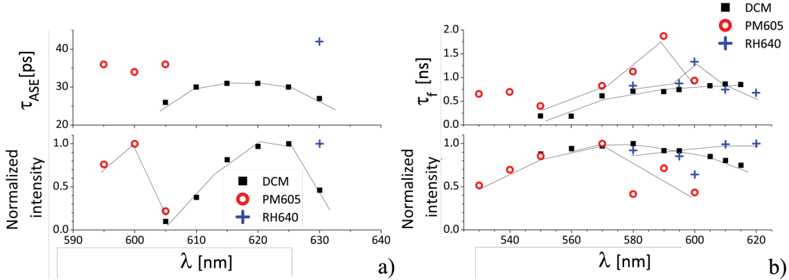
Figure 4.5: Dynamics of stimulated (a) and spontaneous (b) emission in a layer of PMMA polymer doped with 5 wt% of DCM or PM605 dye or 10% of RH640 dye. The upper frame describes the process lifetime (error \pm 1.3 ps for the ASE and \pm 60 ps for the fluorescence), and the lower one - the emission intensity for an examined wavelength, normalized by the maximum intensity in the spectrum.
