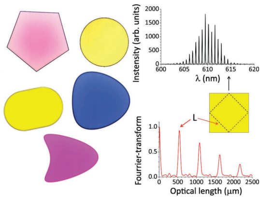
FIG. 3. (Color online) (a) Optical microscope photos of planar microlasers, which are investigated in this paper. Scales are 0.6 \mu\text{m} for the thickness and about 100 \mu\text{m} in-plane. Colors depend on the dye molecules. (b) Typical experimental spectrum of a square microlaser. (c) Fourier transform of the spectrum in (b). The position of the first peak indicates the optical length L of the periodic orbit (i.e., diamond) drawn in the inset, according to the data process described in [26].
