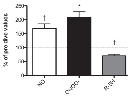
Figure 1 Evolution of nitric oxide (NO), peroxynitrite (ONOO - ) and thiols (R-SH) after repetitive breath-hold dives to 20 msw with a cumulative submergence time of 20.6 ± 1.5 min; results are expressed in percentage of pre-dive values (* P = 0.0012 ; † P = 0.0002 )
