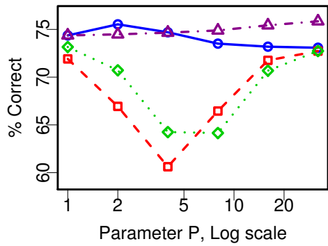
(c) 512 codewords
