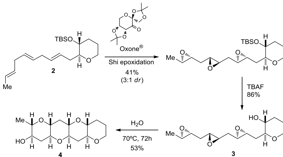
Scheme 2. 2
