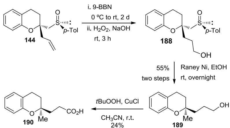
Scheme 3. 11
