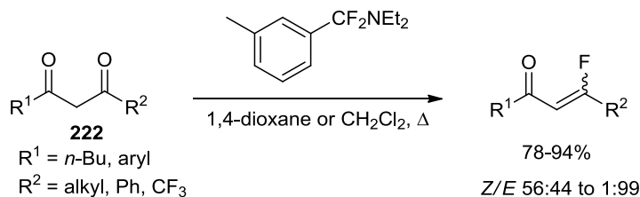
Scheme 3. 22
