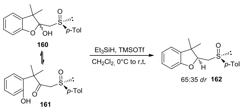
Scheme 2.53
