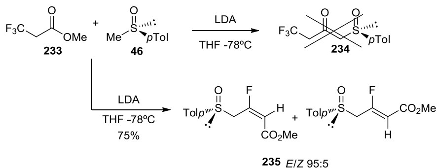
Scheme 3. 32
