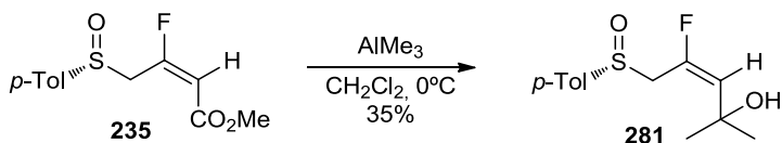
Scheme 3. 55
