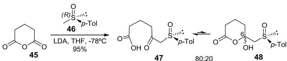
Scheme 2. 17
