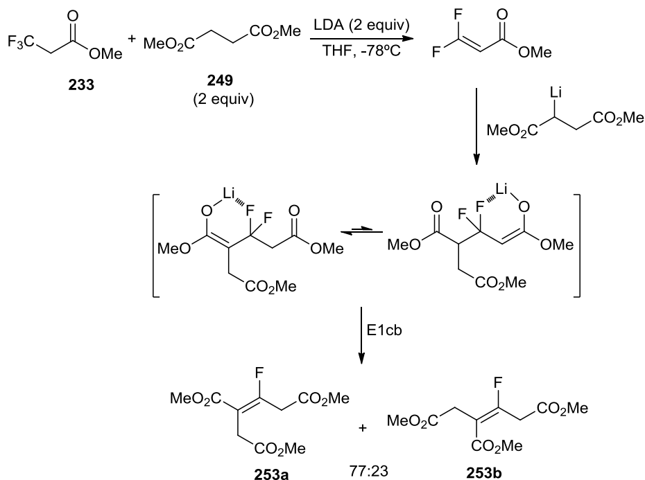
Scheme 3. 35
