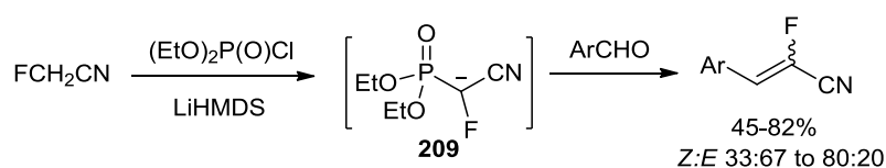
Scheme 3. 9
