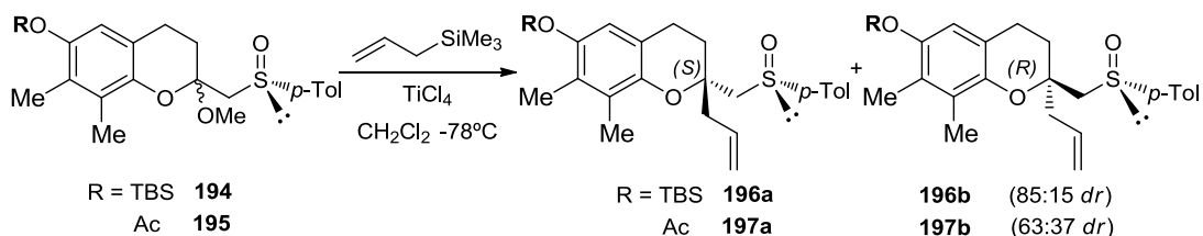
Scheme 3. 14
