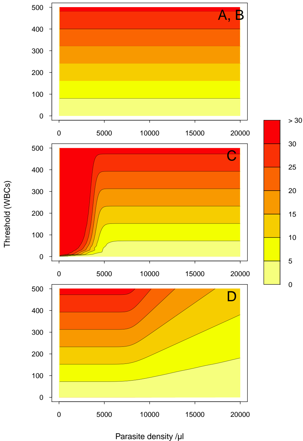
Figure 4.4: Cost-effectiveness colormap.
