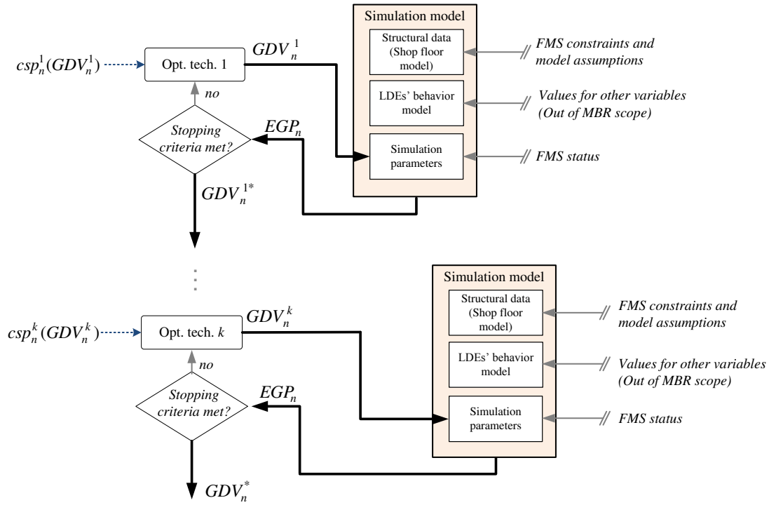
Figure III-6: Decoupled connection between optimization techniques
