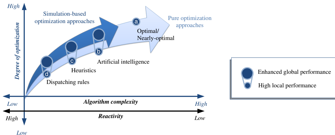
Figure I-3: Scheduling algorithms
