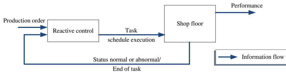
Figure D-1: Fully reactive control
