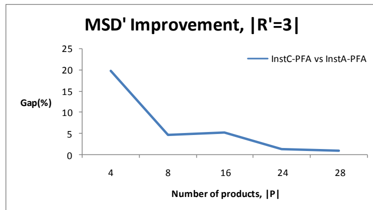
Figure V-21: Gap between the two problem instances, C and A
