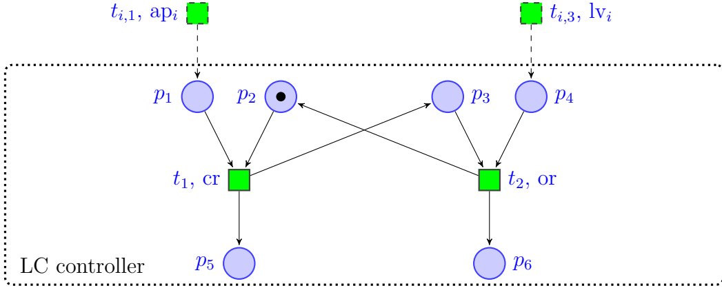
Figure 3: The LPN model for LC controller
