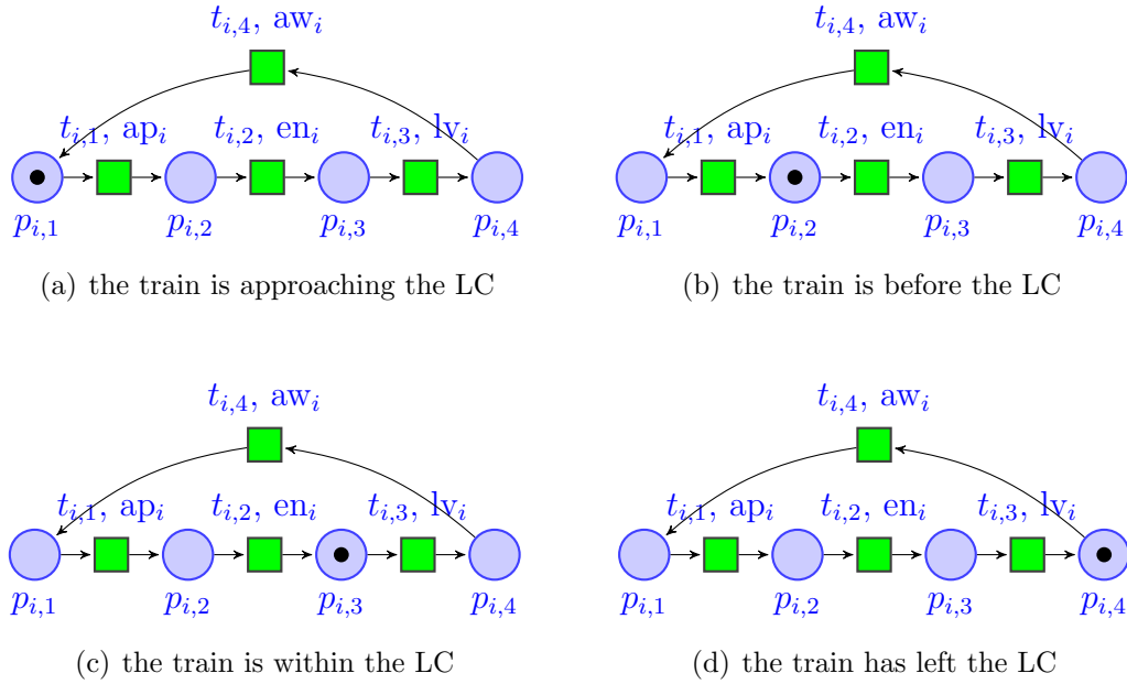
Figure 2: The LPN model for a train passing an LC
