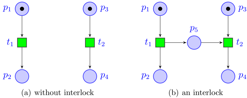
Figure 4: The PN model for an interlock
