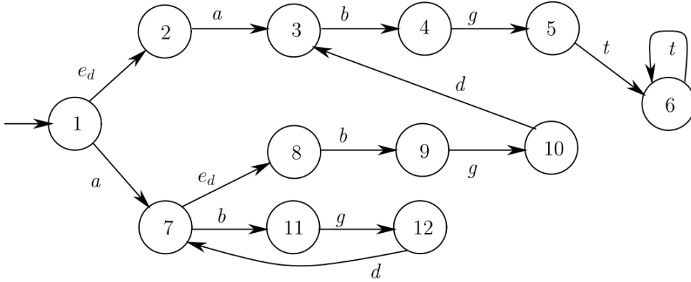
(a) An example of automaton [Cassandras and Lafortune, 2007]
