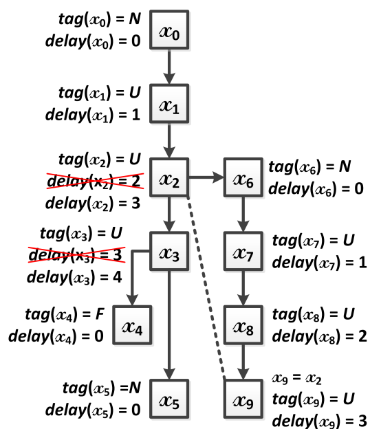
(b) The FM-set tree after generating node x_9
