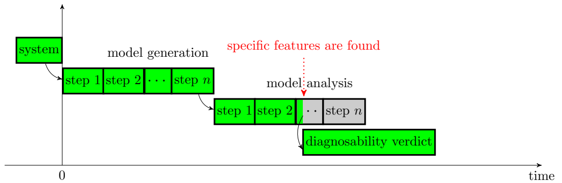
(b) Two-stage on-the-fly analysis
