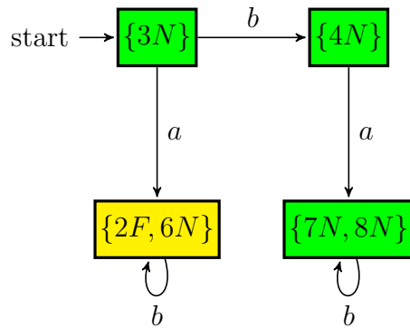
(a) G
