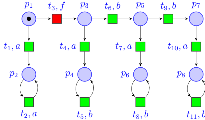
Figure 4.16: LPN N_L
