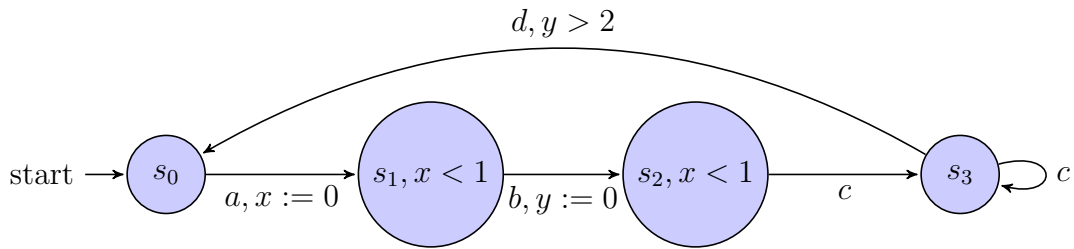
Figure 2.7: An example of timed automaton
