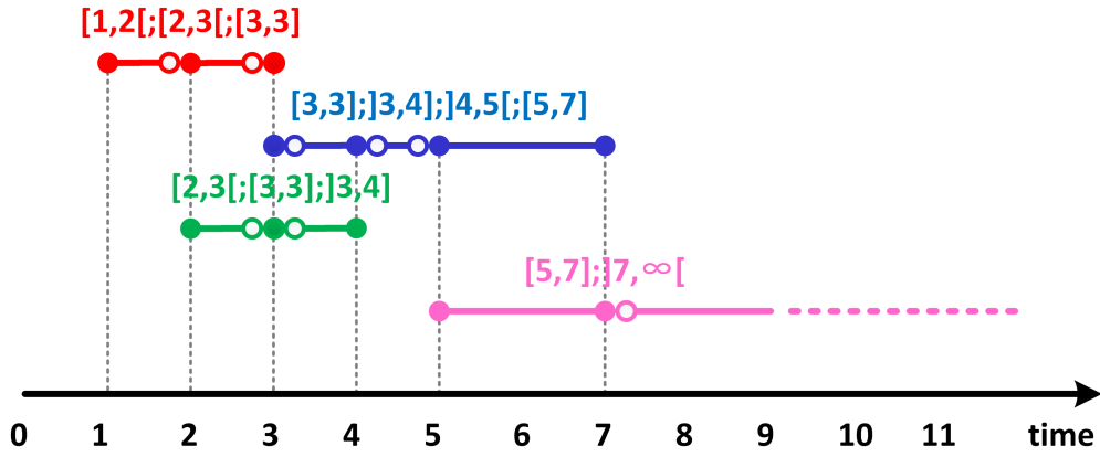
(b) Splitting intervals of A to compute BIS(A)
