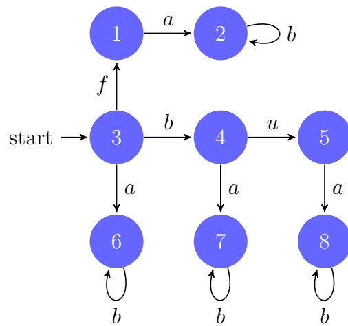
(a) G
