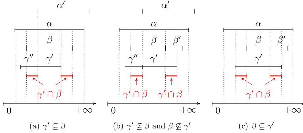
Figure 5.3: The relation between \beta and \gamma'
