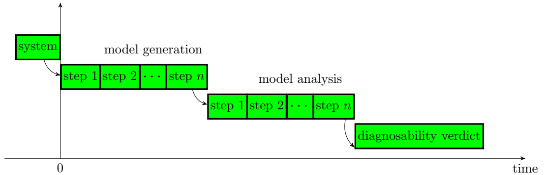
(a) Two-stage enumerative analysis
