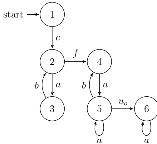
Figure 2.1: An example of automaton
