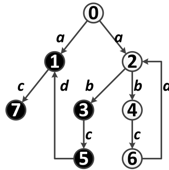
(c) FM-graph
