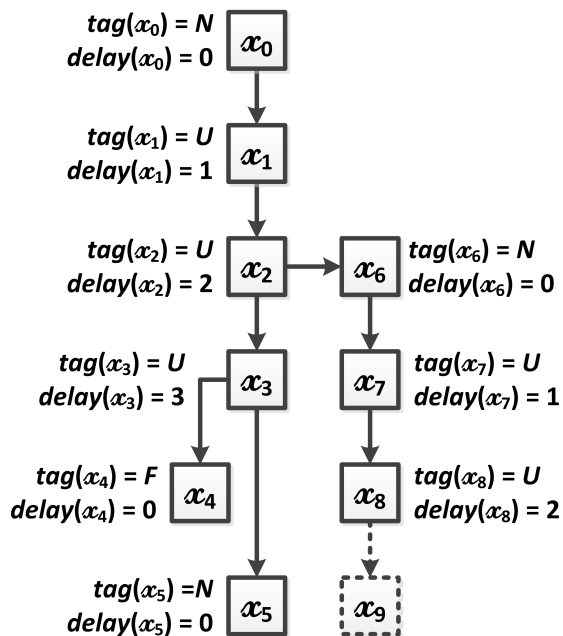
(a) The FM-set tree after generating node x_8
