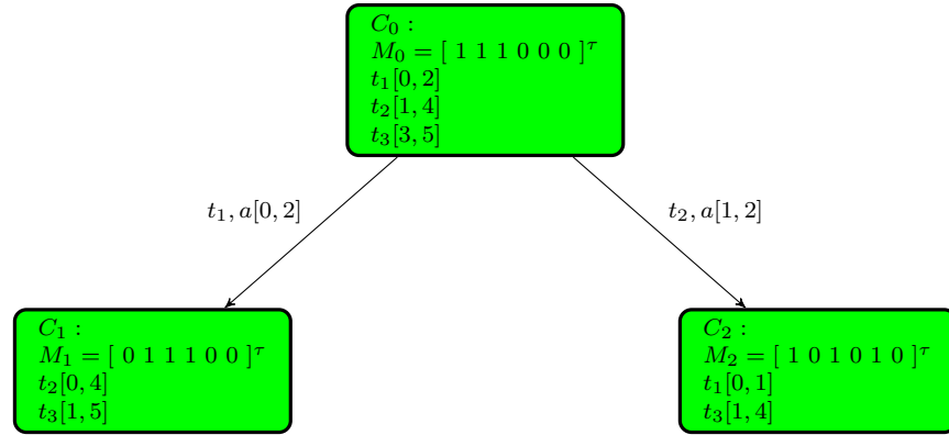
(b) A part of the state class graph of N_{LT}
