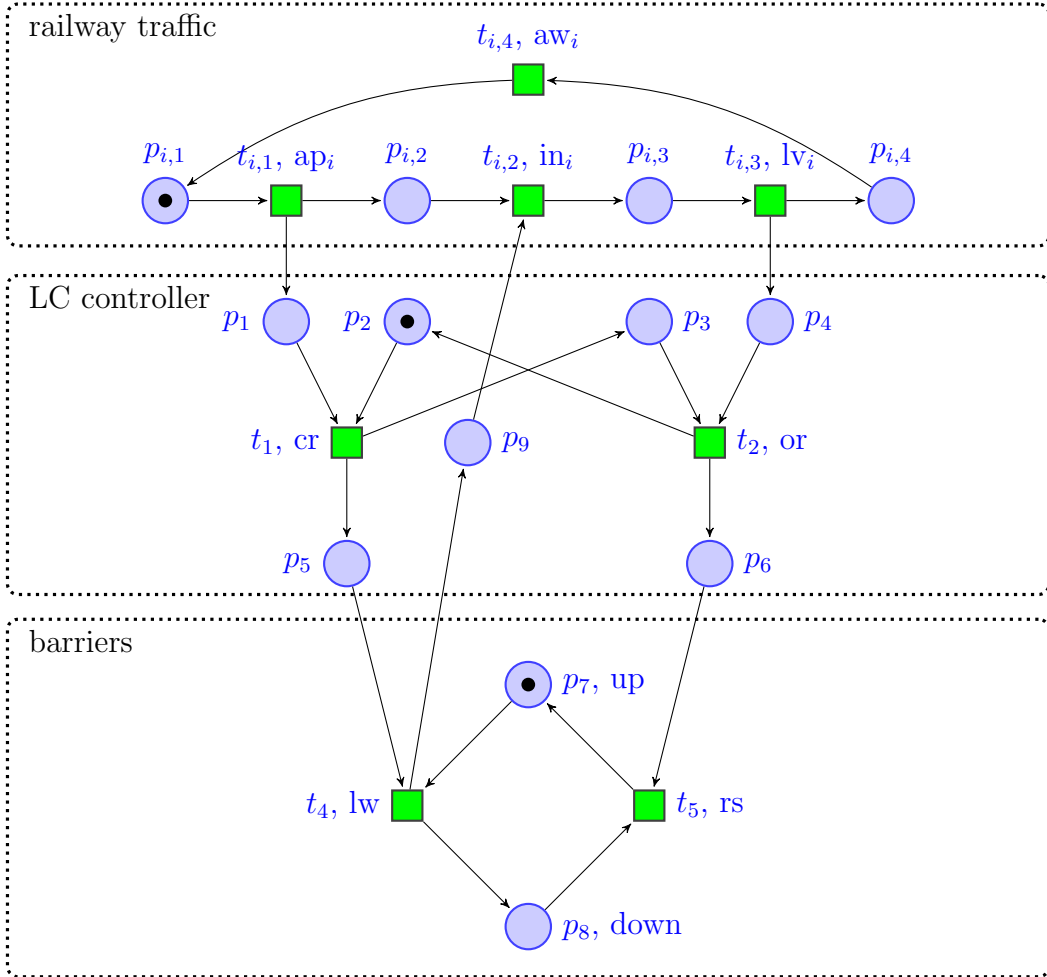
Figure 6: A single-line LC
