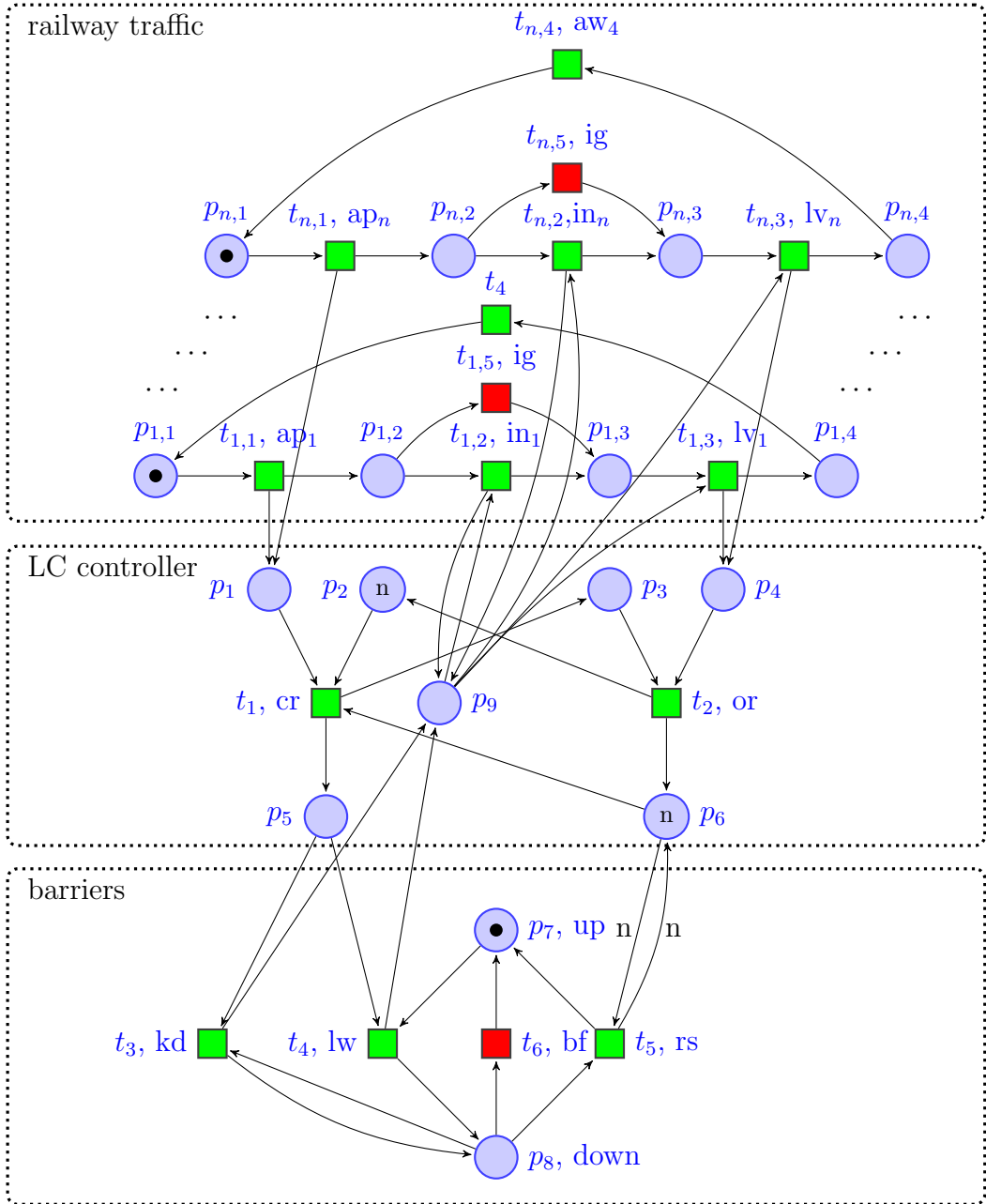
Figure 8: n -line LC benchmark
