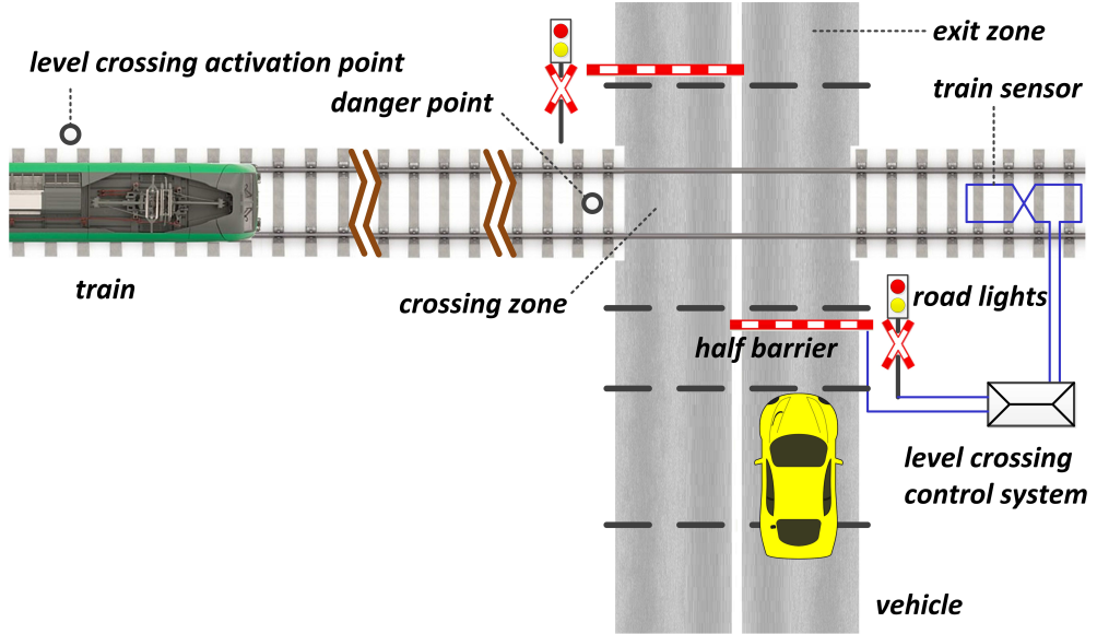
Figure 1: The construction of a single-line track LC system
