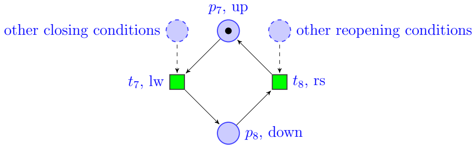
Figure 5: The LPN model for a barrier system
