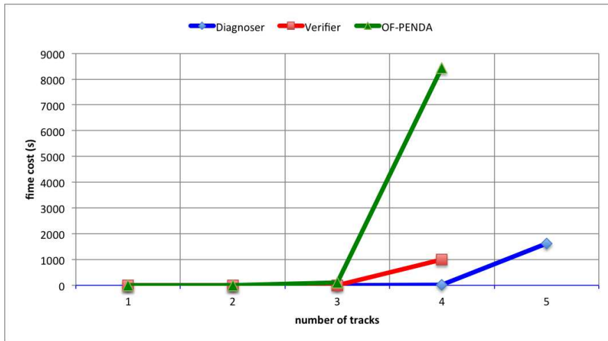
Figure 4.21: Time cost for the diagnosability analysis on \Sigma_{F2}
