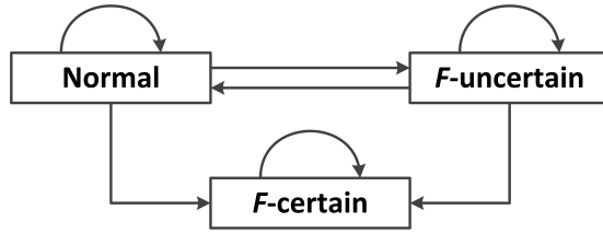
Figure 4.8: Fault propagation between FM-sets
