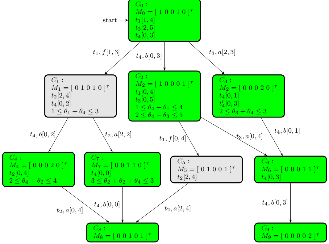
Figure 5.8: The state graph of the LTPN in Figure 5.7
