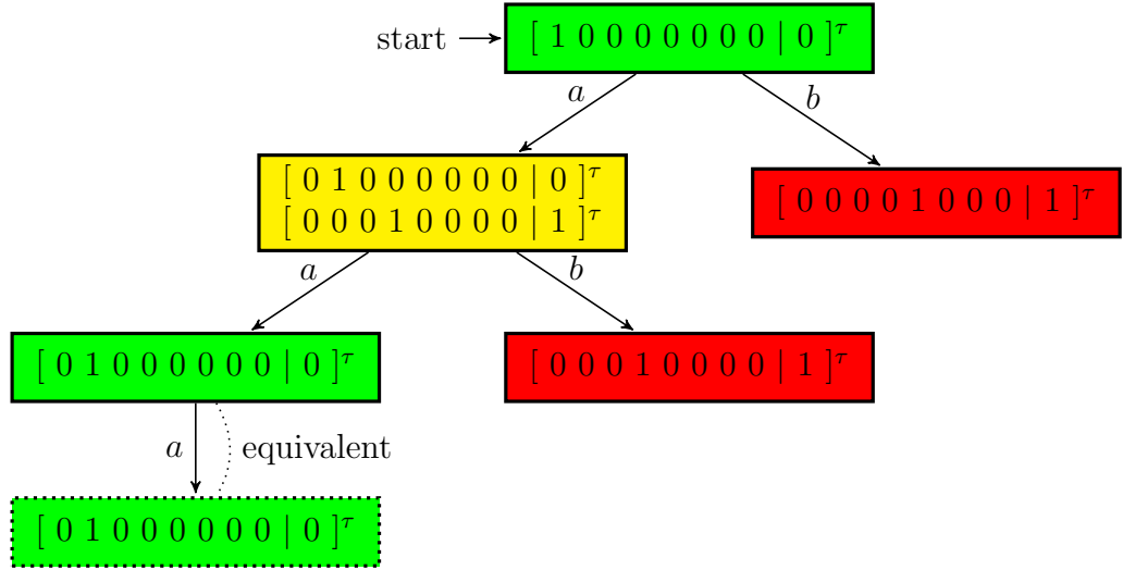
Figure 4.17: The FM-set tree of N_L
