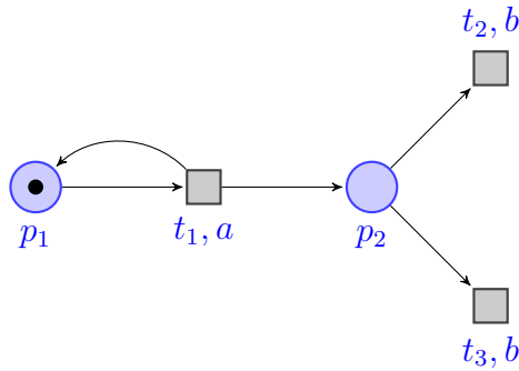
Figure 2.6: An example of LPN
