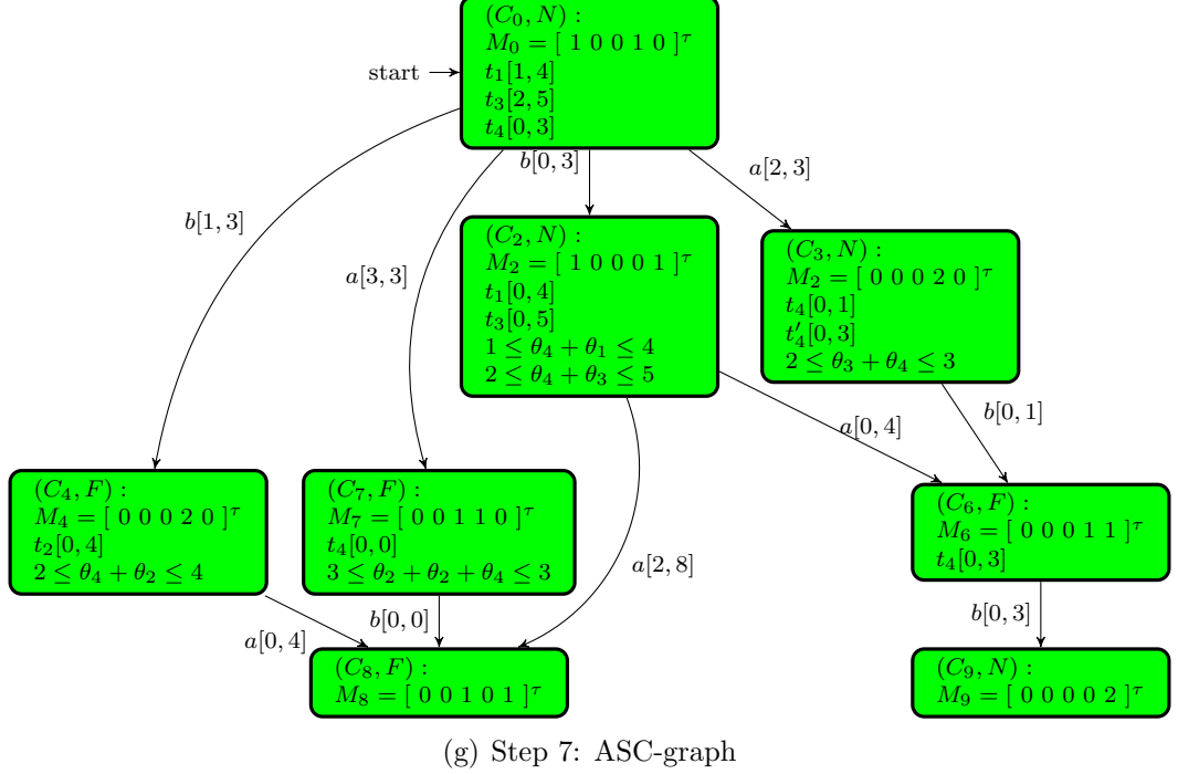
Figure 5.9: The construction of ASC-graph (Continued)
