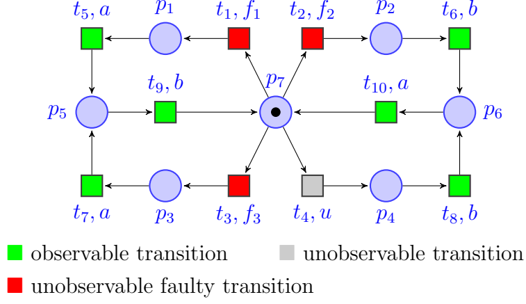
Figure 4.4: An LPN
