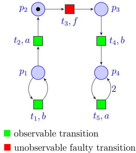
Figure 4.3: An unbounded PN
