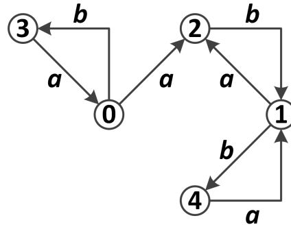
(a) FM^1 -graph
