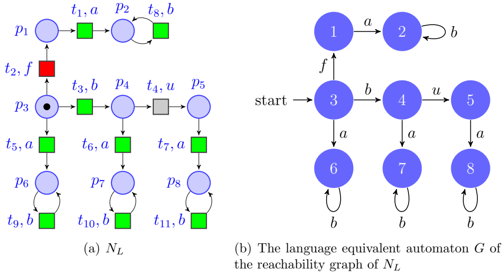
Figure 4.13: LPN N_L and its reachability graph G
