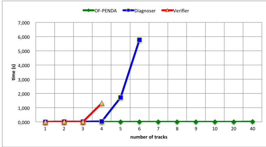
Figure 4.20: Time cost for the diagnosability analysis on \Sigma_{F1}
