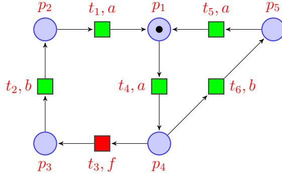
Figure 3.2: A diagnosable LPN with 2 minimal T-invariants w.r.t the same observable projection
