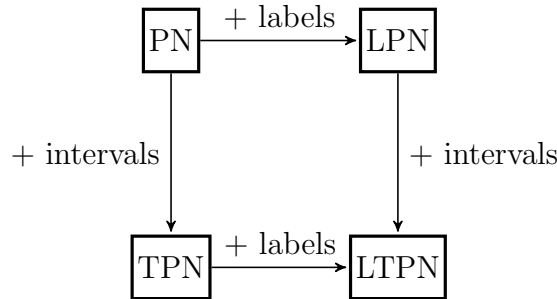
Figure 2.9: Relation between LTPN and PN, TPN, LPN
