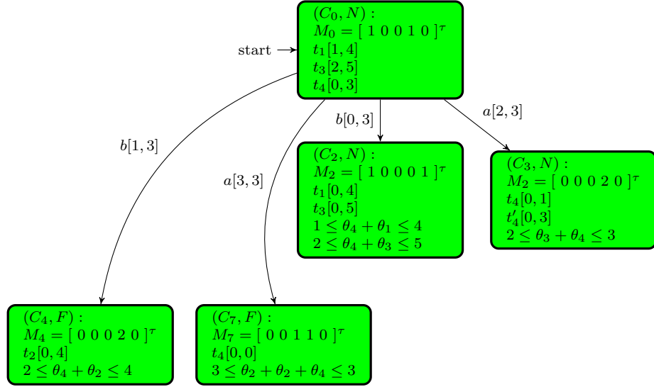
(c) Step 3
