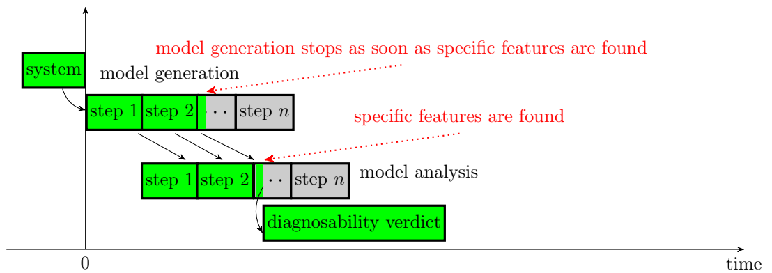
(c) Two-stage parallel and on-the-fly analysis
