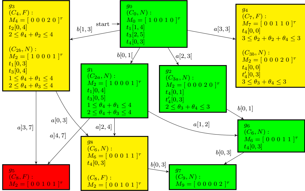
Figure 5.11: The ASG for Example 35
