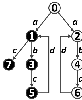
(b) FM-graph
