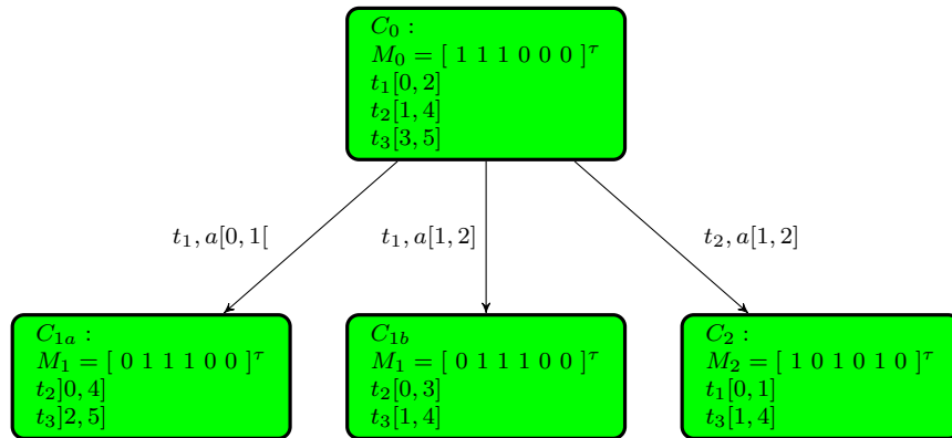
(c) A part of the modified state class graph of N_{LT}
