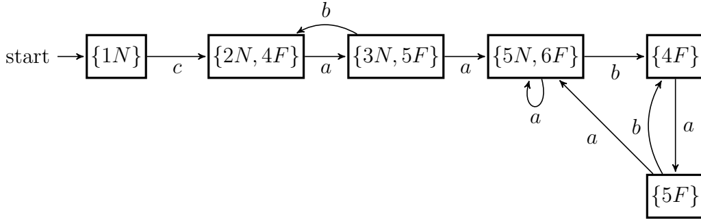
Figure 2.3: The diagnoser of the automaton in Figure 2.1
