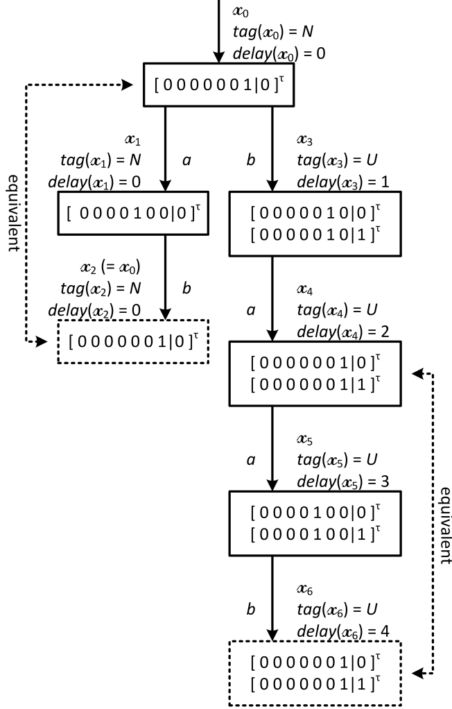
Figure 4.12: Solution process of K -diagnosability for \Sigma_{F_2}
