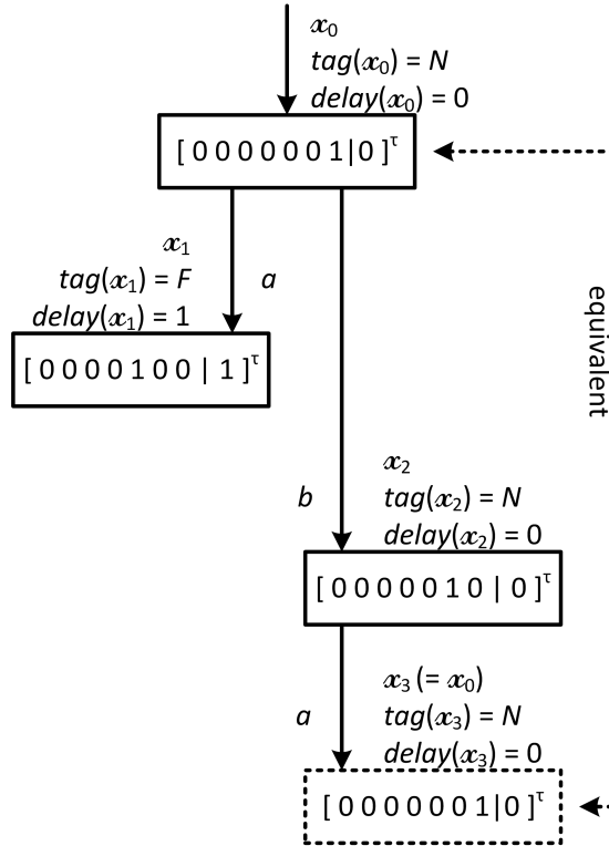
Figure 4.11: Solution process of K -diagnosability for \Sigma_{F_1}
