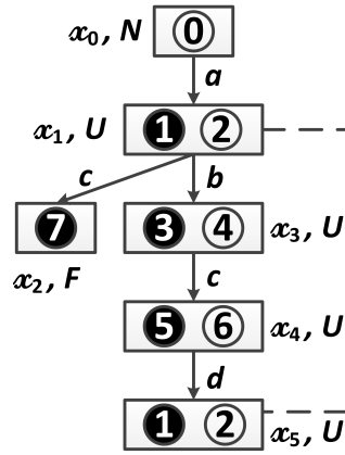
(a) FM-set tree
