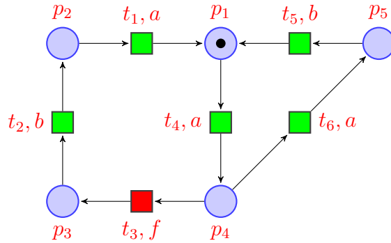
Figure 3.2: A diagnosable LPN with 2 minimal T-invariants w.r.t the same observable projection
