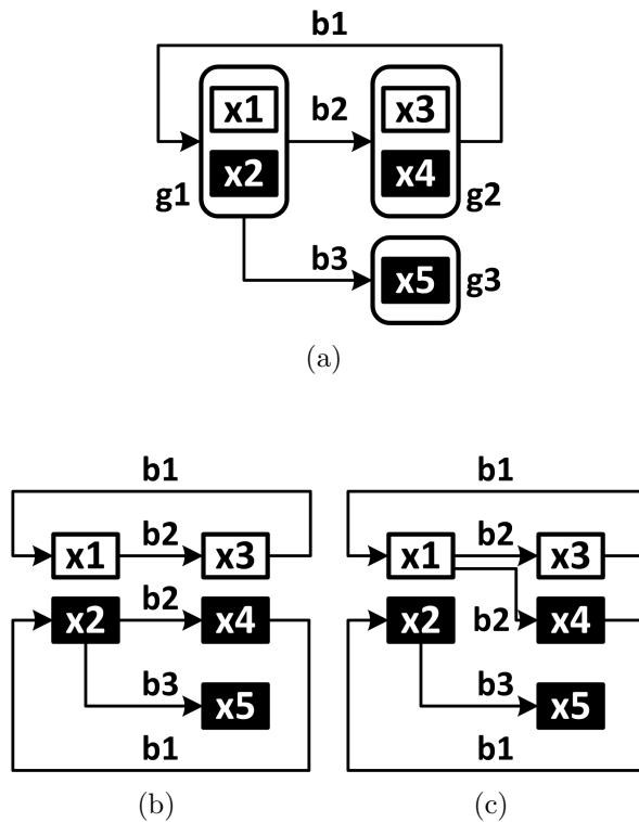
Figure 5.12: Illustration of indeterminate cycle
