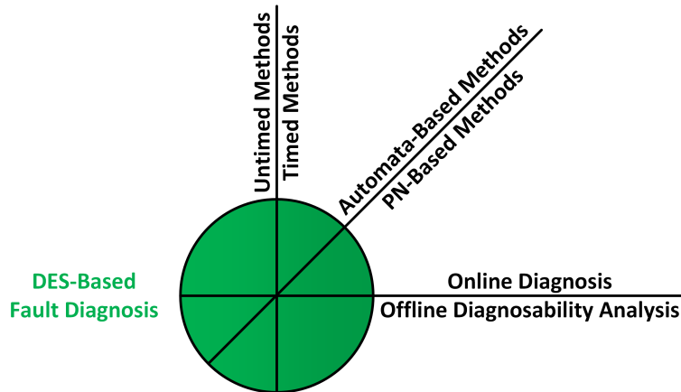
Figure 3.1: DES-based fault diagnosis
