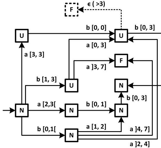
Figure 5.14: Diagnoser of the LTPN in Figure 5.7
