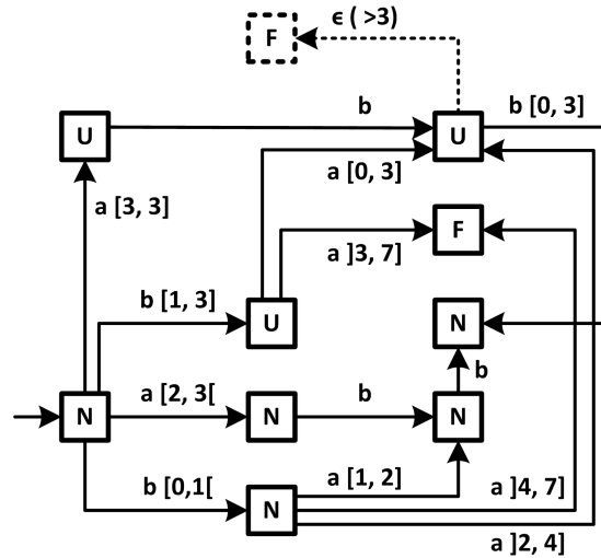
Figure 5.15: The MLTD of the LTPN in Figure 5.7
