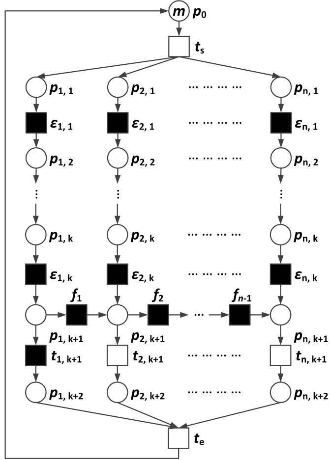
Figure 4.19: The WODES diagnosis benchmark
