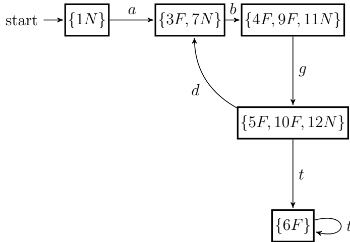
(b) The diagnoser of the automaton in 2.4(a)
