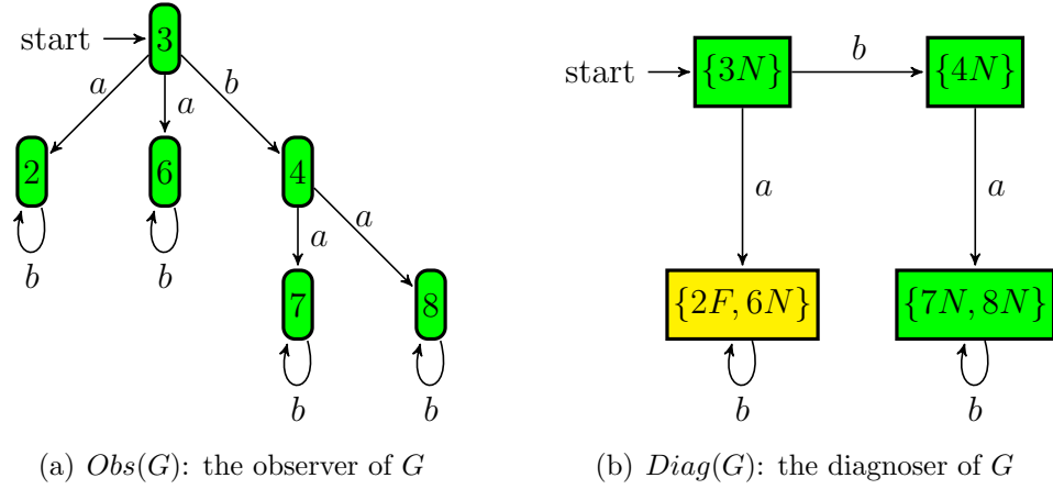
Figure 4.14: The observer and diagnoser of G
