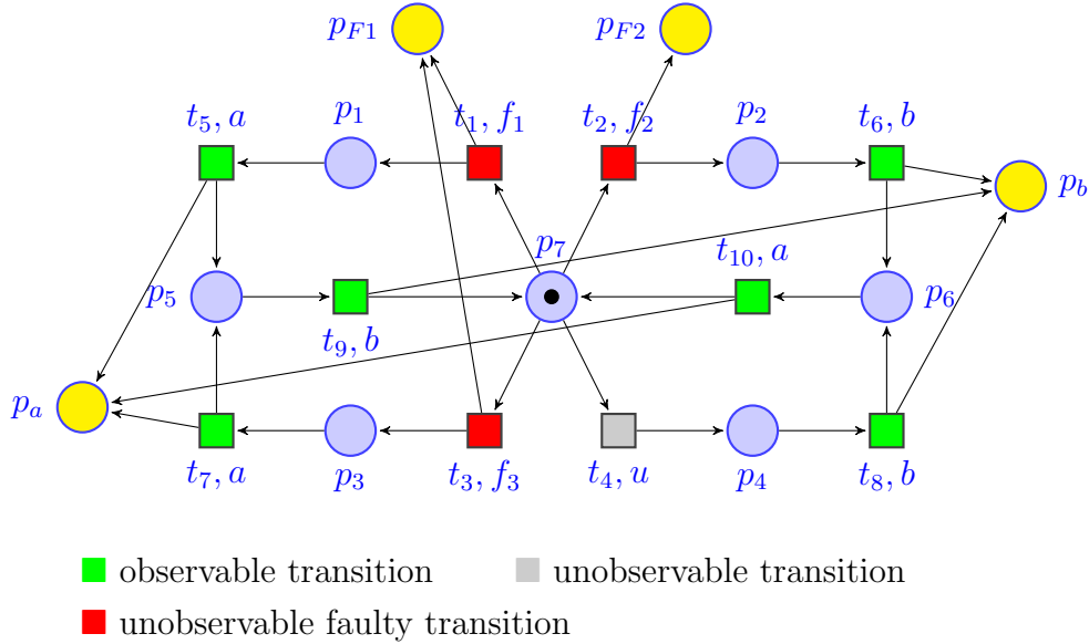
Figure 4.5: A LPN-EC
