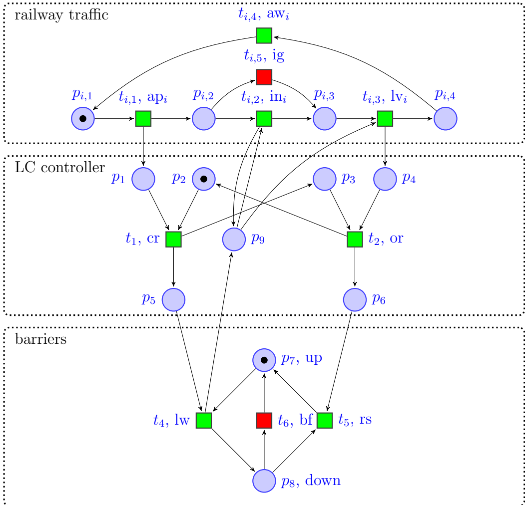
Figure 7: A single-line LC with two classes of faults
