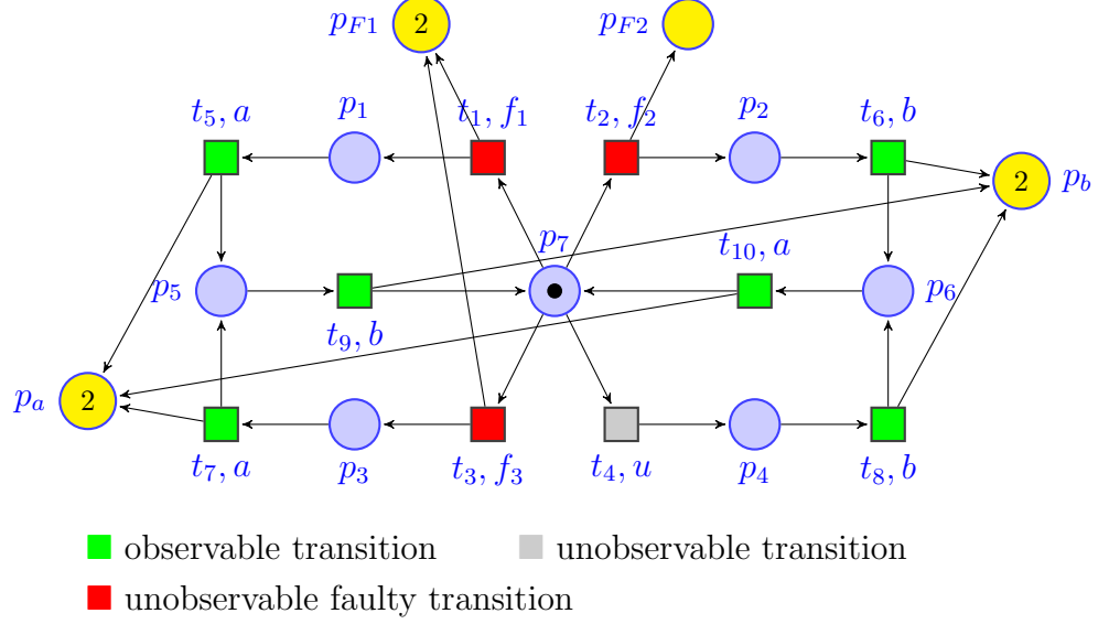
Figure 4.6: The reached marking of the LPN-EC in Figure 4.5 by the firing of t_1 t_5 t_9 t_3 t_7 t_9
