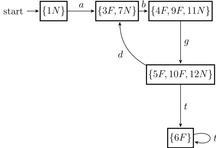
(b) The diagnoser of the automaton in 2.4(a)
