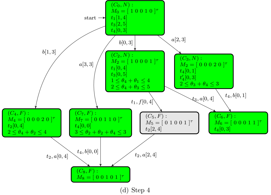
Figure 5.9: The construction of ASC-graph (Continued)
