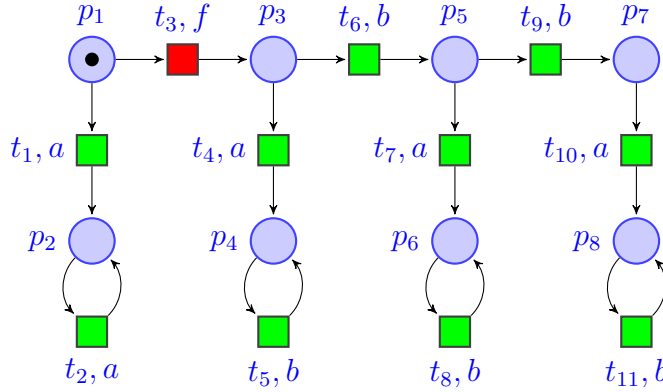
Figure 4.16: LPN N_L
