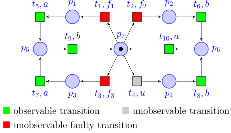
Figure 4.4: An LPN
