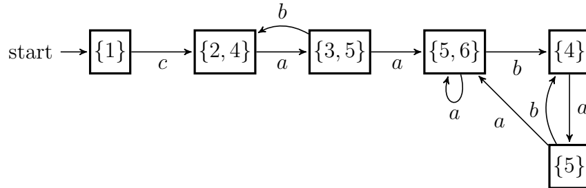
Figure 2.2: The observer of the automaton in Figure 2.1
