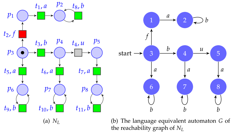
Figure 4.13: LPN N_L and its reachability graph G
