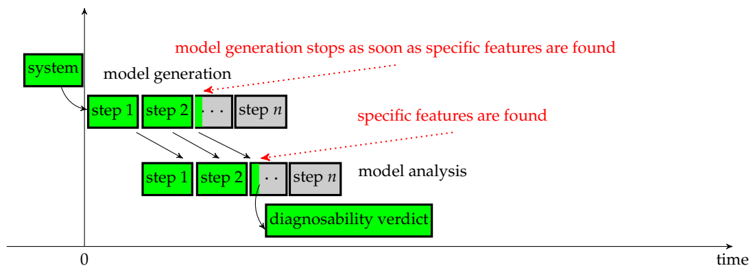
(c) Two-stage parallel and on-the-fly analysis
