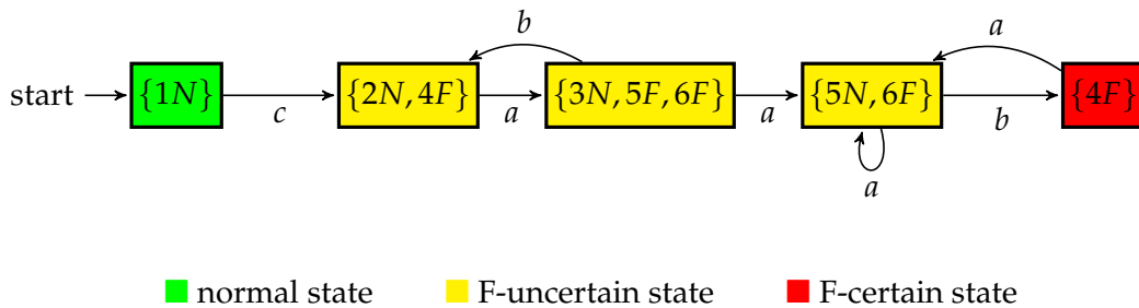
Figure 2.3: The diagnoser of the automaton in Figure 2.1
