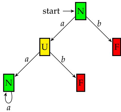
Figure 4.18: The diagnoser of N_L
