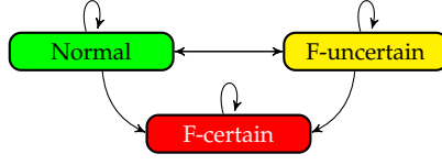
Figure 4.8: Fault propagation between FM-sets
