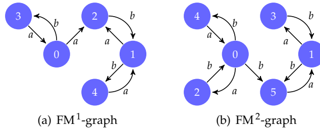
Figure 4.7: The FM-graphs of the LPN in Figure 4.3
