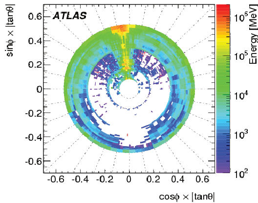
Figure 5.10: Illustration of a noise burst in the LAr calorimeter. Some cells have abnormal measured energy ( \sim 10^5 MeV) creating a hot spot in orange on this plot [87].
