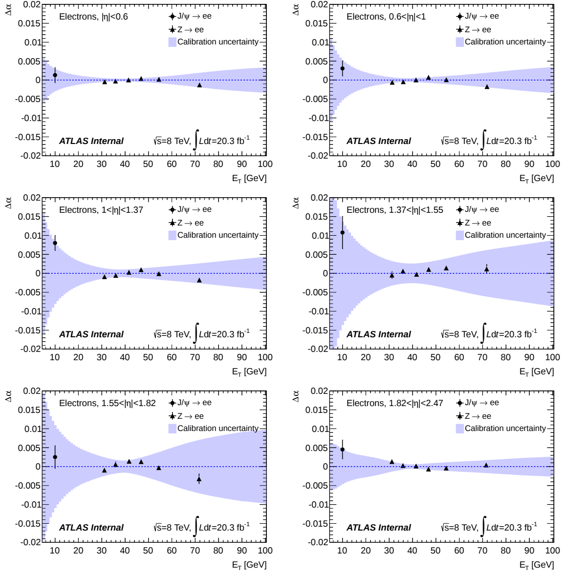
Figure 5.18: Energy scale factors \Delta\alpha for electrons. They represent the data/Monte Carlo difference after 2012 calibration [91].
