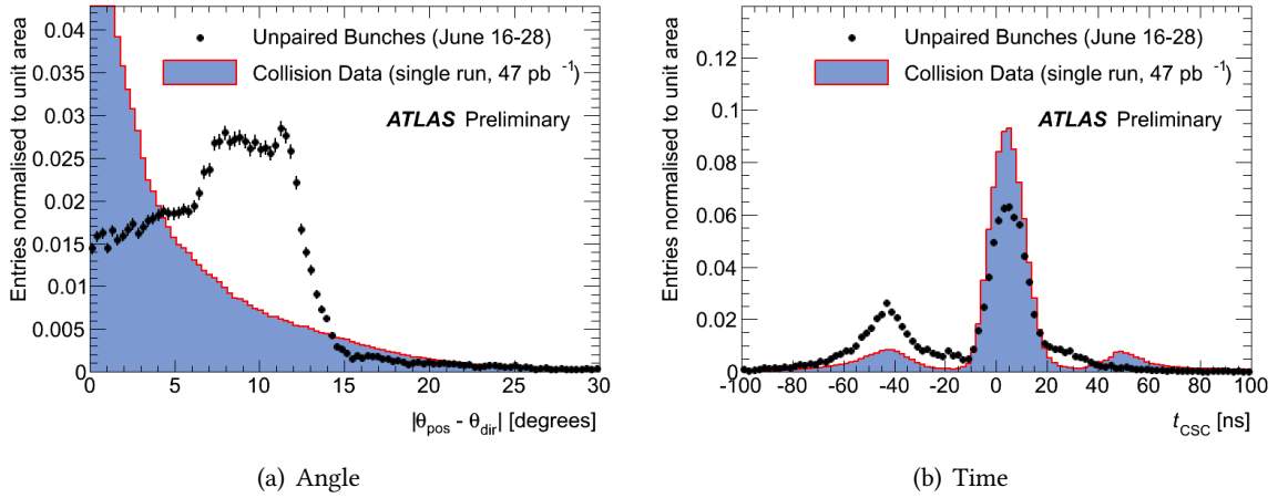
Figure 5.12: Discriminant variables used in the CSC veto technique [89]
