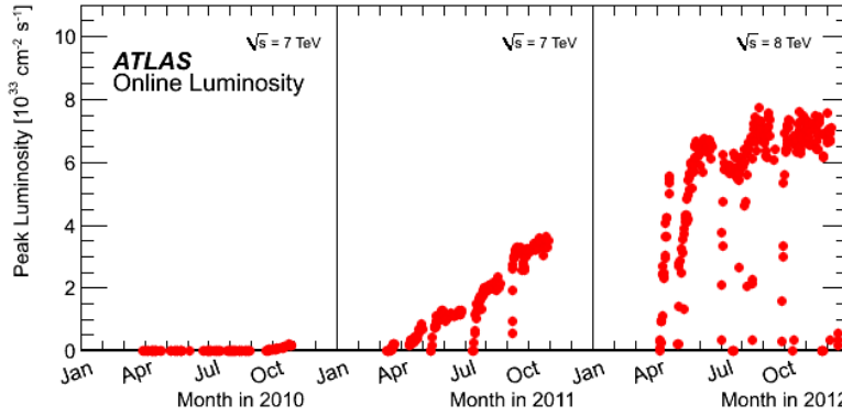
Figure 3.3: Peak luminosity as a function of time during LHC Run I (2010 to 2012) [54].
