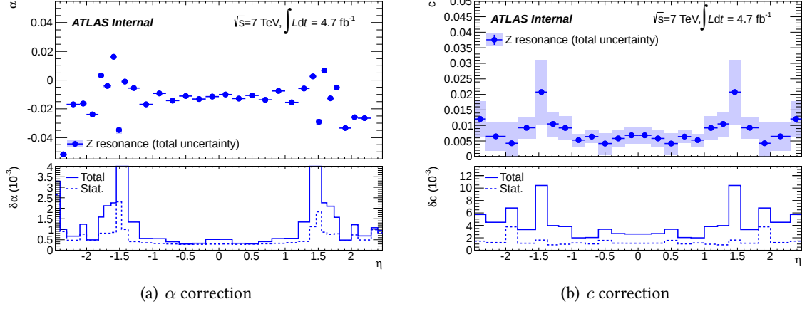
Figure 5.16: Final data to Monte Carlo corrections for 2011 data [91].
