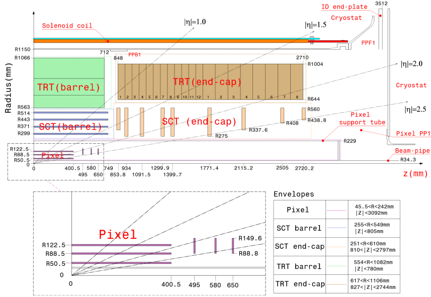
Figure 4.5: Plan view of a quadrant of the inner detector showing each of the major detector elements with their active dimensions and envelopes. The lower part shows a zoom of the pixel region [57].
