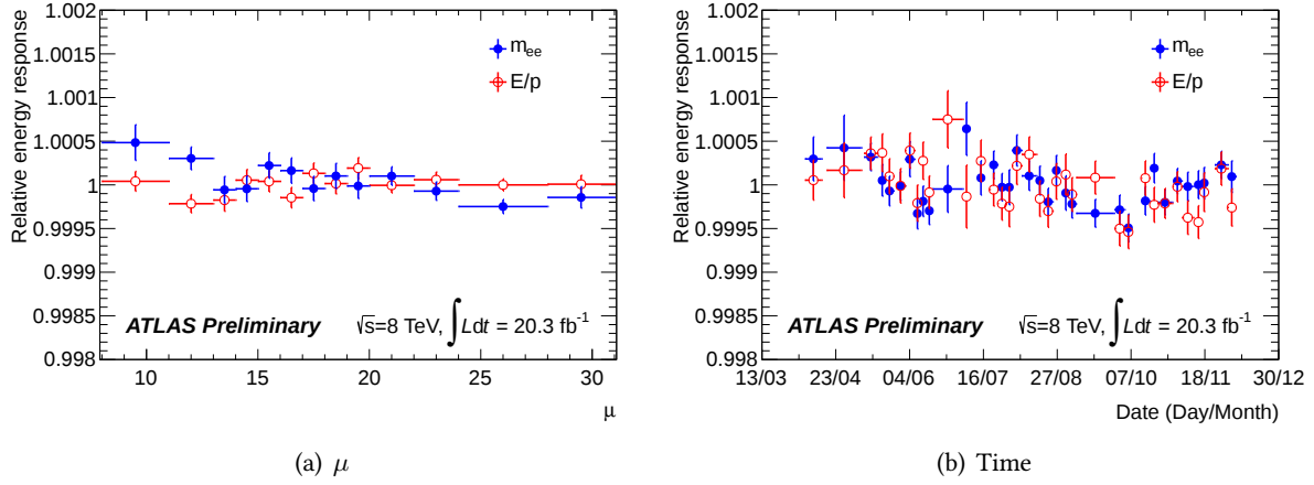
Figure 5.17: Energy response as a function of \mu and time, normalised to its average quantity for 2012 data [91].
