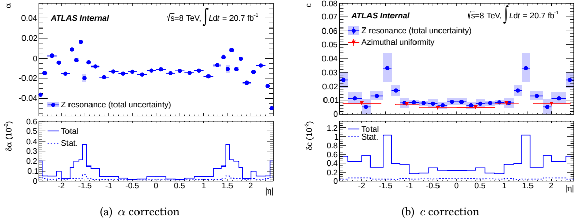
Figure 5.14: Final data to Monte Carlo corrections for 2012 data [91].
