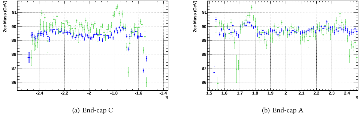
Figure 5.30: Profiles of the Z mass when the Z decays to an electron pair as a function of the leading p_T electron pseudorapidity. One point corresponds to half a cell in the second layer \Delta\eta = 0.025/2 . The blue points are from Monte Carlo while green markers represent data [100, 102].
