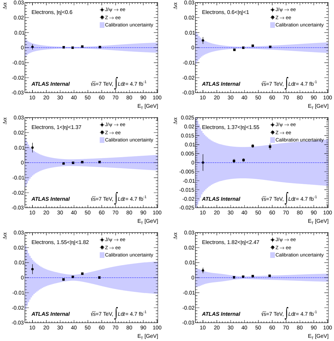
Figure 5.19: Energy scale factors \Delta\alpha for electrons. They represent the data/Monte Carlo difference after 2011 calibration [91].
