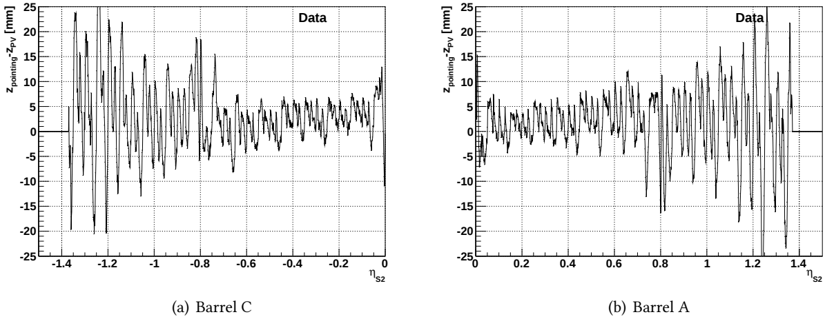
Figure 5.39: \Delta z profile as a function of the pseudorapidity in the barrel for data [100].
