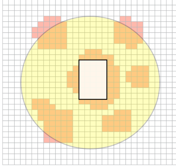
Figure 6.18: Topo-isolation principle. All cells belonging to the depicted topo-clusters are considered [117].
