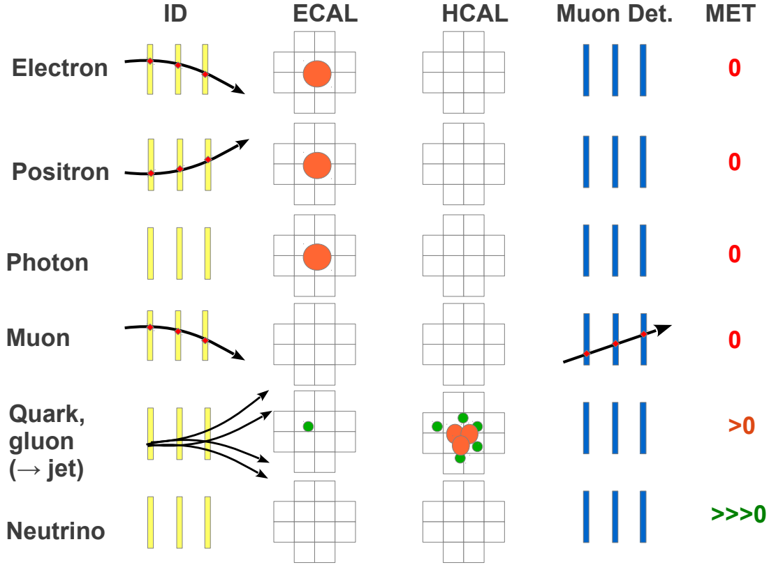
Figure 4.2: Principle of particle identification by combining the information from all the sub-detectors: Inner tracking Detector, Electromagnetic CALorimeter, Hadronic CALorimeter and Muon Detector. Track bending is shown in the (Rz) plane, i.e. the magnetic field is orthogonal to the sheet. MET stands for Missing Transverse Energy, quantity used to infer the presence of neutrinos in the event. Only the unconverted photons are represented.
