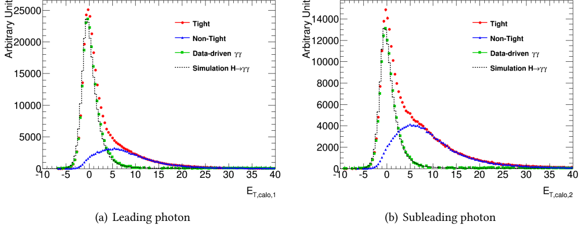
Figure 6.20: Calorimetric isolation distributions for leading and subleading photons. The red histograms show the distribution for photons passing the tight quality criteria. The blue distribution is made from non-tight photons, normalized to the tail of the distribution for tight photons, where one does not expect prompt photons. The green is obtained by subtracting the blue contribution from the red. It is compared to a Monte Carlo H \rightarrow \gamma\gamma signal sample [122].
