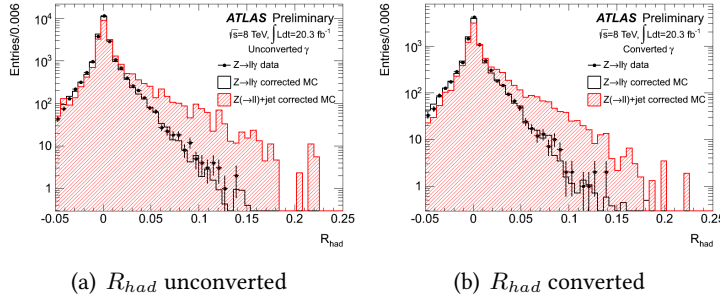
Figure 6.15: Shower shape variables using the hadronic leakage for photon reconstructed as unconverted (left) and converted (right). The Monte Carlo is corrected with Fudge Factors to merge the mean of the distributions in data and Monte Carlo [112].
