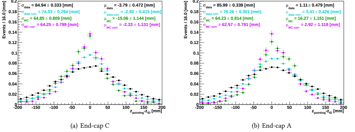
Figure 5.37: Comparison of \Delta z distributions for data and Monte Carlo before correction and after applying a specific correction to each kind of samples.
