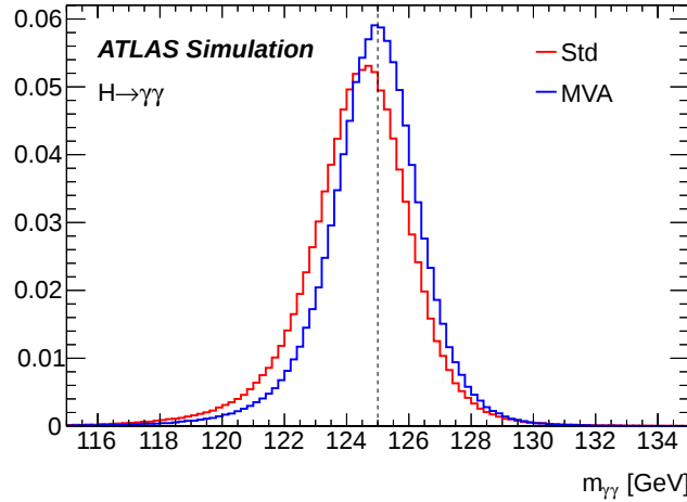
Figure 5.13: New MVA calibration compared to the cut-based approach [91].
