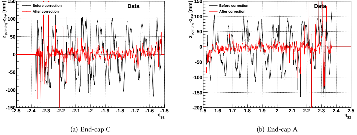
Figure 5.35: Effect of the bin-by-bin correction on the photons profiles with respect to \eta_{S2} in data [100].
