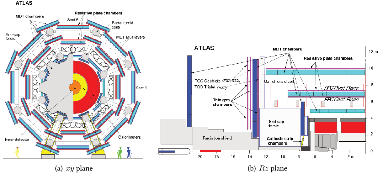
Figure 4.10: Muon spectrometer [61].
