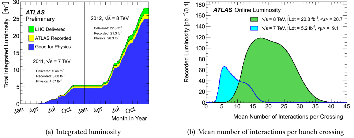
Figure 4.12: (a): luminosity delivered and recorded in ATLAS. (b): mean number of interaction per bunch crossing in 2011 and 2012 data [54].
