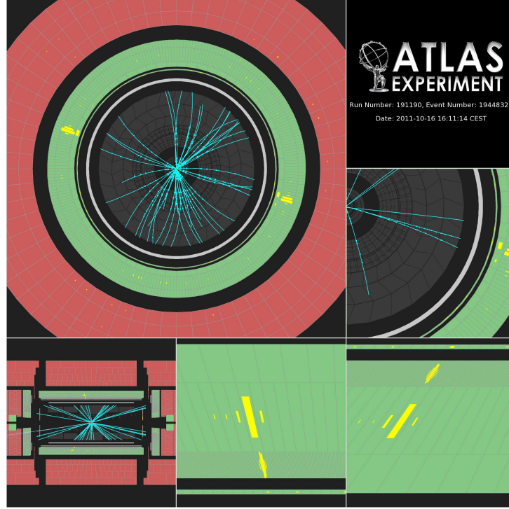
Figure 6.38: Event display of a candidate diphoton event where the leading (subleading) photon candidate is unconverted (converted). The leading photon has E_T = 66.8 GeV and \eta = -0.27 . The subleading photon has E_T = 56.9 GeV and \eta = -0.67 . The measured diphoton mass is 125.8 GeV. [170].
