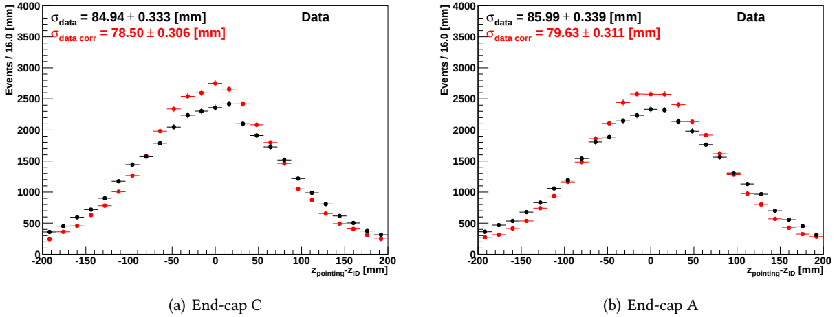
Figure 5.32: Improvement on the \Delta z distribution from the crenel correction for data [100].
