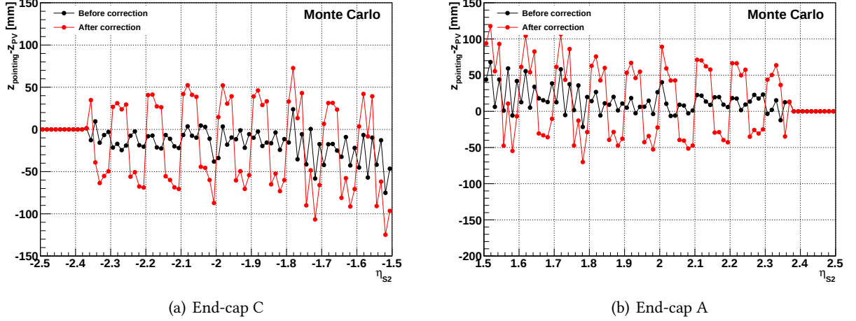
Figure 5.33: Creation of oscillations with four-cell periodicity in the Monte Carlo by applying the crenel function shown in blue in Figure 5.32 [100].
