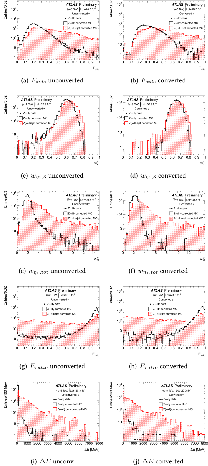
Figure 6.13: Shower shape variables using the first layer for photon reconstructed as unconverted (left) and converted (right). The Monte Carlo is corrected with Fudge Factors to merge the mean of the distributions in data and Monte Carlo [112].
