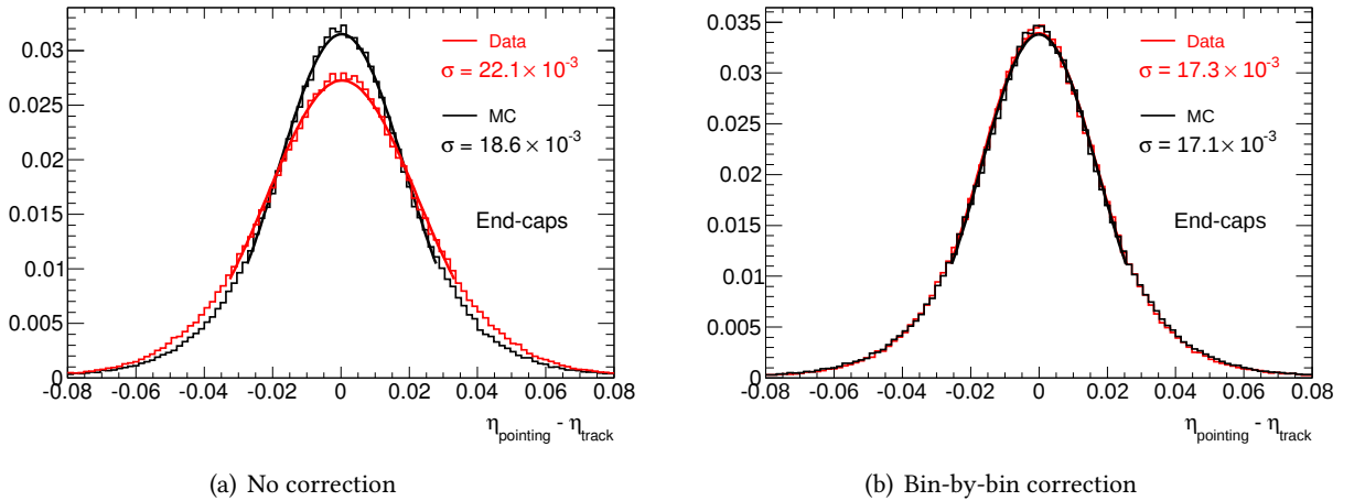
Figure 5.34: Effect of the bin-by-bin correction on \Delta\eta = \eta_{\text{pointing}} - \eta_{\text{track}} distribution for electrons in data and Monte Carlo [100].
