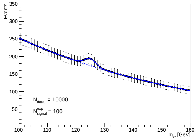
Figure 2.6: Asimov dataset corresponding to the model of Figure 2.3 with \mu_A = 1 .
