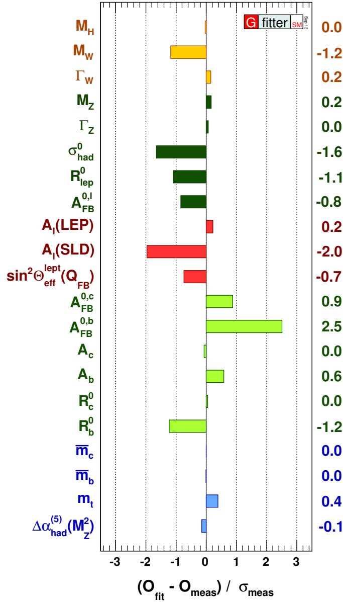
Figure 1.16: Comparison of the measured values of some Standard Model parameters with the expectations from a global fit [36].
