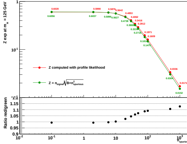
Figure 6.33: An interpretation of spurious signal: expected significance computed with a profile likelihood compared to the significance obtained with the simple spurious signal interpretation, as a function of the number of spurious signal events.
