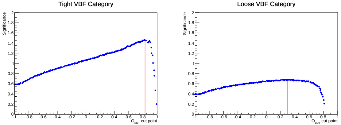
Figure 7.5: Expected VBF significance in the tight and loose VBF categories as a function of the cut on the BDT output [105].
