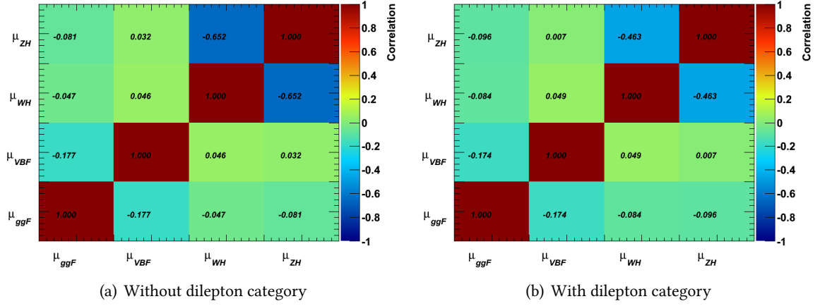
Figure 7.20: Correlation between the four parameters of interest.
