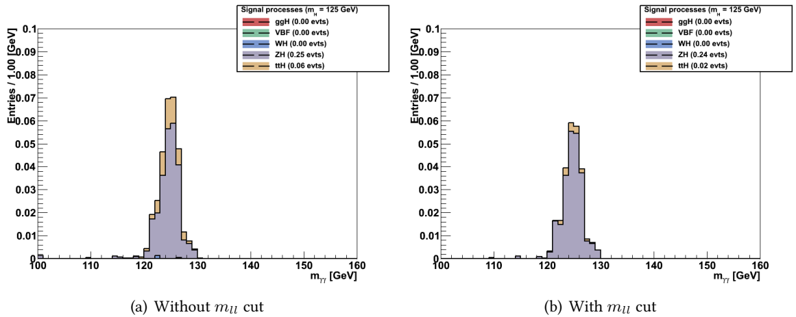
Figure 7.15: Signal composition in the dilepton category with and without cut on the dilepton invariant mass.
