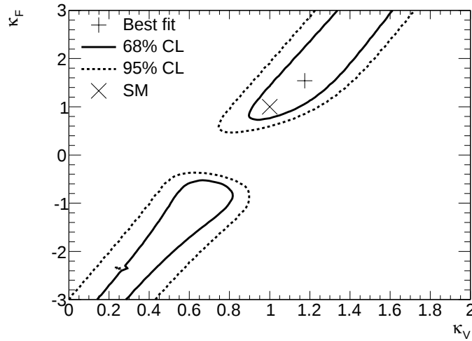
Figure 7.47: \kappa_V - \kappa_F contour from \gamma\gamma channel only [125].
