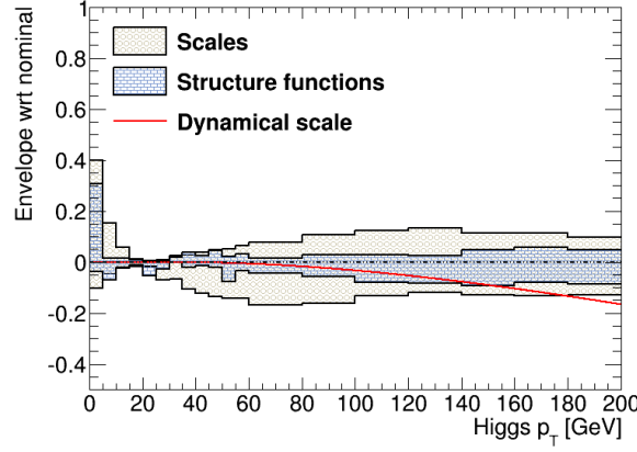
Figure 9.17: Structure functions shape uncertainties compared to the scale variations uncertainty from HRes2.0 [105].
