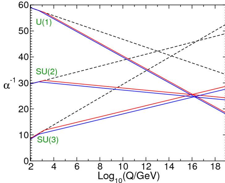
Figure 1.18: Evolution of the force strength as a function of the energy scale as predicted by the Standard Model and the MSSM [39].
