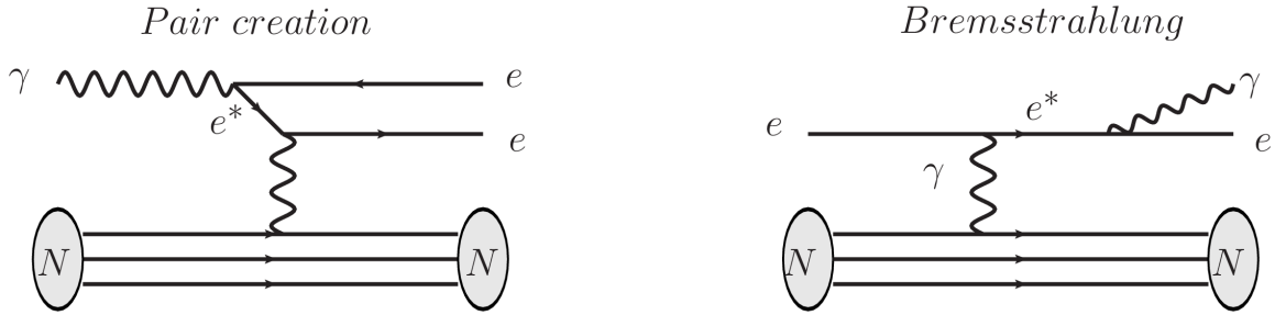
Figure 5.2: Processes responsible for a shower development in an electromagnetic calorimeter. Presence of matter, denoted as N in this picture, is mandatory to ensure energy conservation.
