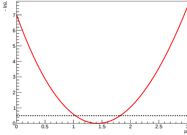
Figure 2.7: \mu likelihood scan (profile).
