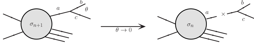
Figure 8.9: Cross-section factorization.
