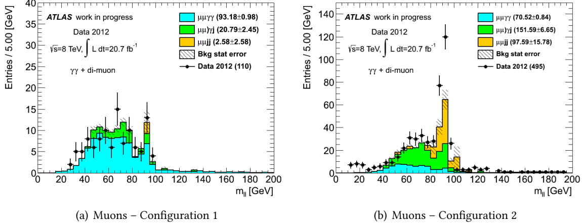
Figure 7.19: Dimuon invariant mass distribution for relaxed cuts on photons. Numbers in parenthesis show the number of events normalized to the luminosity. Data are from the \mu\mu\gamma stream. The \mu\mu\gamma\gamma background contribution should be scaled up by about 25%. The m_{ll} < 40 GeV mass range should not be considered as a filter is applied at the Monte Carlo generation stage (for Z + jets samples).
