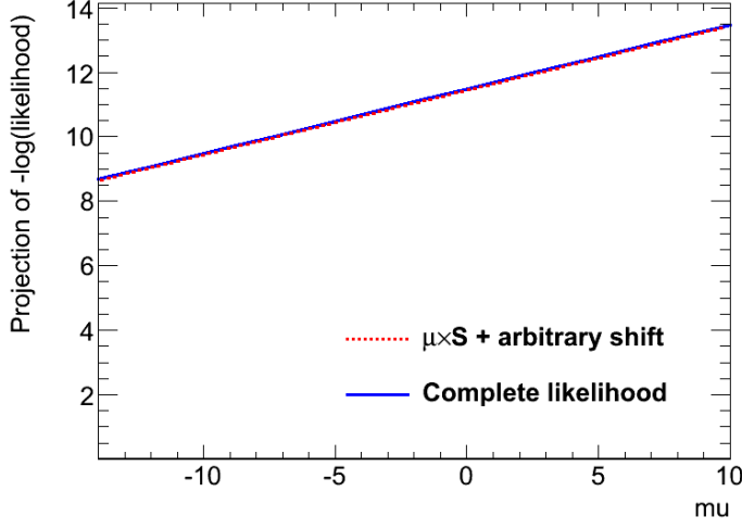
Figure 2.8: Likelihood dependence with \mu with no observed event in the signal region in the case S = 0.2 .
