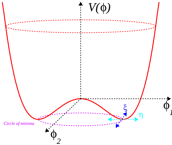
Figure 1.6: Illustration of the Higgs potential in the complex plane.
