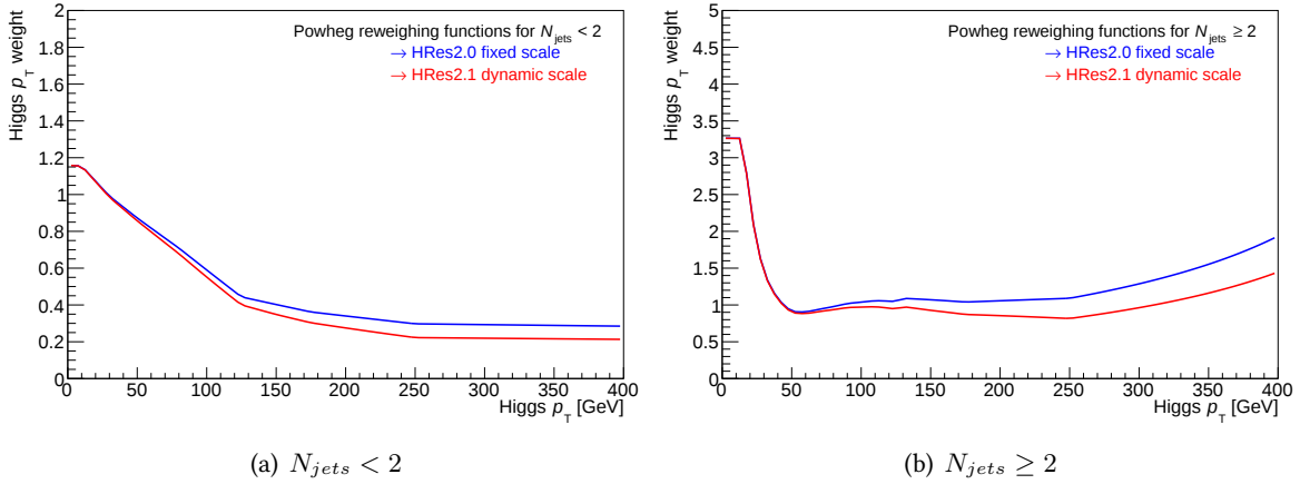
Figure 9.13: p_T weights for events with 0 or 1 jet (a) and for events with at least two truth jets (b) [105].
