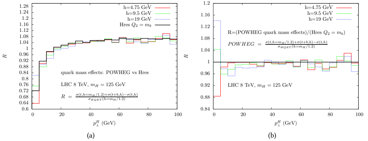
Figure 8.11: Quark mass effect in POWHEG with the linear composition of three samples. Ratio of the p_T^H spectrum coming from the combination of three POWHEG samples to the distribution from POWHEG in the HQET [240].
