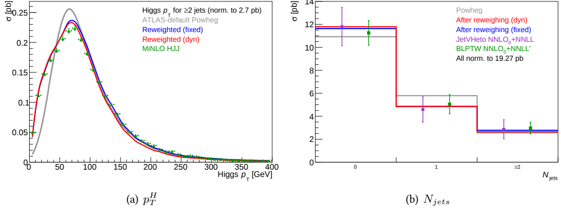
Figure 9.14: (a) p_T spectrum in events with at least two jets after reweighting, compared to MinLO . (b) jet bin cross-section before and after reweighting compared to JetVHeto [244].
