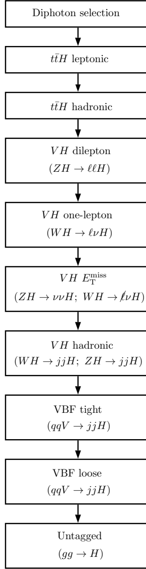
Figure 7.1: Flowchart illustrating the 12 couplings categories and the order of the selection [125].
