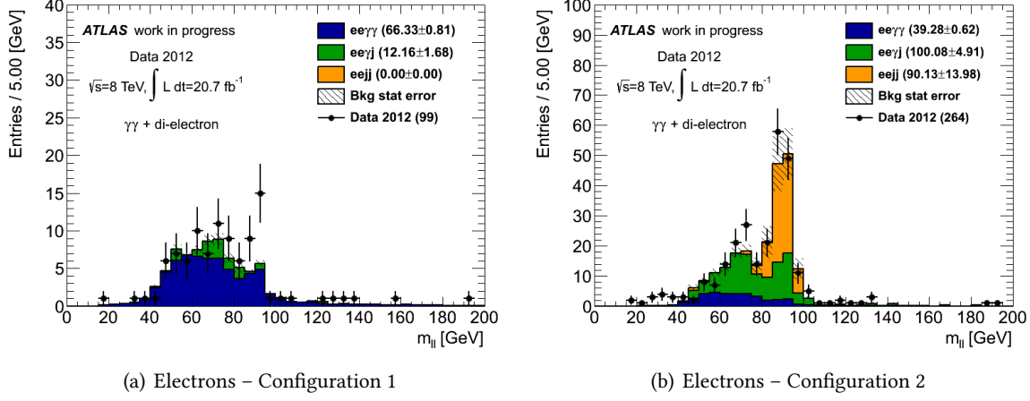
Figure 7.18: Dielectron invariant mass distribution for relaxed cuts on photons. Numbers in parenthesis show the number of events normalized to the luminosity. Data are from the ee\gamma stream. The ee\gamma\gamma background contribution should be scaled up by about 25%. The m_{ll} < 40 GeV mass range should not be considered as a filter is applied at the Monte Carlo generation stage (for Z + jets samples).
