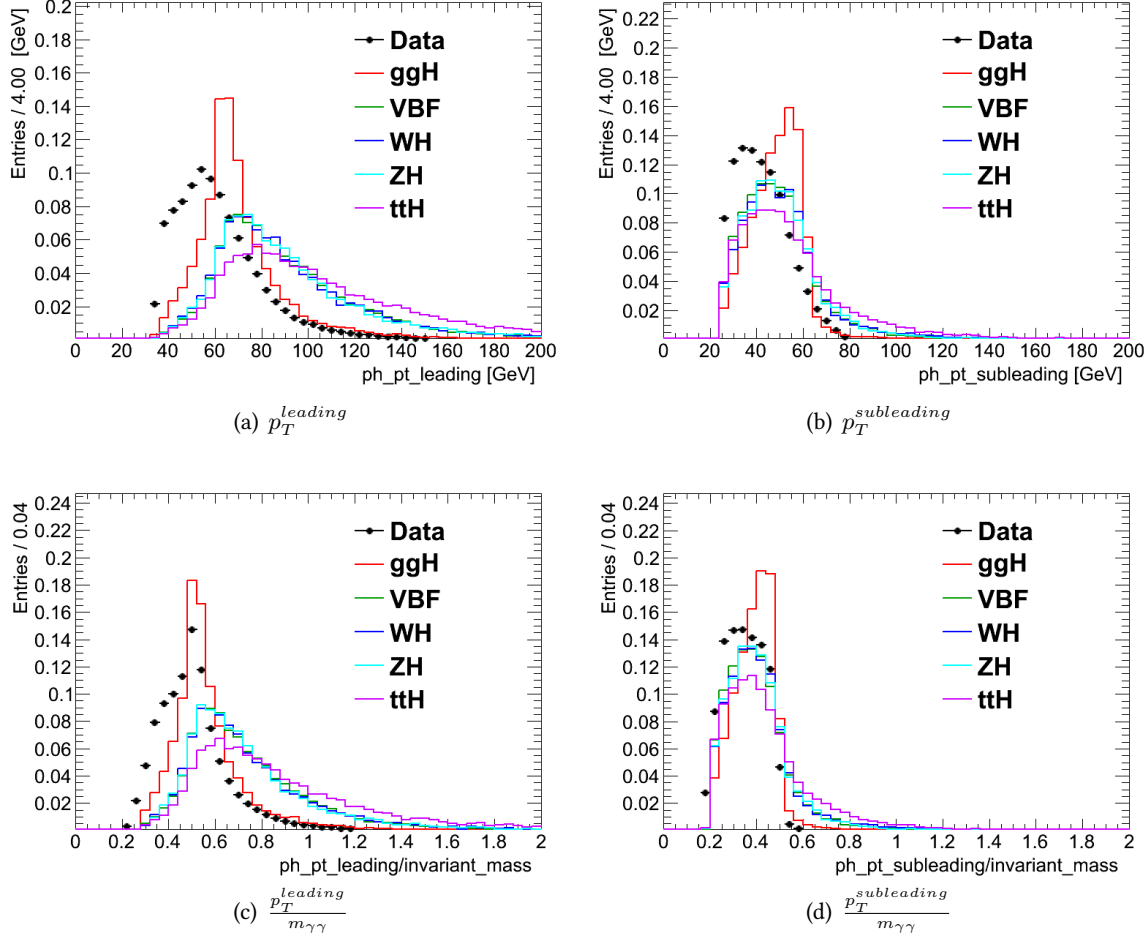
Figure 6.11: p_T and \frac{p_T}{m_{\gamma\gamma}} distributions after diphoton pair preselection for each of the production modes (Monte Carlo at m_H = 125 GeV and \sqrt{s} = 8 TeV) and for 2012 data.
