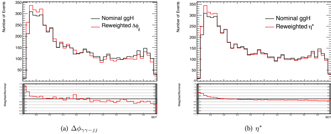
Figure 7.31: The resulting POWHEG BDT distributions with (red) and without (black) reweighting to MINLO HJJ [105].
