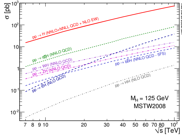
Figure 1.12: Higgs production cross section as a function of the centre of mass energy \sqrt{s} [28].
