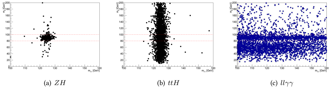
Figure 7.14: Correlation between m_{ll} and m_{\gamma\gamma} for ZH , ttH and background ee\gamma\gamma .
