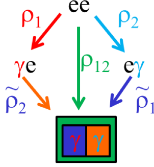
Figure 6.27: Different paths to estimate the Drell-Yan background.
