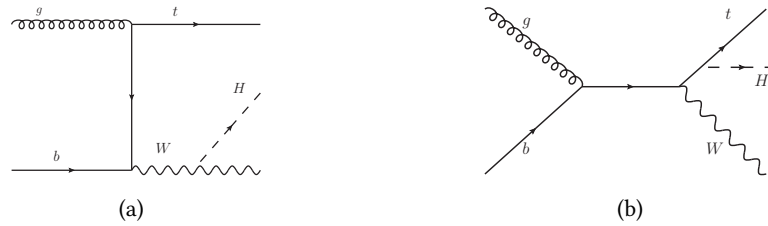
Figure 7.28: Example of diagrams contributing to the tH production in association with a W boson (see [201] for a complete description).
