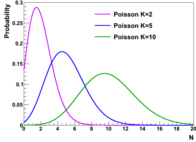
Figure 2.1: Poisson distribution (NB: P_K(0) = e^{-K} ).
