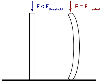
Figure 1.5: An example of spontaneously broken symmetry: rod bending.
