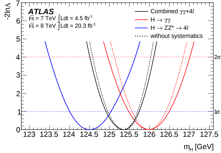
Figure 6.47: Likelihood scan of the Higgs mass hypothesis [183].
