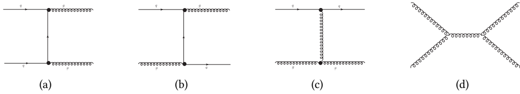
Figure 6.2: Leading order diagrams for the jj production at the LHC forming part of the reducible background to the Higgs diphoton decay channel.
