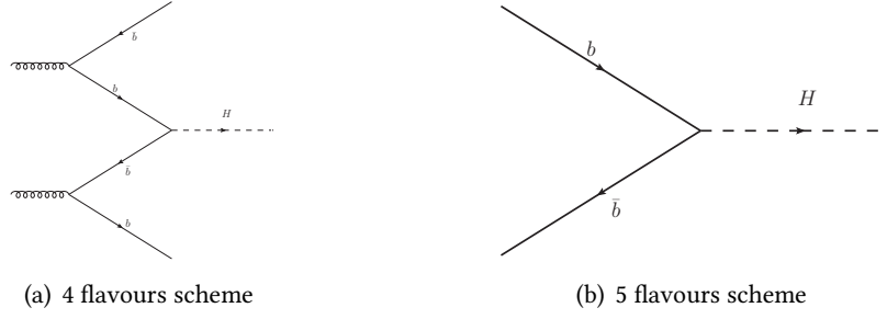
Figure 7.26: bbH process in the four flavours parton density containing only u, d, c, s and g contributions and for the five flavours scheme adding the contribution from b quark.
