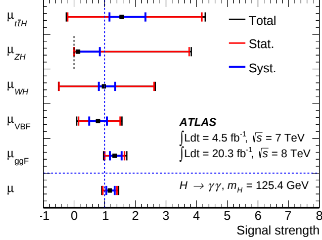
Figure 7.45: Summary of the individual signal strength fit [125].
