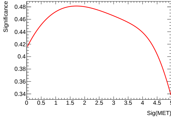
Figure 7.11: The evaluated significance dependence on the MET significance cut in the one lepton category [105].
