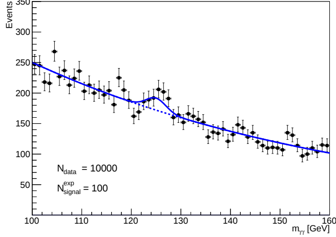
Figure 2.3: Example of model showing expected signal at m_H = 125 GeV and Monte Carlo data. The dashed line shows the background-only pdf.
