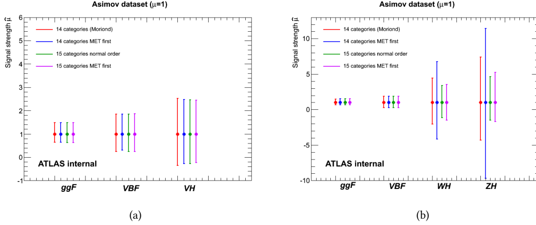
Figure 7.22: Expected improvement on the signal strengths uncertainties. Comparing the red and green lines shows the improvement between the 14 Moriond 2013 categories and the 15-category model including a dilepton category.
