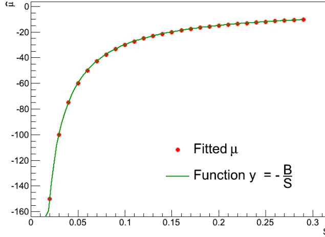
Figure 2.9: Fitted \mu , \hat{\mu} , versus the expected number of signal events S when no event is observed in the signal region.
