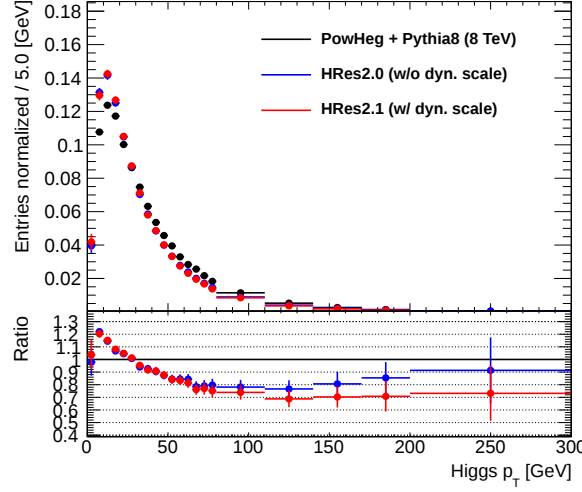
Figure 9.7: Comparison of the weights obtained with HRes2.0 without dynamical scales and HRes2.1 with dynamical scale.
