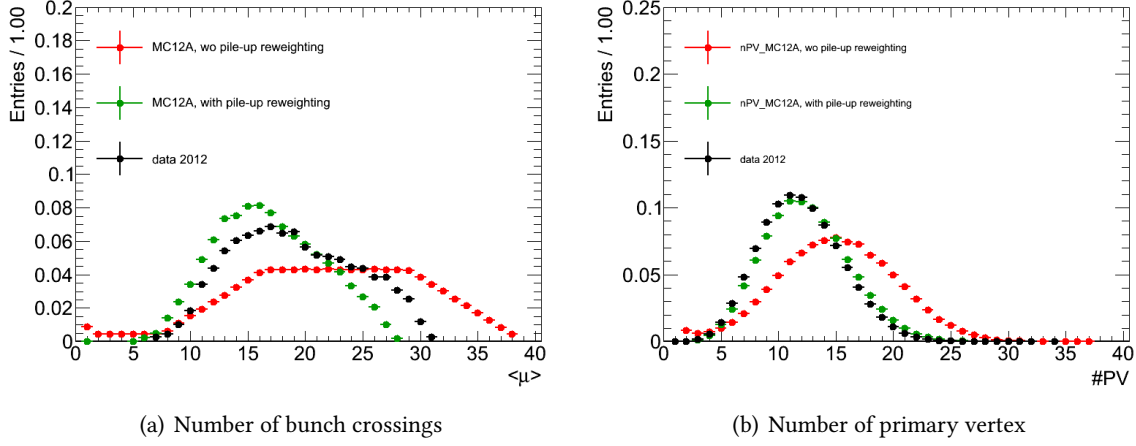
Figure 6.25: Pileup reweighting correction of the Monte Carlo (MC12A).
