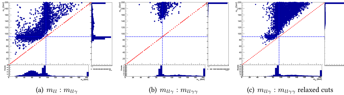
Figure 7.17: Correlation between m_{ll} , m_{ll\gamma\gamma} and m_{ll\gamma\gamma} for the ee\gamma\gamma background. m_{ll\gamma} is the closest to the Z peak among the leading and subleading photon. See text.
