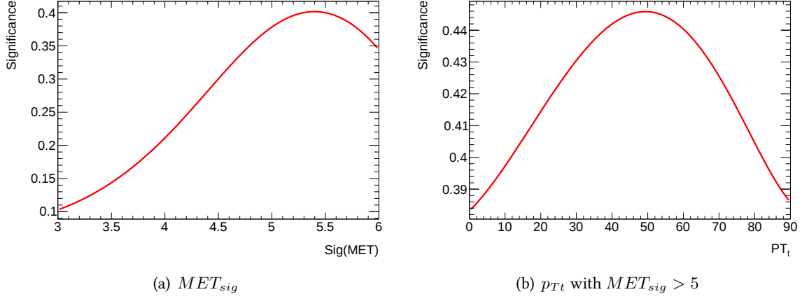
Figure 7.8: The evaluated significance dependence on the E_T^{miss} significance cut and p_{Tt} variable in the VH E_T^{miss} category [105].
