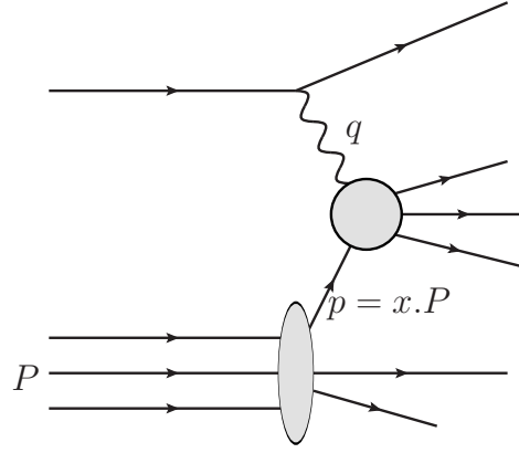
Figure 8.2: Deep inelastic scattering of an electron on a proton or neutron. P is the initial nucleon momentum.
