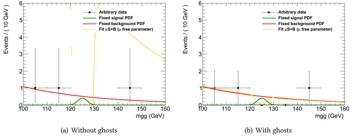
Figure 2.10: Effect of ghost events. On the left, no ghost are included and the fit is stopped when \mu = -\frac{B}{S} . On the right, ghosts are included, allowing the fit to be stopped before the pdf becomes negative.
