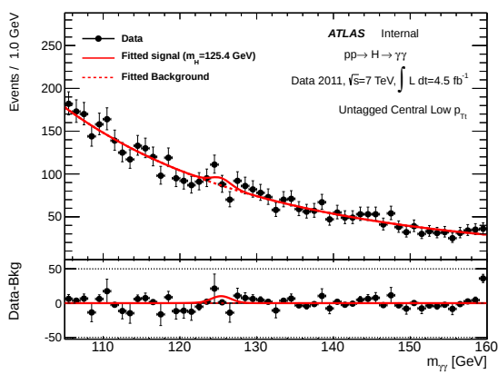
(a) Central low p_{Tt} 2011
