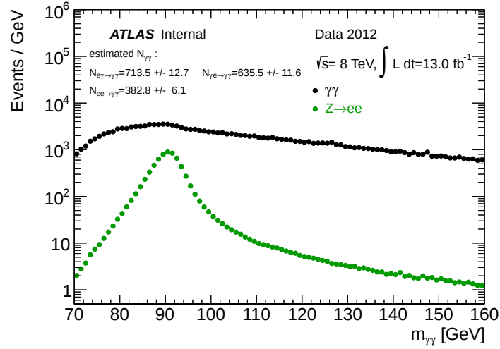
Figure 6.29: Determination of the Drell-Yan background per invariant mass bin in the region of interest for 2012 data [132].
