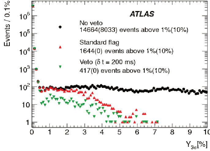
Figure 5.11: Y_{3\sigma} in the end-caps [87].
