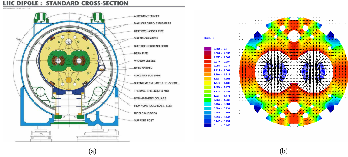
Figure 3.2: LHC dipoles (a) and the resulting magnetic field (b) [53].
