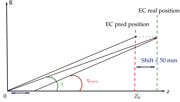
Figure 5.27: Schematic view of the expected and effective end-cap positions in the (R, z) plane. The effect on the \eta_{S2} is also shown together with the \eta'_{S2} \equiv \eta_{corr} definition [100].
