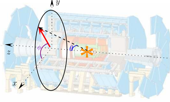
Figure 4.3: Illustration of the coordinate system in ATLAS. The orange star represents the centre of the detector taken as the origin of all axis.
