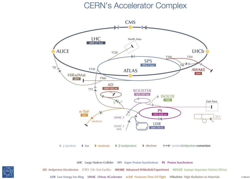
Figure 3.1: CERN accelerator complex [52].
