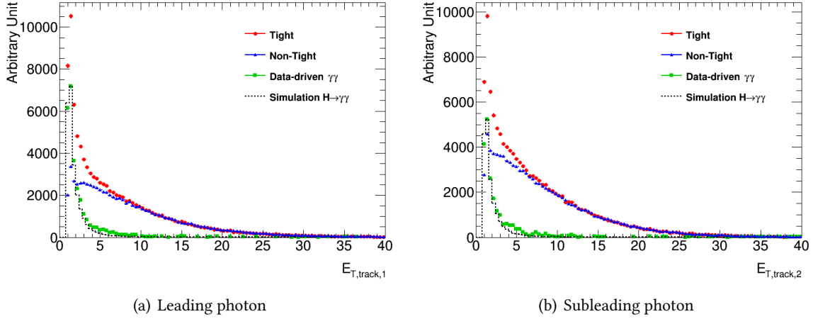
Figure 6.21: Track isolation distributions for leading and subleading photons. The red histograms show the distribution for photons passing the tight quality criteria. The blue distribution is made from non-tight photons, normalized to the tail of the distribution for tight photons, where one does not expect prompt photons. The green is obtained by subtracting the blue contribution from the red. It is compared to a Monte Carlo H \rightarrow \gamma\gamma signal sample [122].
