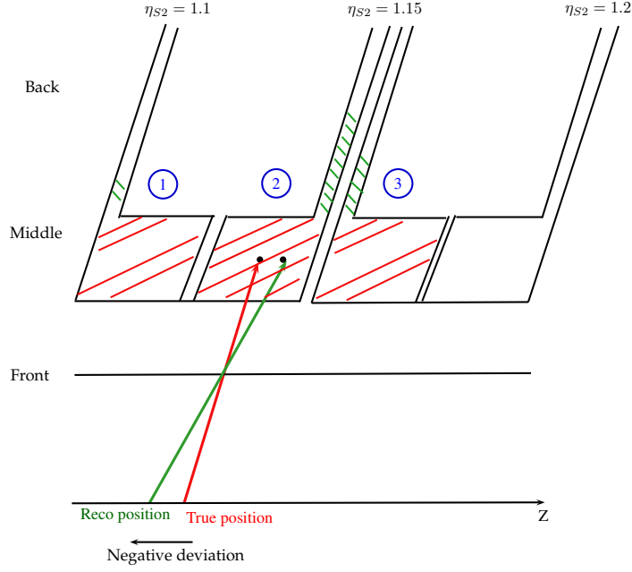
Figure 5.38: Electrode geometry in the barrel. The red line corresponds to the real photon path, that would be properly reconstructed if one considers only red energy deposit. The green line is the reconstructed path, taking into account the energy deposited in the connection strips of middle cells. The deviation is reversed if the particle hits the cell number 1 or 3, which creates a 2-cell periodic oscillation [100].
