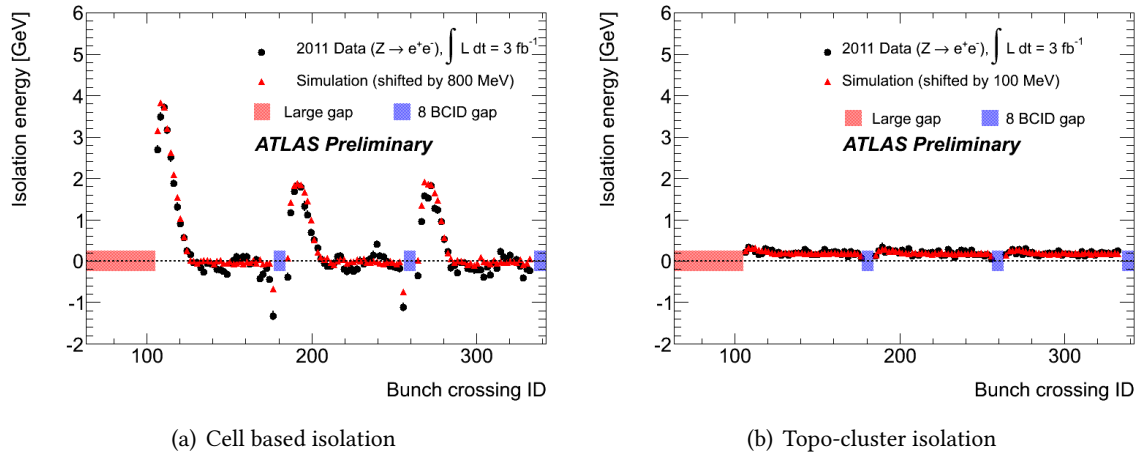
Figure 6.19: Mean of the isolation energy as a function of the out of time pile up for 2011 data. The cell-based isolation sums up all cells within \Delta R = 0.4 while the topo-cluster isolation only use cells in topo-clusters whose barycentre lies within \Delta R = 0.4 . The pile-up suppression for the topo-cluster isolation is shown to be efficient [121].
