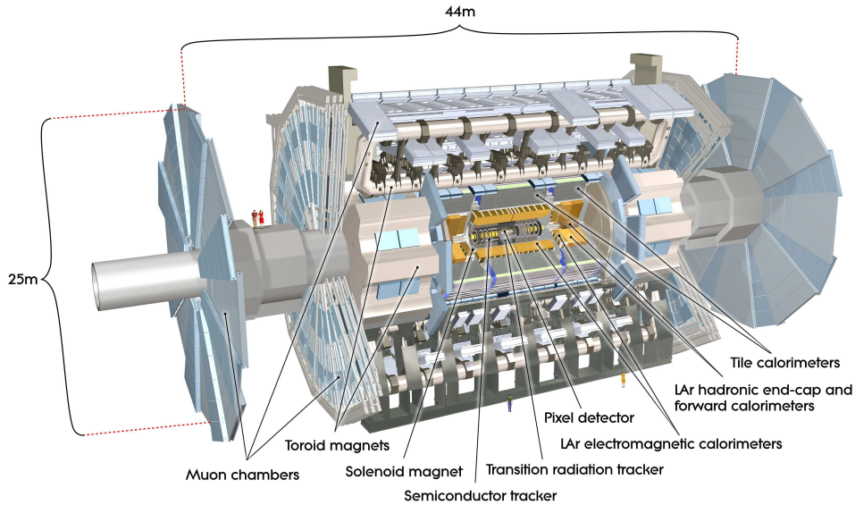
Figure 4.1: Schematic view of the ATLAS detector with its sub-systems highlighted [57].
