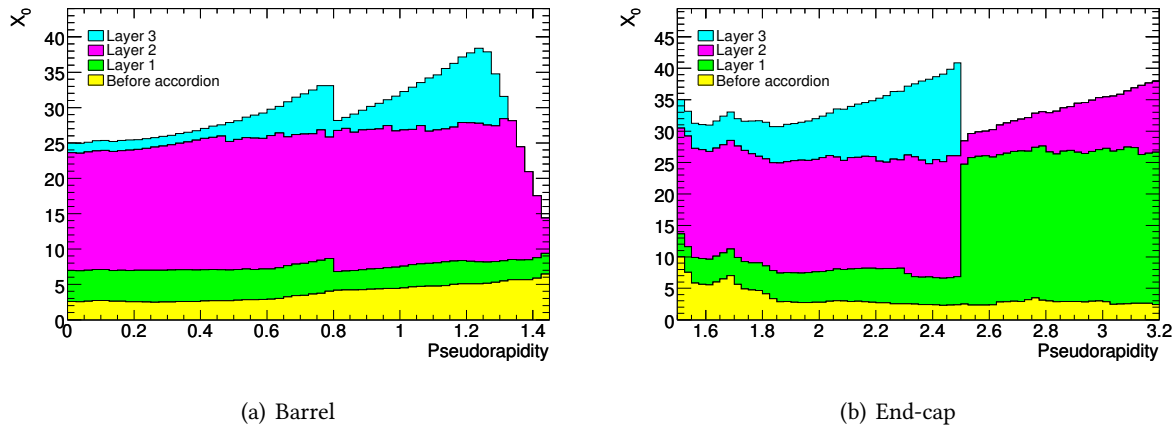
Figure 5.5: Calorimeter depth in X_0 unit. The matter before the electromagnetic calorimeter and the detail of the three LAr layers are shown in the barrel and in the end-caps [57].
