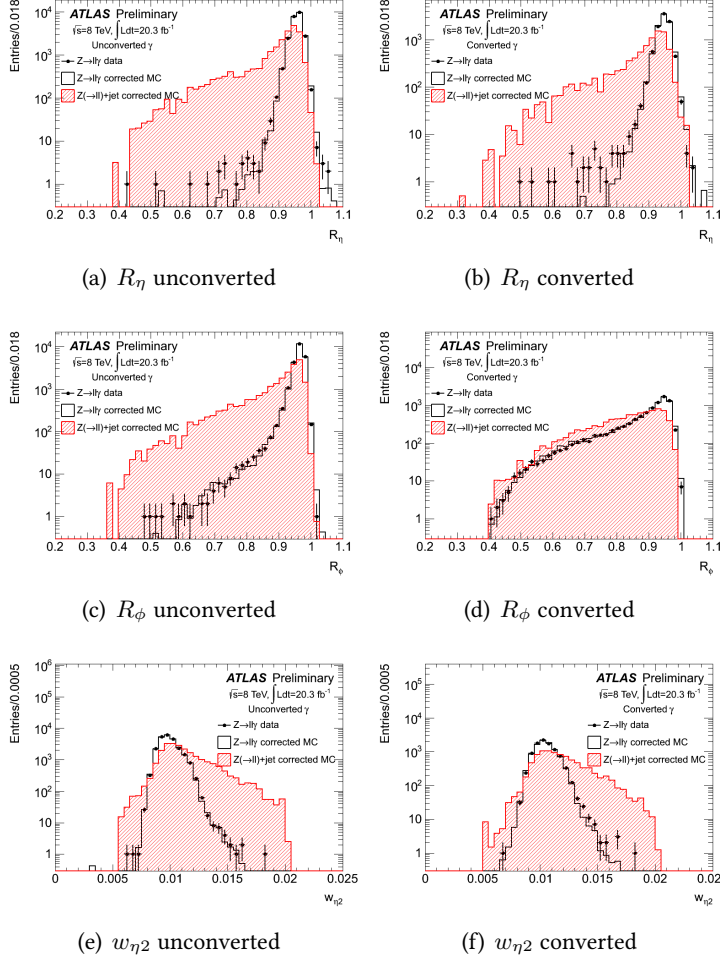
Figure 6.14: Shower shape variables using the second layer for photon reconstructed as unconverted (left) and converted (right). The Monte Carlo is corrected with Fudge Factors to merge the mean of the distributions in data and Monte Carlo [112].
