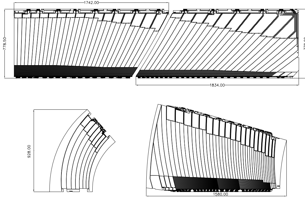
Figure 5.4: Electrode geometry. Top: in the barrel. Bottom: for the two end-cap wheels [57].
