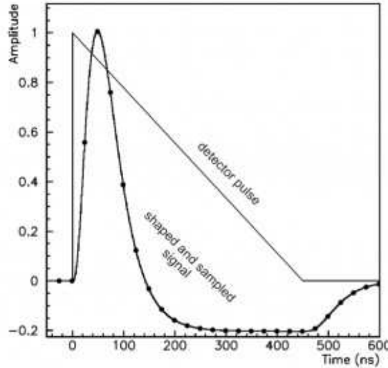
Figure 5.7: Triangular signal shape going out of the electrode and pulse bipolar shape after the FEB [57].
