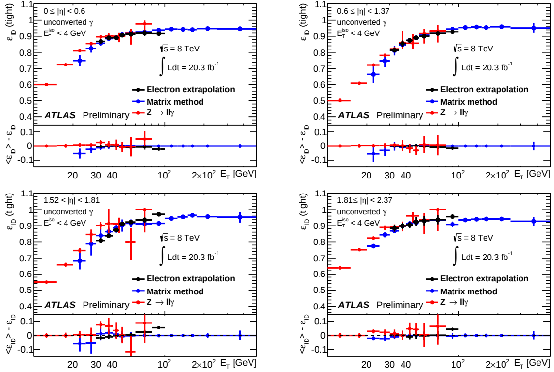
Figure 6.16: Unconverted photon identification efficiency in 2012 data from data-driven techniques as a function of the photon E_T , in four \eta regions [114].
