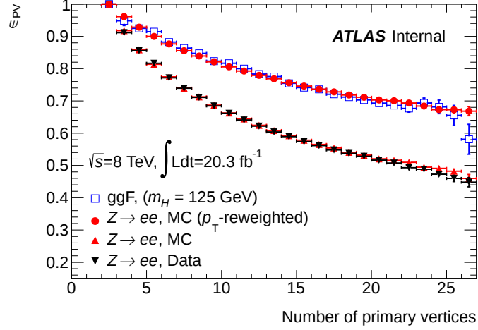
Figure 6.23: Evolution of the primary vertex reconstruction efficiency (reconstructed vertex less than 3 mm away from the vertex reconstructed from the tracking information) as a function of the number of primary vertices in 2012 data [125].
