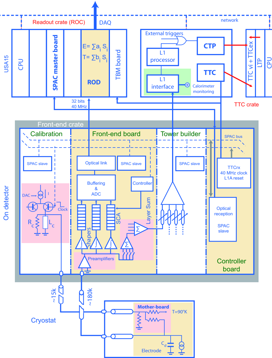
Figure 5.8: The LAr calorimeter readout electronics. The different locations are shown; the electrode in the cryostat, the front-end crate on the detector and the read-out crate in the cavern [57].
