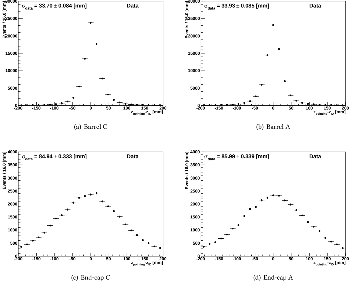
Figure 5.24: \Delta z = z_{pointing} - z_{ID} distribution in the different parts of the detector for data [100].
