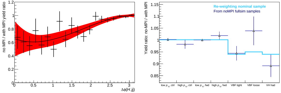
Figure 7.32: Left: Reweighting function used to propagate the the effect of the UE modelling uncertainty to the events. Right: Impact of turning the modelling of UE off, using the fullsim sample (points) and by re-weighting the nominal sample (light blue line). The reweighting gives more stable results that are consistent within statistics with the (low-stats) fullsim results [105].
