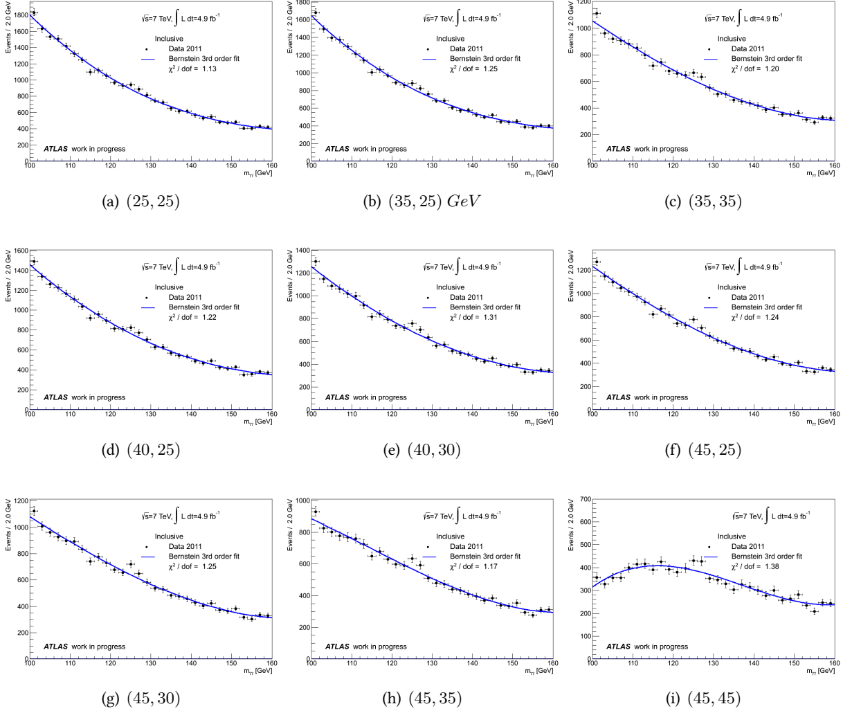
Figure 6.10: Diphoton invariant mass distribution in data for different (p_T^{\text{leading}}, p_T^{\text{subleading}}) [GeV] cuts configurations. The result of a fit of these data points with a 3 rd order Bernstein polynomial on the whole mass range is superimposed [108].
