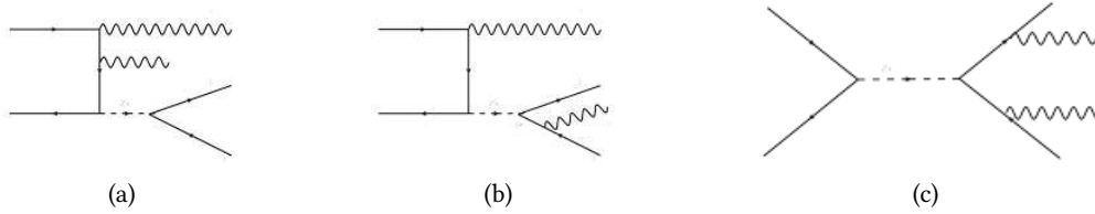
Figure 7.16: Main background contributions to the dilepton category.
