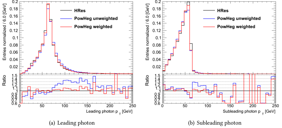
Figure 9.9: Effect of the Higgs p_T reweighting to HRes1.0 on single photon transverse momentum.
