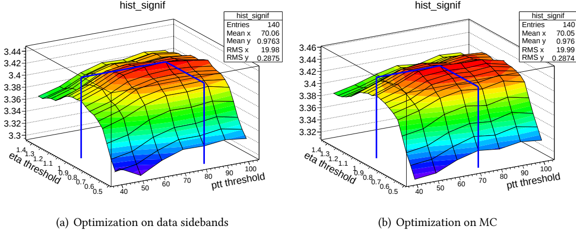
Figure 7.24: Significance as a function of the cut on p_{Tt} (10 GeV step) and \eta (0.05 step) for the p_{Tt} - \eta model [105].
