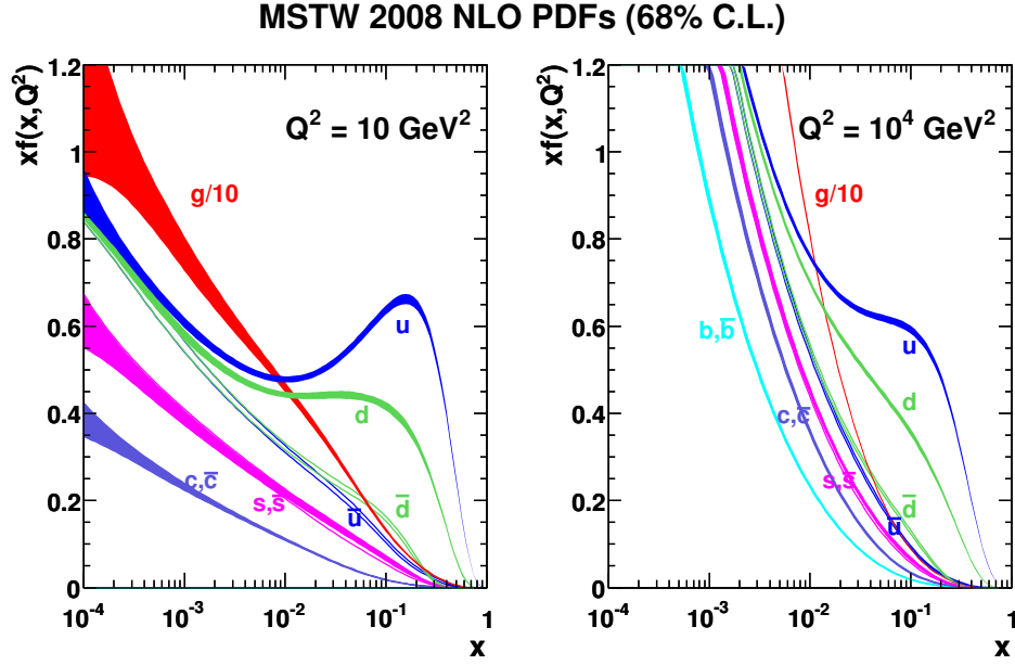
Figure 8.3: MSTW08 parton density functions as a function of x for two different energy scales Q^2 [221].
