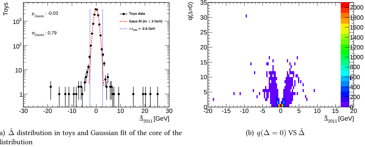
Figure 7.41: Cross-checks on the toys for the compatibility between 2011 and 2012 measured mass with the couplings categories [105].
