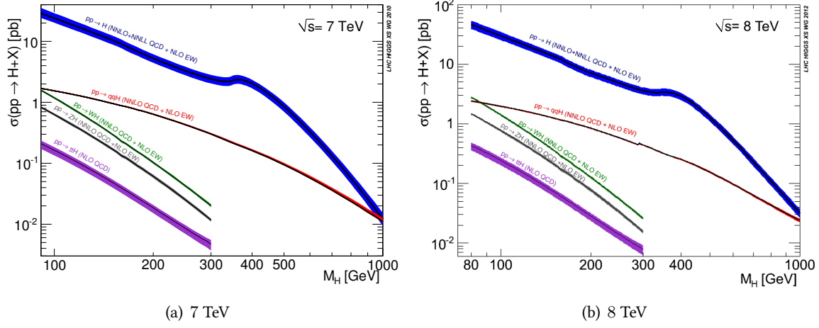
Figure 1.11: Higgs production cross section for the five main production modes of the Standard Model [27].
