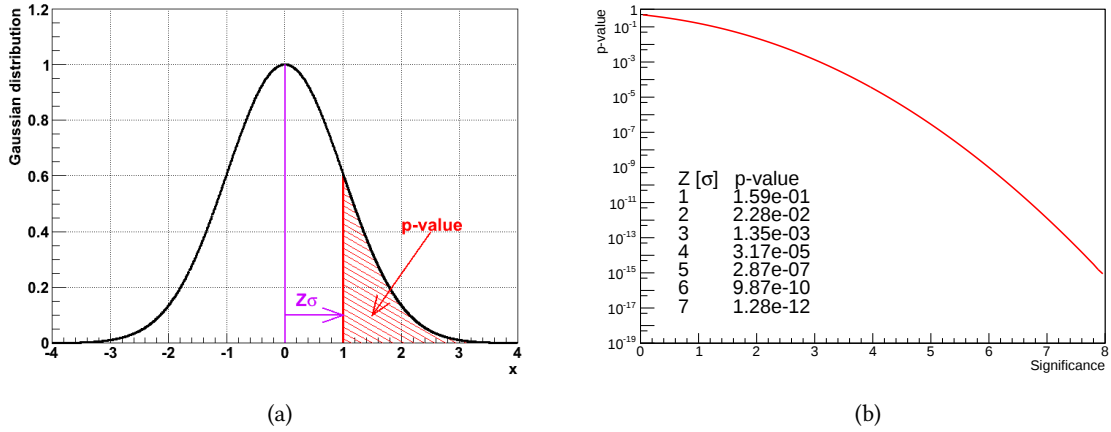
Figure 2.4: Relation between p -value and significance Z .
