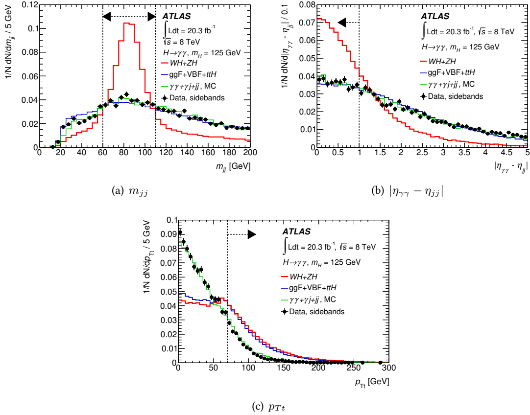
Figure 7.6: Shape comparison of inputs variables for the VH categories for different Higgs production modes and side-bands data [125].
