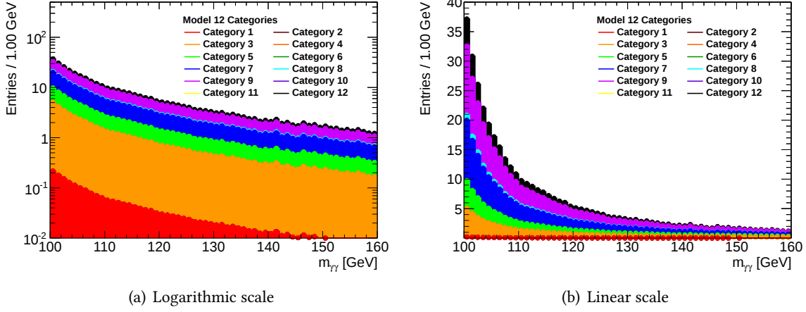
Figure 6.30: Per category decomposition of the Drell-Yan background. The shape is common to all categories, only the normalization is adapted. The estimation yields 0 for the categories not appearing on these plots.
