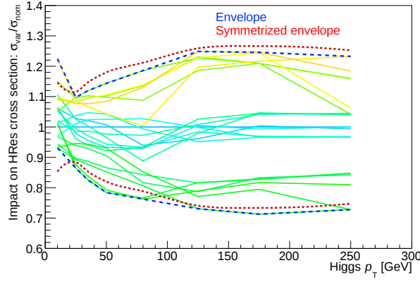
Figure 9.16: Scale variations from HRes2.0 .
