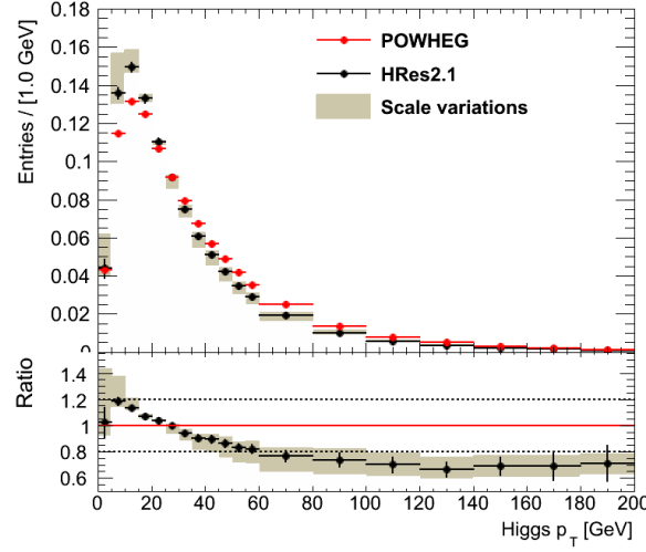
Figure 9.15: Reweighting function to HRes2.1 and shape uncertainties coming from the scale variations.
