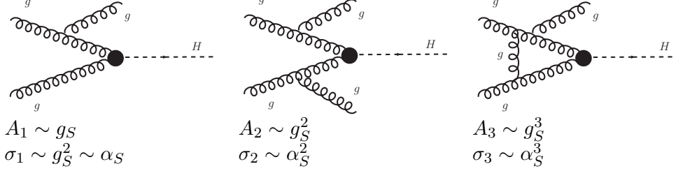
Figure 8.5: Example of higher order diagrams to the ggH process.
