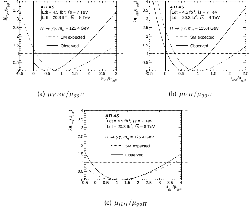
Figure 7.46: Likelihood scan for \mu_X/\mu_{ggH} [125].
