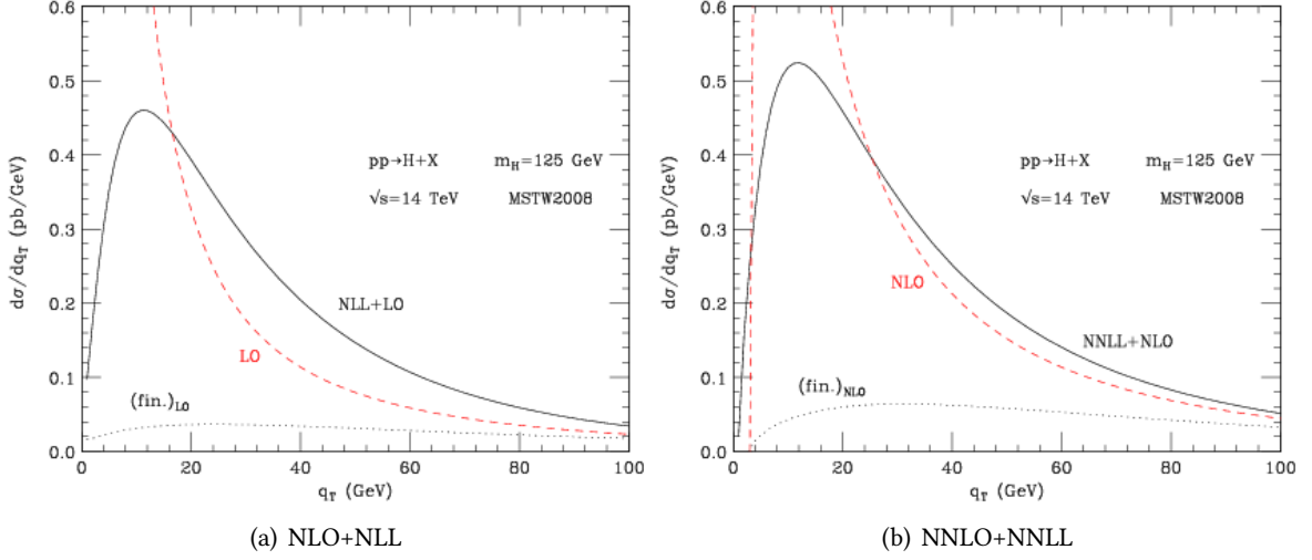
Figure 8.7: Higgs transverse momentum with resummation compared to the fixed order calculations at m_H = 125 GeV in pp collisions at \sqrt{s} = 14 TeV [146]. Note that, when considering the Higgs transverse momentum, the leading order diagram always lead to p_T^H = 0 . For the Higgs to have non zero transverse momentum, one has to go to higher order computations, where it can recoil against a jet emitted in the initial state. For this reason, the inclusive NLO cross-section is sometimes labelled LO at high Higgs p_T as is the case in these plots.
