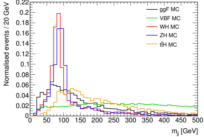
Figure 7.7: m_{jj} distribution for different Higgs production modes for events with at least two reconstructed jets [191].
