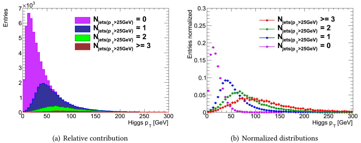
Figure 9.11: p_T distributions for different jet multiplicities.
