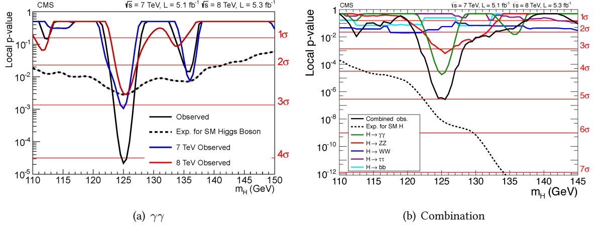
Figure 6.39: Discovery paper results from CMS [171].
