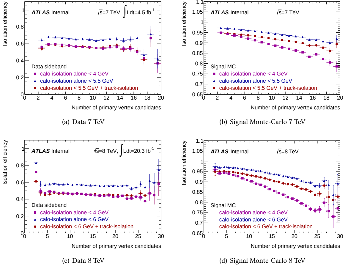
Figure 6.22: Track isolation optimization for 7 and 8 TeV analyses [105].
