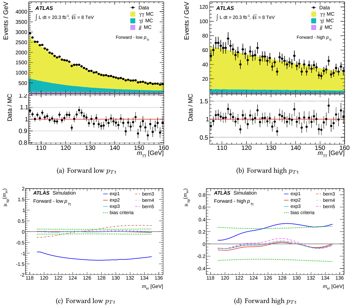
Figure 7.30: Top: smeared Monte Carlo shape and comparison to data at 8 TeV. Bottom: \mu_{SS} = \frac{N_{\text{spurious}}}{N_{\text{expected}}} [125].
