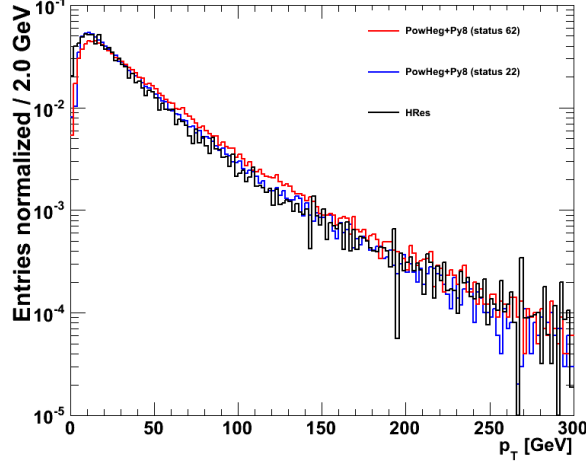
Figure 9.2: Comparison of the p_T^H spectrum coming out of POWHEG+PYTHIA8 and the HRes1.0 distribution at \sqrt{s} = 8 TeV. Status 22 refers to the POWHEG results before the action of the PYTHIA parton shower; status 62 is the code for the final particle after parton shower.
