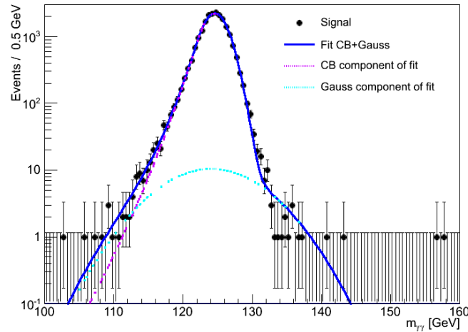
Figure 6.32: Global fit of all signal processes (inclusive). The Gauss and Crystal-Ball components are shown with dashed lines. The selection is the one from the Moriond 2013 analysis.
