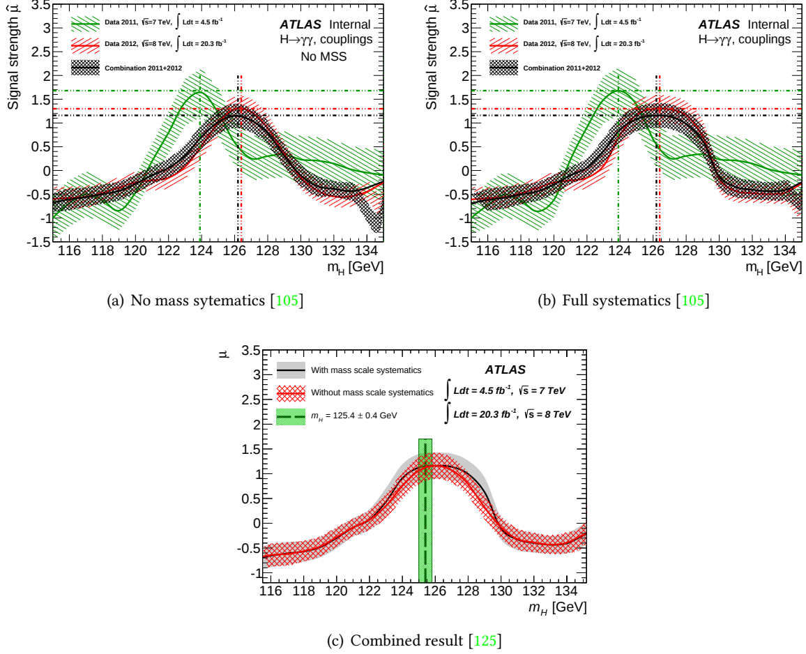
Figure 7.36: Fitted signal strength as a function of the fixed Higgs mass for data with and without the mass scale systematics.
