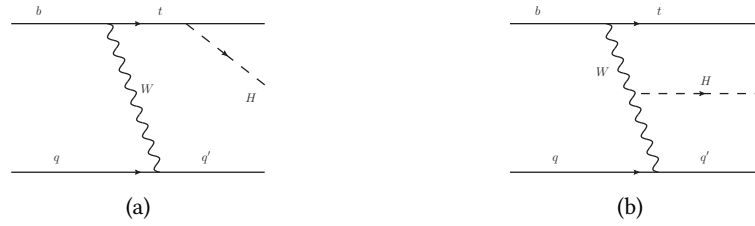
Figure 7.27: Example of diagrams for the tH production in the tHj channel (see [201] for a complete description).
