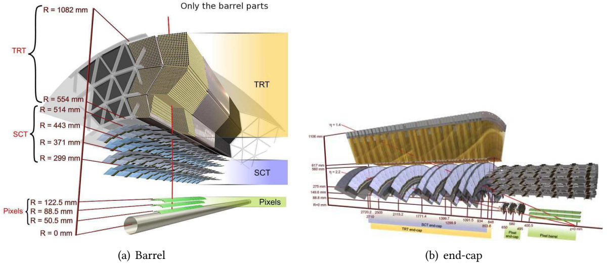
Figure 4.4: Inner detector structure. A particle track is also drawn for a 10 GeV transverse momentum at \eta = 0.3 in the barrel (a) and \eta = 1.4; 2.2 in the end-cap (b) [57].
