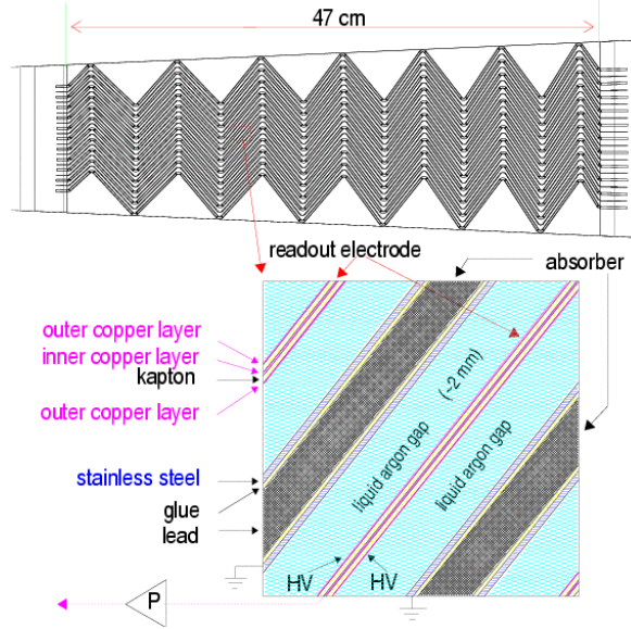
Figure 5.6: Accordion structure of the barrel. The top figure is a view of a small sector of the barrel calorimeter in a plane transverse to the LHC beams. The bottom is a zoom on the electrode structure showing the liquid argon, lead absorber and copper electrode [84].
