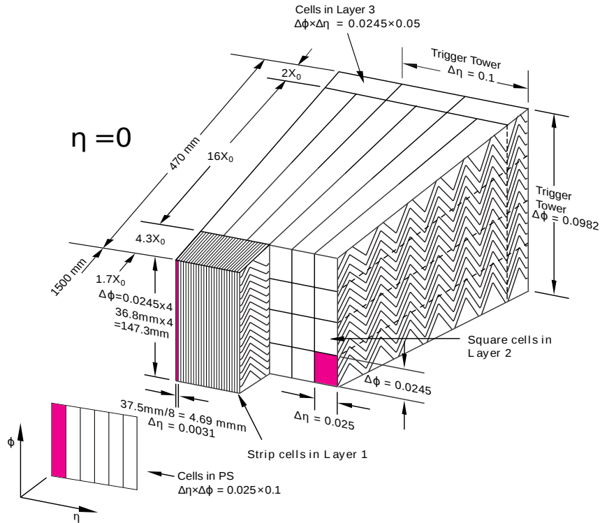
Figure 4.9: Barrel segmentation in the electromagnetic calorimeter [60].
