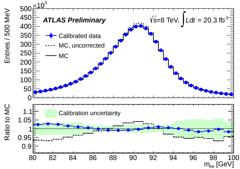
Figure 5.15: Comparison between Monte Carlo and data after offline calibration for 2012 data [91].
