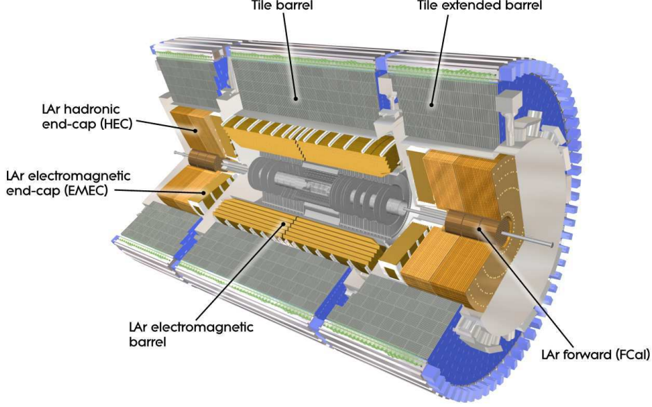
Figure 4.7: ATLAS calorimeter system including both the electromagnetic calorimeter and hadronic calorimeter. Liquid argon calorimeters are drawn in orange [57].
