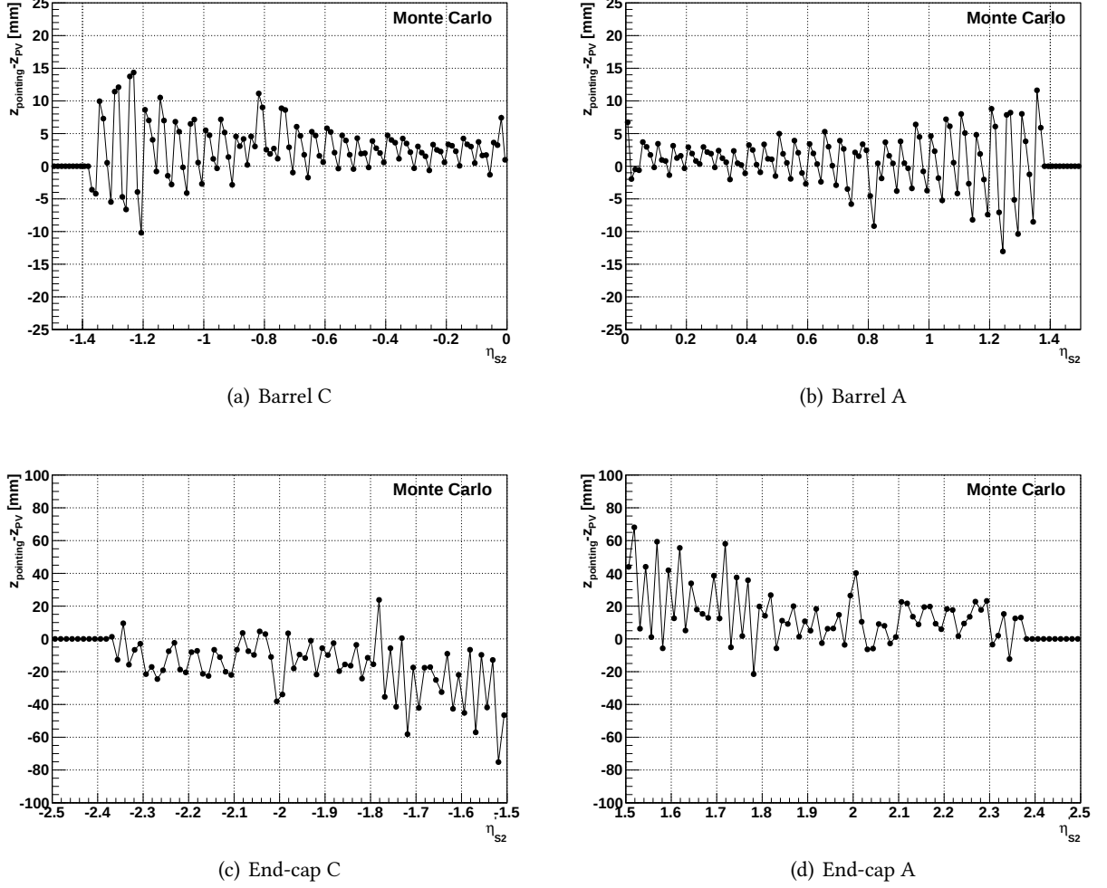
Figure 5.26: \Delta z = z_{\text{pointing}} - z_{ID} profile as a function of the second layer pseudorapidity for Monte Carlo. A point corresponds to half a cell in the second layer \Delta\eta = 0.025/2 [100].
