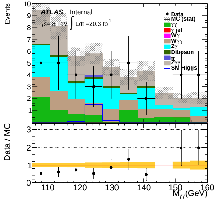
Figure 7.13: Background composition in the VH-1lepton category from Monte Carlo [105].
