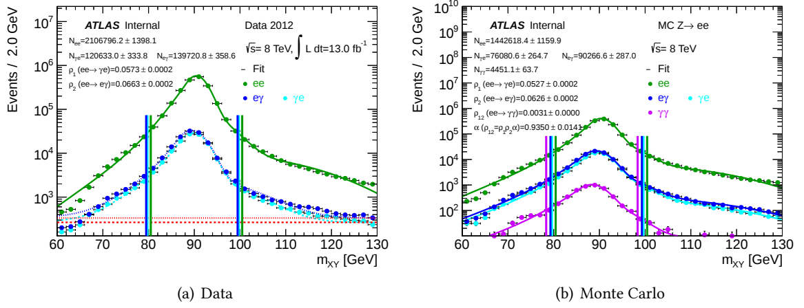
Figure 6.28: Determination of the e \rightarrow \gamma fake rate coefficients [133].
