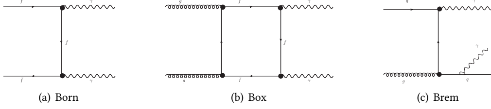
Figure 6.3: Leading order diagrams for the direct diphoton production at the LHC forming the irreducible background to the Higgs diphoton decay channel.
