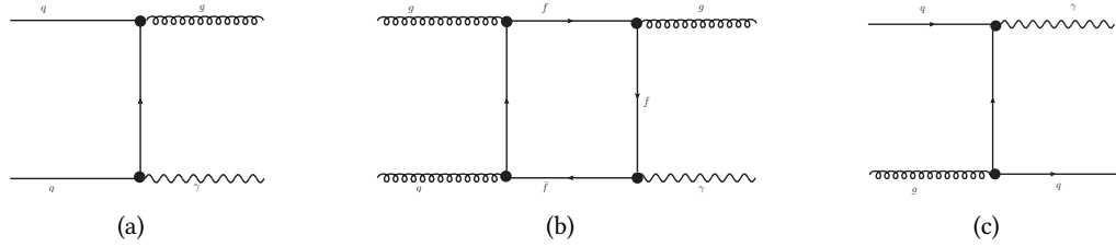
Figure 6.1: Leading order diagrams for the \gamma j production at the LHC forming part of the reducible background to the Higgs diphoton decay channel.
