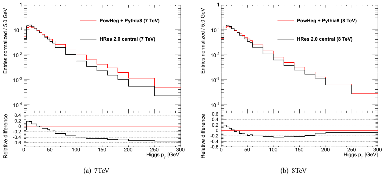
Figure 9.6: Reweighting POWHEG to HRes2.0 for the 7 and 8 TeV samples.
