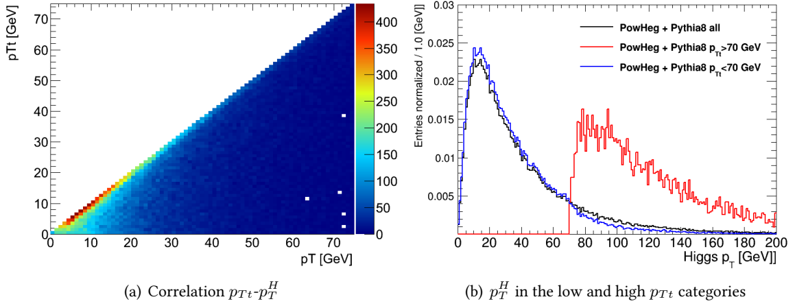
Figure 9.1: (a): correlation between p_T^H and p_{Tt} at truth level without any acceptance cuts and (b) normalized p_T^H distributions for p_{Tt} > 70 GeV and p_{Tt} < 70 GeV at truth level.
