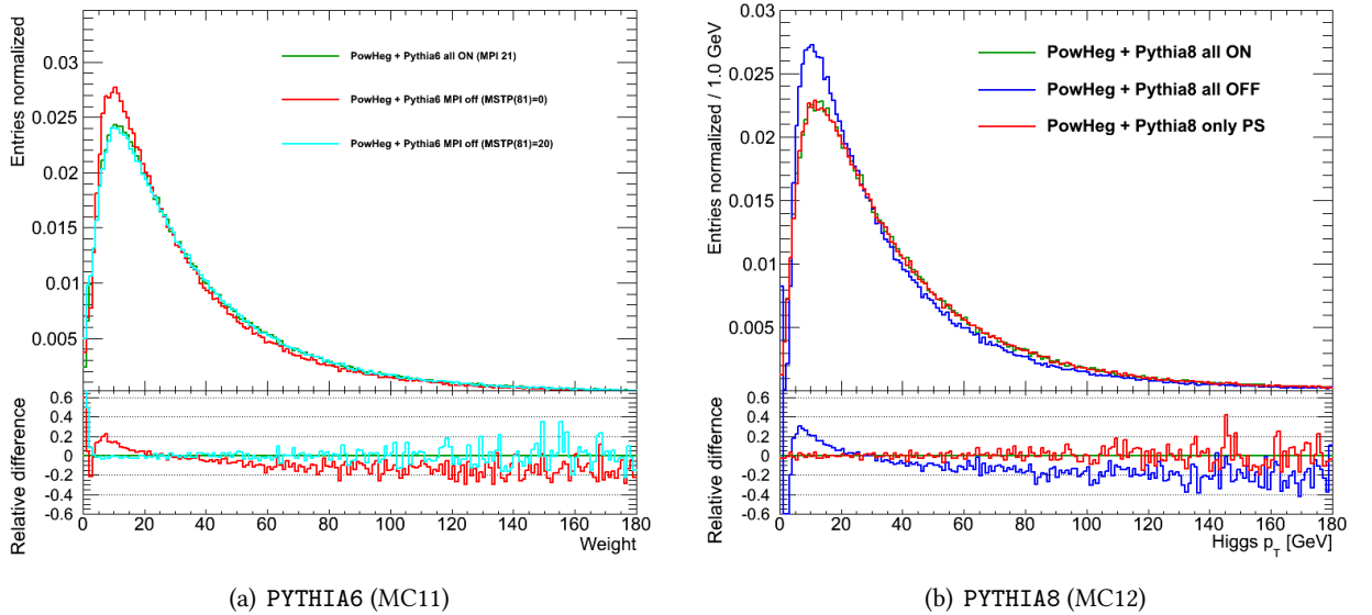
Figure 9.3: Non perturbative effect in PYTHIA shown by the cyan (left) and red (right) histograms. The green lines correspond to the default PYTHIA configuration. The blue histogram on the right plot corresponds to the case where the ISR was disabled, hence retrieving the POWHEG NLO spectrum.
