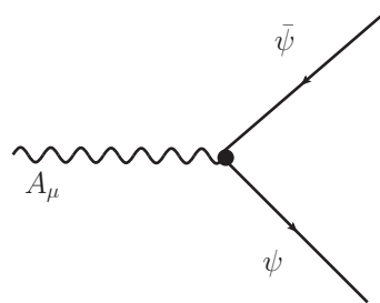
Figure 1.1: Example of interaction between two fermions via a boson.
