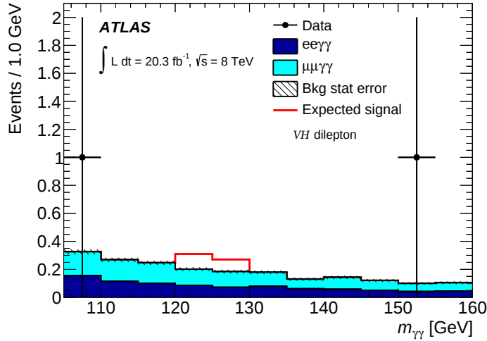
Figure 7.23: Background composition in the VH -dilepton category from Monte Carlo [125].
