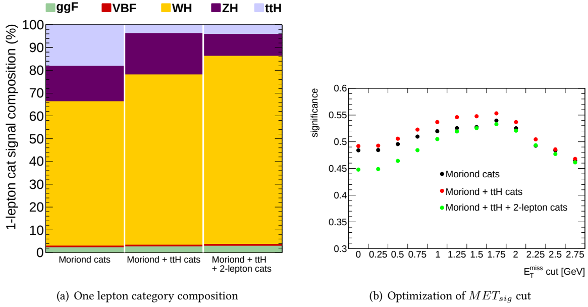
Figure 7.12: (a) Signal composition for a Higgs boson with a mass of 125 GeV in the 1-lepton category with the default Moriond 2013 selection and when adding new categories before it in the selection order. (b) Expected VH significance in the 1-lepton category when adding a cut on the MET_{sig} , for different hypotheses of categories [105].
