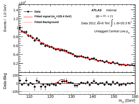
(b) Central low p_{Tt} 2012
