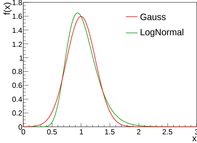
Figure 2.2: Comparison of log-normal and Gaussian shapes with \sigma = 0.25 .
