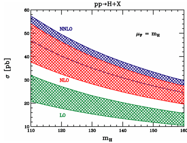
Figure 8.6: Higher order corrections effect on the ggH cross section as a function of the Higgs mass [224].
