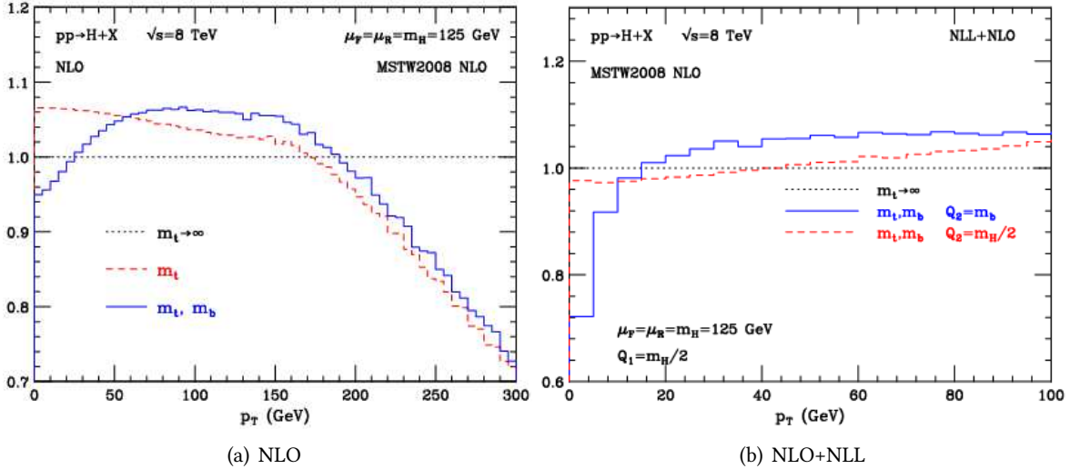
Figure 8.10: Quark mass effect in HRes2.0 at NLO and NLO+NLL. Bottom pad shows the ratio of HRes with top and bottom mass included to HRes in the HQET ( m_t \rightarrow \infty ). On the right plot, the red curve is equivalent to the POWHEG treatment [238].
