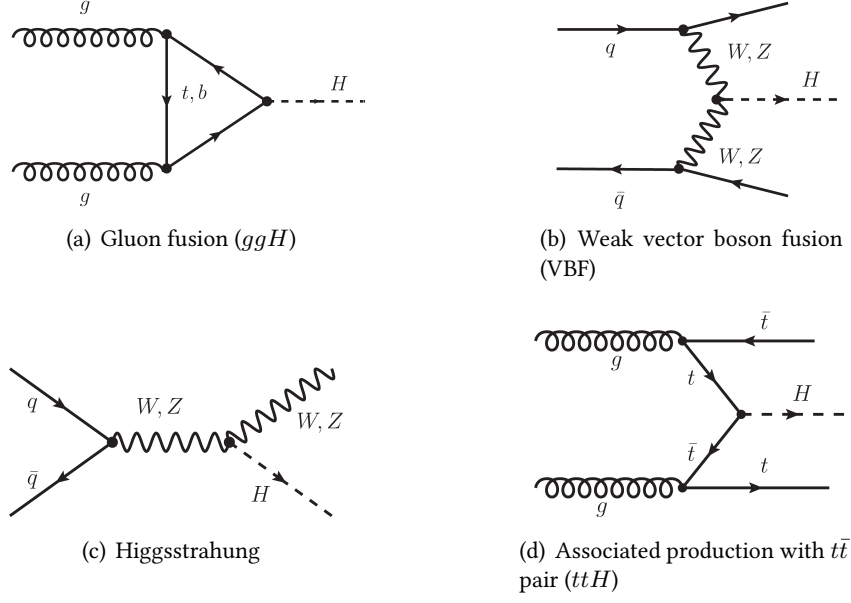
Figure 1.10: Main Higgs production modes at the LHC.
