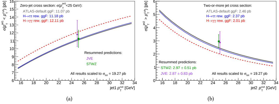
Figure 9.12: Cumulative cross-section and comparison to JetVHeto [244].
