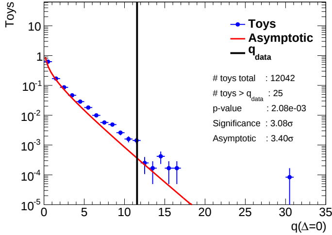
Figure 7.40: q(\Delta = 0) distribution in toys compared to asymptotic expectations [105].
