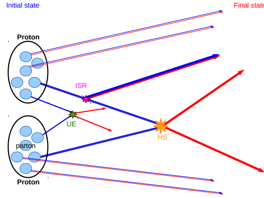
Figure 3.5: Illustration of a proton-proton collision with a Hard Scattering and one Underlying Event reaction between remaining partons.
