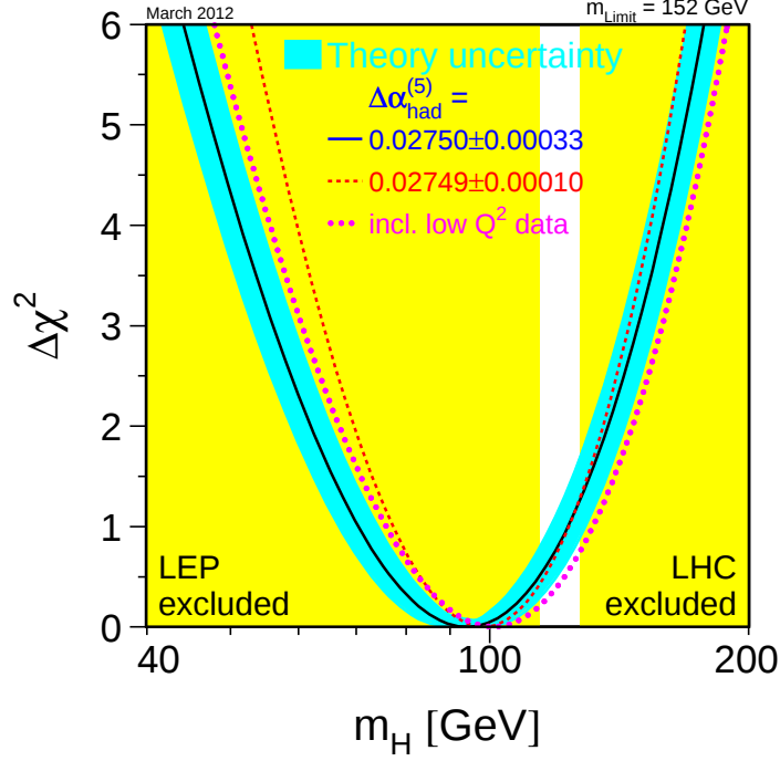
Figure 1.15: \Delta\chi^2 curve derived from precision electroweak measurements as a function of the Higgs-boson mass [32].
