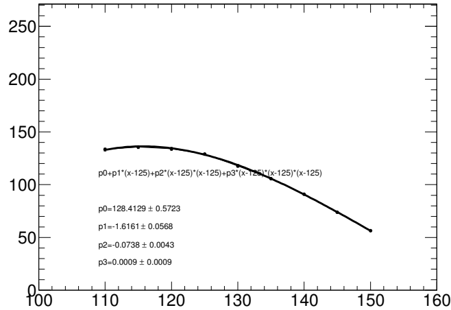
Figure 6.31: Signal yield parametrization as a function of the Higgs mass (example of ggH in category central low p_{Tt} as defined in Section 7.3.7 [105]).
