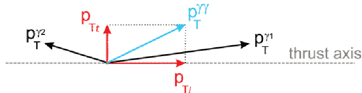
Figure 6.5: Diphoton p_{Tt} definition [106].
