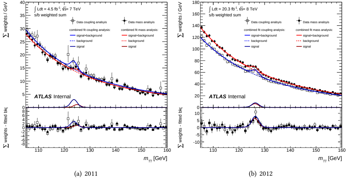
Figure 7.43: Comparison of the weighted mass spectra for the mass and couplings categories of the final Run I analysis [105].
