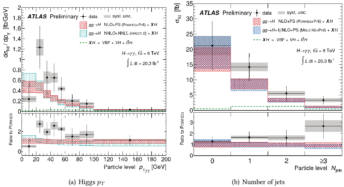
Figure 9.19: Differential cross section measurement using the diphoton decay channel. After unfolding [248].
