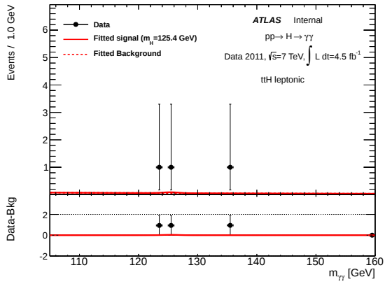
(e) ttH leptonic 2011
