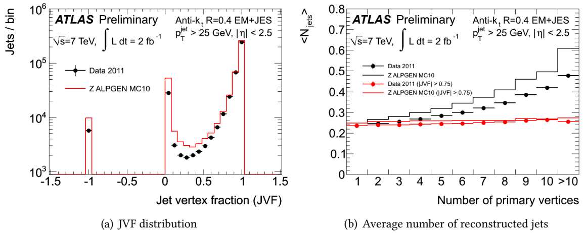
Figure 4.15: Jet Vertex Fraction performance: (a) JVF distribution for data and Monte Carlo. JVF is set to -1 when no track is associated to the jet. JVF = 0 corresponds to jets with no track associated to the selected primary vertex in the event. (b) illustrates the impact of a |JVF| cut at 0.75 on the reconstructed number of jets with respect to the number of primary vertices, representative of the pileup [73].
