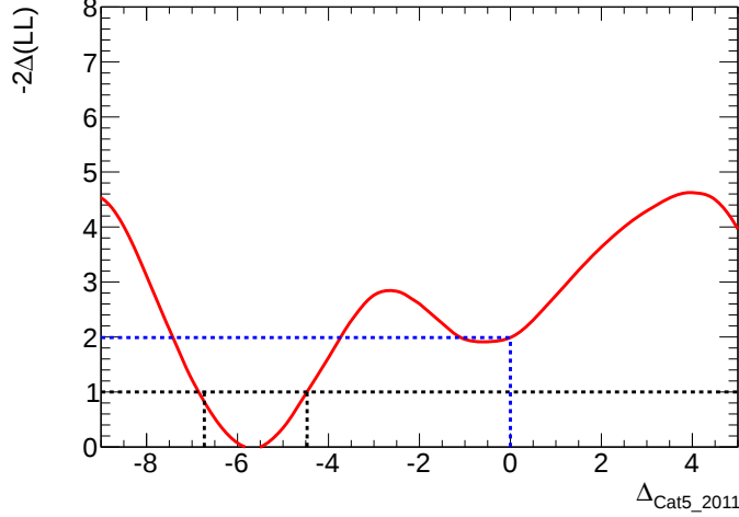
Figure 7.38: Likelihood scan for the VBF-loose category in 2011 (Cat5) [105].
