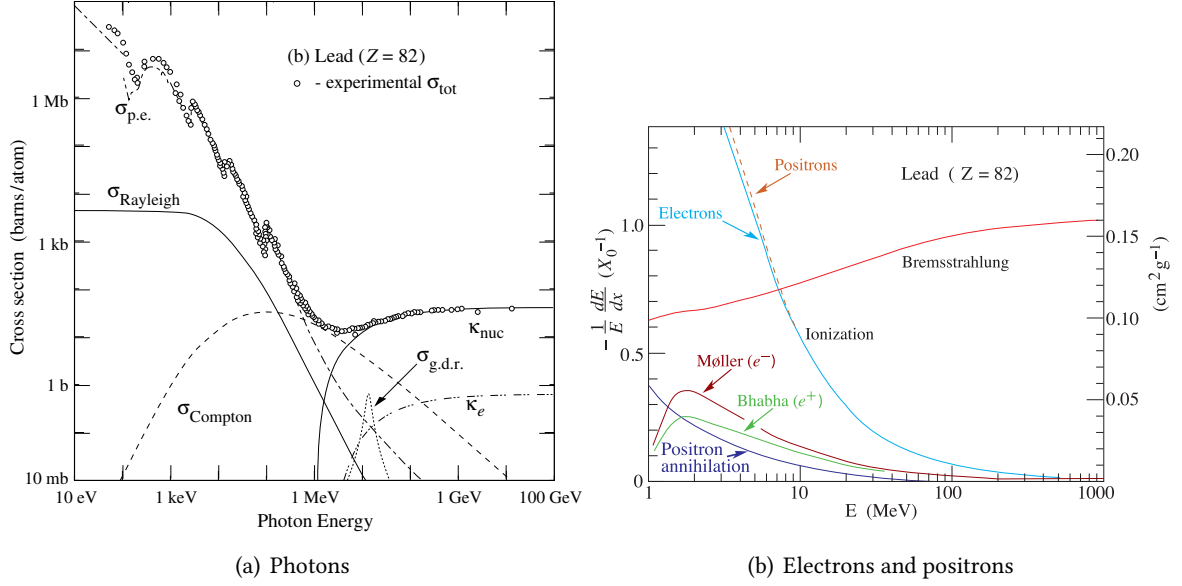
Figure 5.1: Energy losses in matter (lead) as a function of the particle energy. For photons, the dominant processes are photoelectric effect ( \sigma_{p.e.} ) at low energy and pair production ( \kappa ) at energies higher than a few MeV (see [1] for more explanations about the notations).
