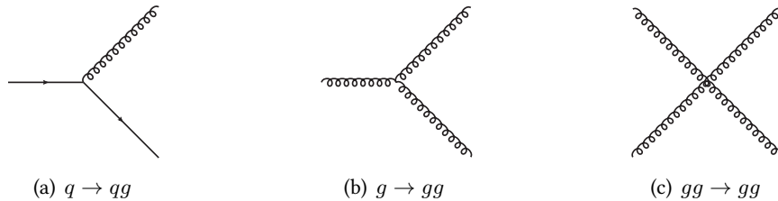
Figure 1.2: Possible vertices in the QCD theory. Only the first one is possible in QED with photons instead of gluon.
