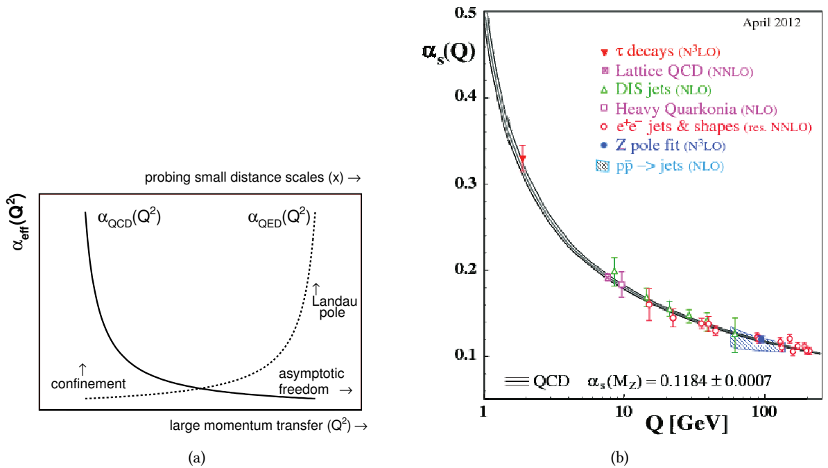
Figure 1.3: Strong coupling evolution: (a) compared to the QED coupling evolution (schematic) and (b) compared to the various measurements taking as reference the point \alpha_s(m_Z) [13].
