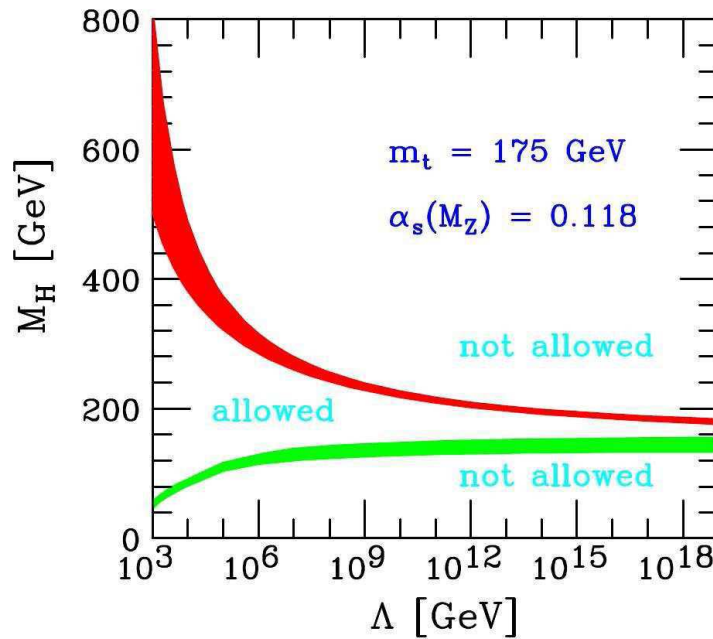
Figure 1.13: Theoretical limits on the Higgs boson mass [29].
