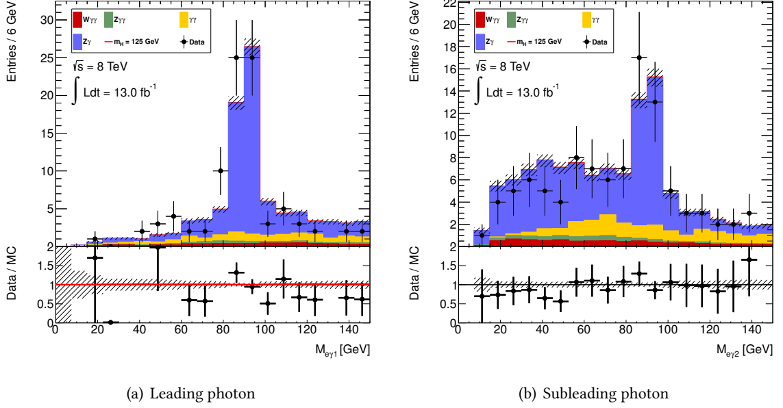
Figure 7.10: Electron-photon invariant mass distribution for the leading and subleading photon for events having at least one lepton for background Monte Carlo samples and data [188].
