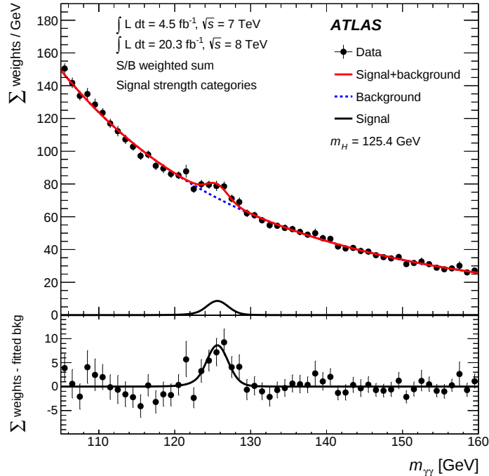
Figure 7.34: Diphoton invariant mass spectra observed in combined 2011+2012 dataset. The events are weighted by the signal-to-noise ratio of each category [125].
