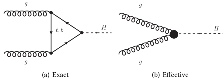
Figure 8.4: Diagrams of the ggH production in the exact and effective theory at leading order in \alpha_S (LO).
