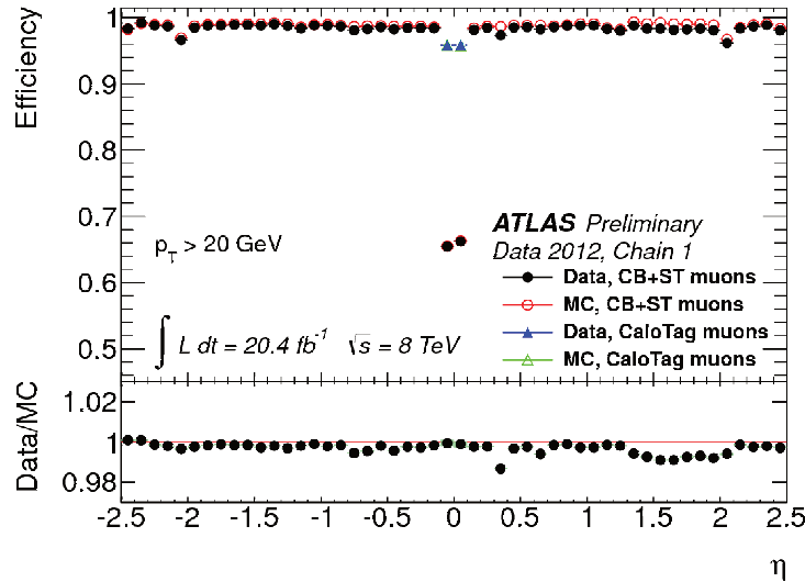
Figure 4.17: Muon reconstruction efficiency in 2012 data [77].
