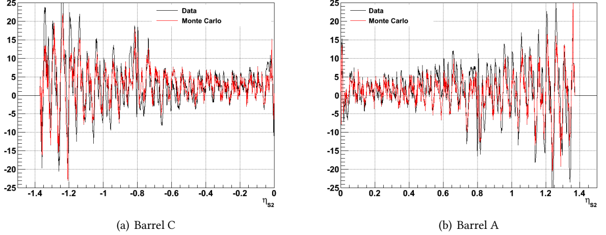
Figure 5.40: Comparison of \Delta z profiles as a function of the pseudorapidity in the barrel for data (black) and Monte Carlo (red) [100].
