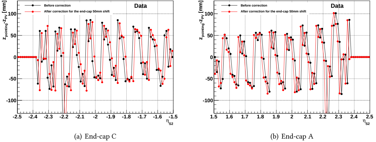
Figure 5.28: Comparison of the \Delta z profiles obtained with respect to the pseudorapidity reconstructed from the centre of the detector \eta_{S2} and the corrected pseudorapidity taking into account the end-caps shift \eta'_{S2} . One point corresponds to half a cell in the second layer \Delta\eta = 0.025/2 [100].
