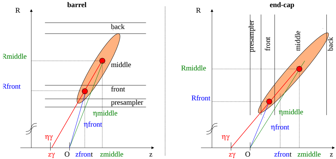
Figure 5.22: Illustration of the pointing technique in the barrel (left) and in the end-caps (right) (adapted from [98]).
