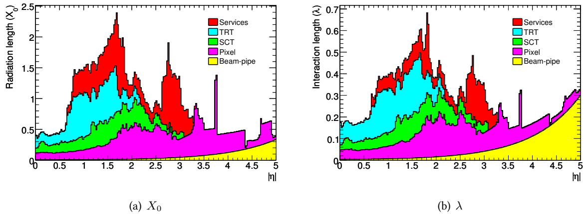
Figure 4.6: Material in front of the electromagnetic calorimeter in terms of radiation length as a function of the pseudorapidity \eta and integrated along \phi [57].
