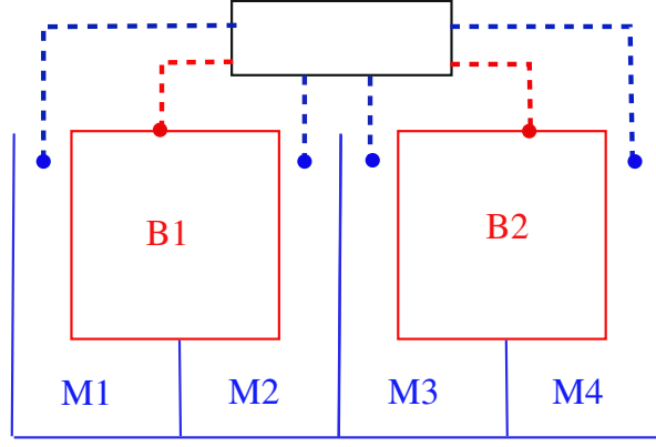
Figure 5.29: Electronics layout in the end-cap: two back and four middle cells are connected to the same electronics card. Electric connections are longer for M1 and M4 middle cells than for M2 and M3. Scheme is not to scale. [100].
