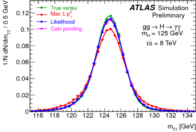
Figure 5.23: Higgs mass resolution in the diphoton channel when the selected primary vertex is the highest \sum p_T^2 one or the vertex is selected with pointing. This last method considerably improved the resolution [99]. The likelihood method will be presented in Chapter 6.
