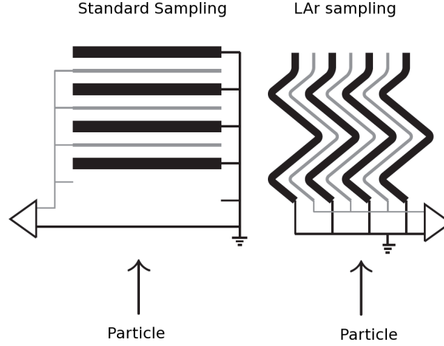
Figure 4.8: Accordion geometry on the right compared to the standard geometry on the left [59].
