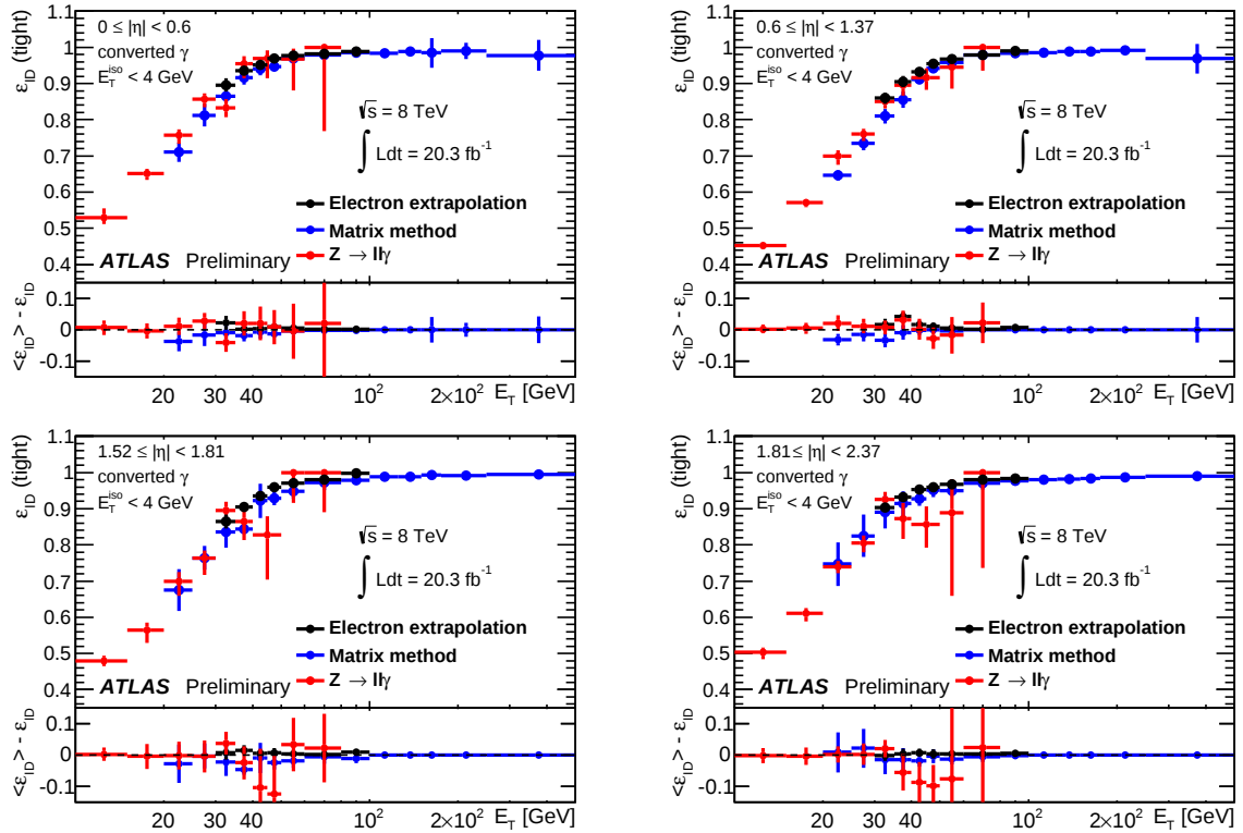
Figure 6.17: Converted photon identification efficiency in 2012 data from data-driven techniques as a function of the photon E_T , in four \eta regions [114].
