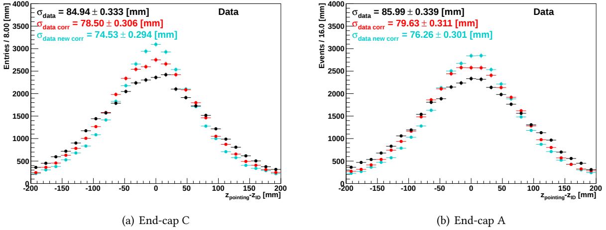
Figure 5.36: Improvement of the \Delta z resolution due to the bin-by-bin correction in data. The new correction (blue) is compared to the previous one (red) and to the uncorrected data (black) [100].
