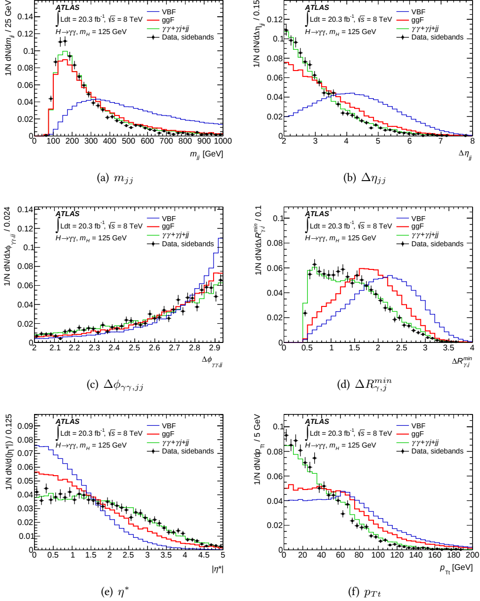
Figure 7.3: Distributions of the six variables entering the BDT for the signal (VBF), resonant background (ggH) and non-background (from data sidebands), after diphoton and 2-jet selection [125].
