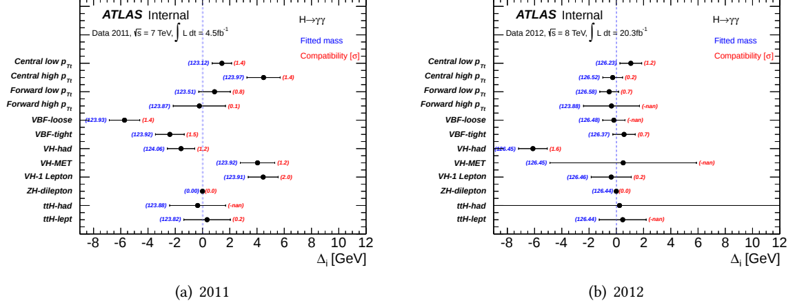
Figure 7.37: Compatibility among categories for 2011 and 2012 separately. The results for the ZH category are arbitrarily set to 0. The blue numbers are the fitted combined mass in each case. The red numbers are the compatibility with the blue combined mass from Equation 7.13 with two-sided asymptotic approximation [105].
