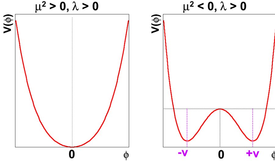
Figure 1.4: Illustration of the mexican hat Higgs potential in the case of U(1) global symmetry.
