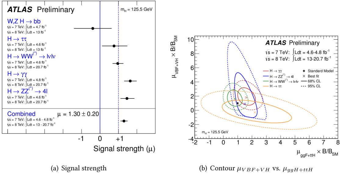
Figure 6.43: Couplings combination [176].
