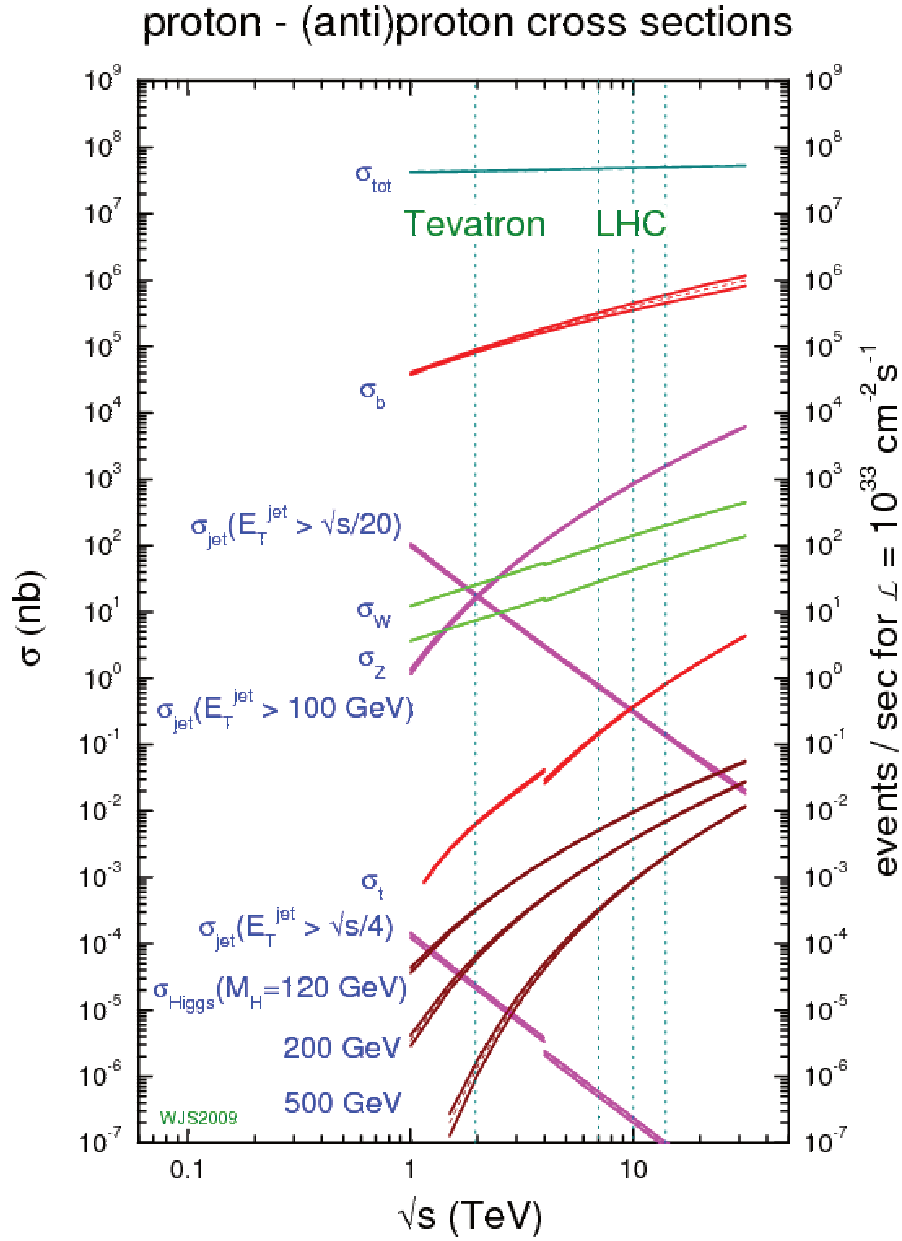
Figure 3.4: Expected cross section of sought signals and main backgrounds as a function of the centre of mass energy for pp and p\bar{p} collisions. Computations are performed up to NLO or NNLO with the corresponding MSTW2008 parton distribution set [55].
