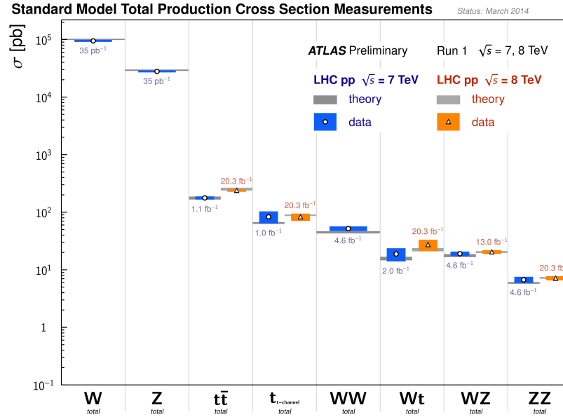
Figure 1.17: Preliminary cross section of several processes measured by ATLAS and compared to the Standard Model predictions [37].
