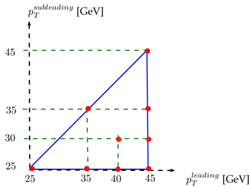
Figure 6.7: p_T configurations considered for the kinematics cut optimization.
