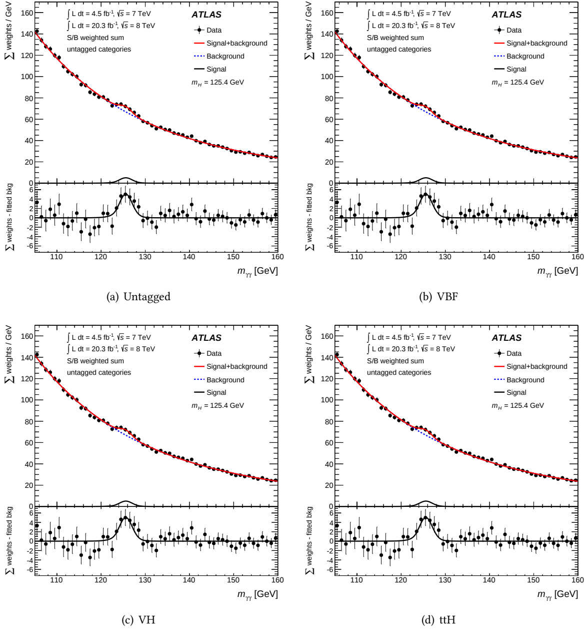
Figure 7.35: Diphoton invariant mass spectra observed in combined dataset for the different groups of categories. The events are weighted by the signal-to-noise ratio of each category [125].
