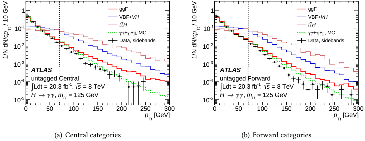
Figure 7.25: p_{Tt} distributions in the untagged categories [125].
