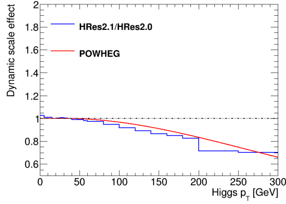
Figure 8.12: Effect of the dynamical scale in POWHEG (from a fit) and HRes2.1 (histogram). Ratio of the p_T^H distributions with to without dynamical scales.
