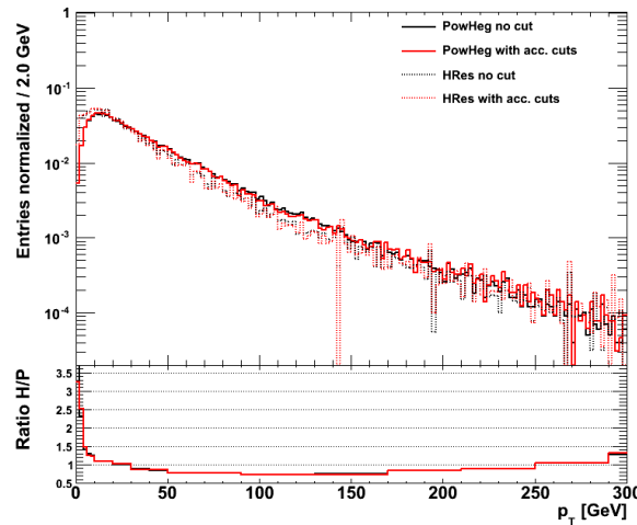
Figure 9.8: Effect of the acceptance cuts on the reweighting function using HRes1.0 .
