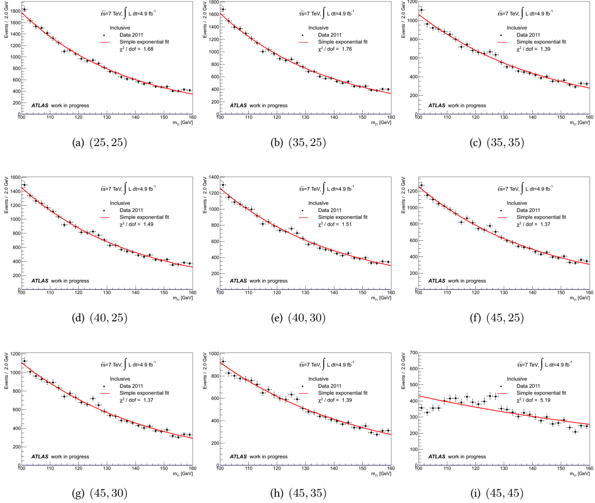
Figure 6.9: Diphoton invariant mass distribution in data for different (p_T^{\text{leading}}, p_T^{\text{subleading}}) [GeV] cuts configurations. The result of an exponential fit of these data points on the whole mass range is superimposed [108].
