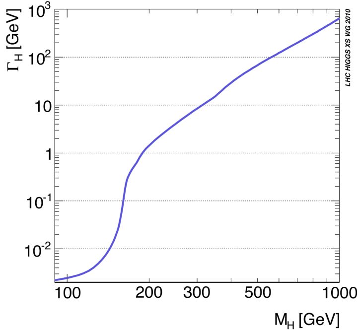
Figure 1.7: Higgs boson natural width [27].
