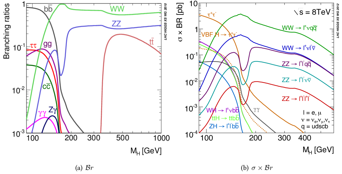
Figure 1.8: Higgs decay branching ratio in the Standard Model [27]
