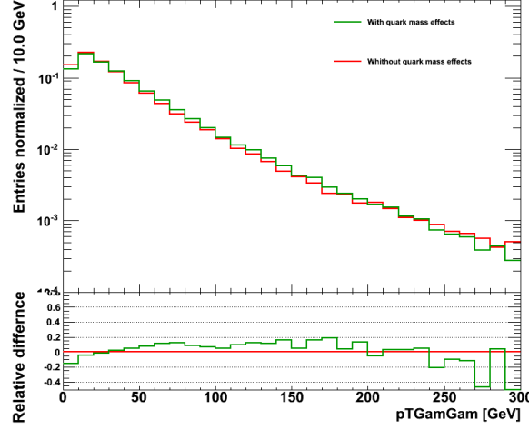
Figure 9.4: Effect of the top and bottom masses in POWHEG (a single scale).
