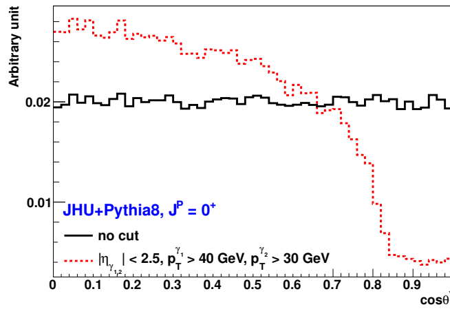
Figure 6.45: The distribution of |\cos(\theta^*)| for a scalar, without (black line) and with (red line) p_T cuts on the photons. The kinematic cuts distort the flat shape [179].
