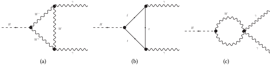
Figure 1.9: Higgs decay to two photons at lowest order in the Standard Model.
