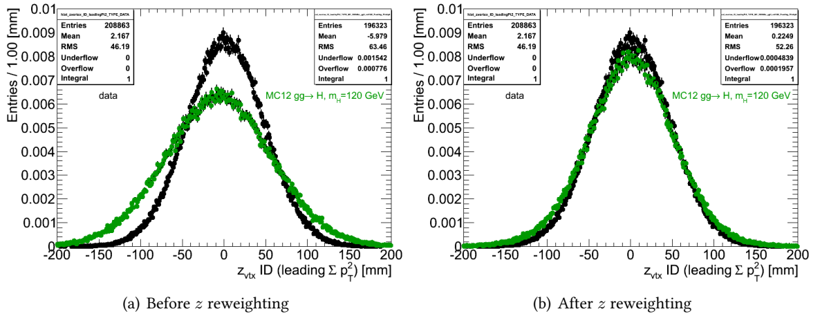
Figure 6.24: z reweighting correction of the Monte Carlo.
