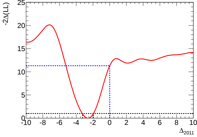
Figure 7.39: Likelihood scan of the \Delta_{2011} parameter of interest [105].
