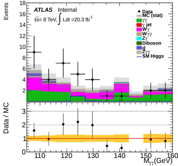
Figure 7.9: Background composition in the VH E_T^{miss} category from Monte Carlo [105].
