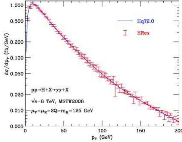
Figure 8.8: Comparison of HqT and HRes1.0 p_T^H spectra [229].
