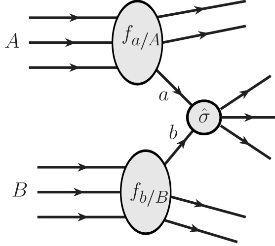
Figure 8.1: Illustration of the short and long distance effect in the QCD factorization theorem.
