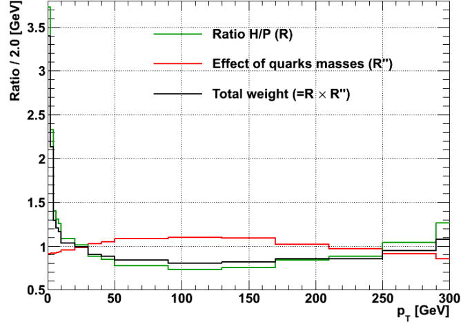
Figure 9.5: Reweighting POWHEG+PYTHIA8 to HRes1.0 at 8TeV for a Higgs mass of 125GeV.
