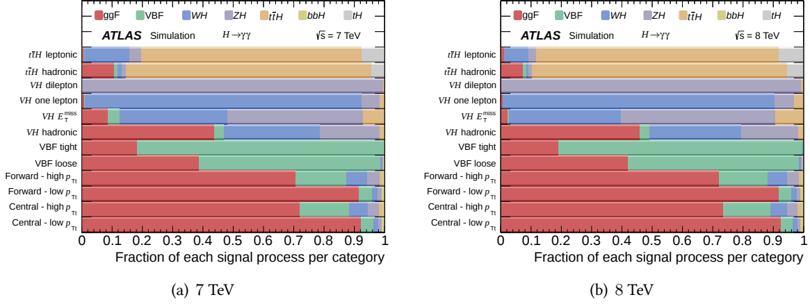
Figure 7.29: Category composition in terms of signal processes for the 7 and 8 TeV Standard Model predictions [125].
