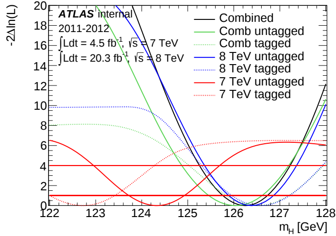
Figure 7.42: Likelihood scan of m_H in the tagged and untagged categories in 2011, 2012 dataset and the combination [105].
