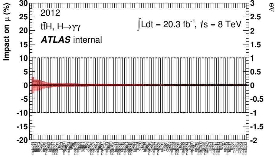
Figure 7.33: b -tagging nuisance parameters effect on the \mu uncertainty using only the t\bar{t}H categories (red area). Only the first ten are kept in the analysis [195].
