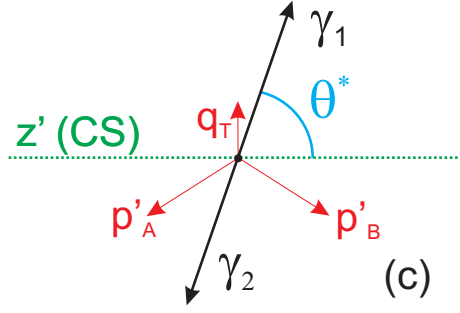
Figure 6.44: Illustration of the sensitive angular variable in the resonance's rest frame, \theta^* . It is calculated with respect to the z -axis in the Collins-Soper (CS) frame: p'_A is the momentum of the beam, and p'_B is the target momentum in the CS system, and then the z -axis of the CS coordinate system bisects the angle between p'_A and -p'_B , q_T is the unit vector of the direction opposite of (p'_A + p'_B)_T [179].
