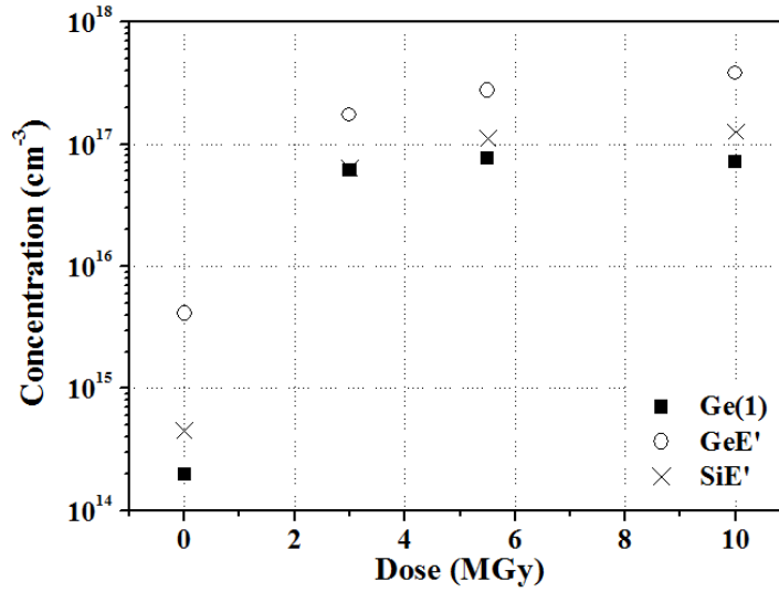
Figure 6.32: Defect concentration of the Ge-doped multi-mode fiber, as a function of the \gamma -radiation dose. The SiE' concentration was calculated from spectra recorded with P_{in} = 8 \cdot 10^{-4} mW and H_m = 0.1 G. The error coincides with the point dimension.
