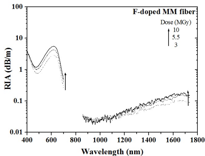
Figure 6.2: RIA spectra of the \gamma -irradiated F-doped multi-mode fibers at different doses: 3, 5.5 and 10 MGy.
