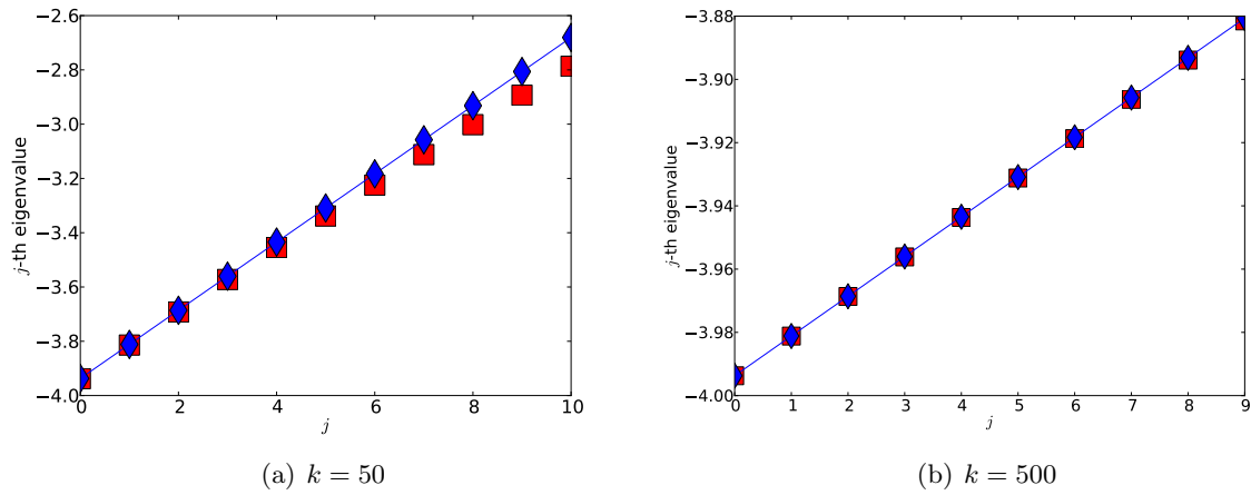
Figure 4.4: Eigenvalues in [-4, -4+20\pi k^{-1}] ; in red squares, the eigenvalues of A_k obtained numerically; in blue diamonds, the theoretical eigenvalues up to order k^{-2} ( i.e. forgetting the O(k^{-2}) in formula (4.22)).
