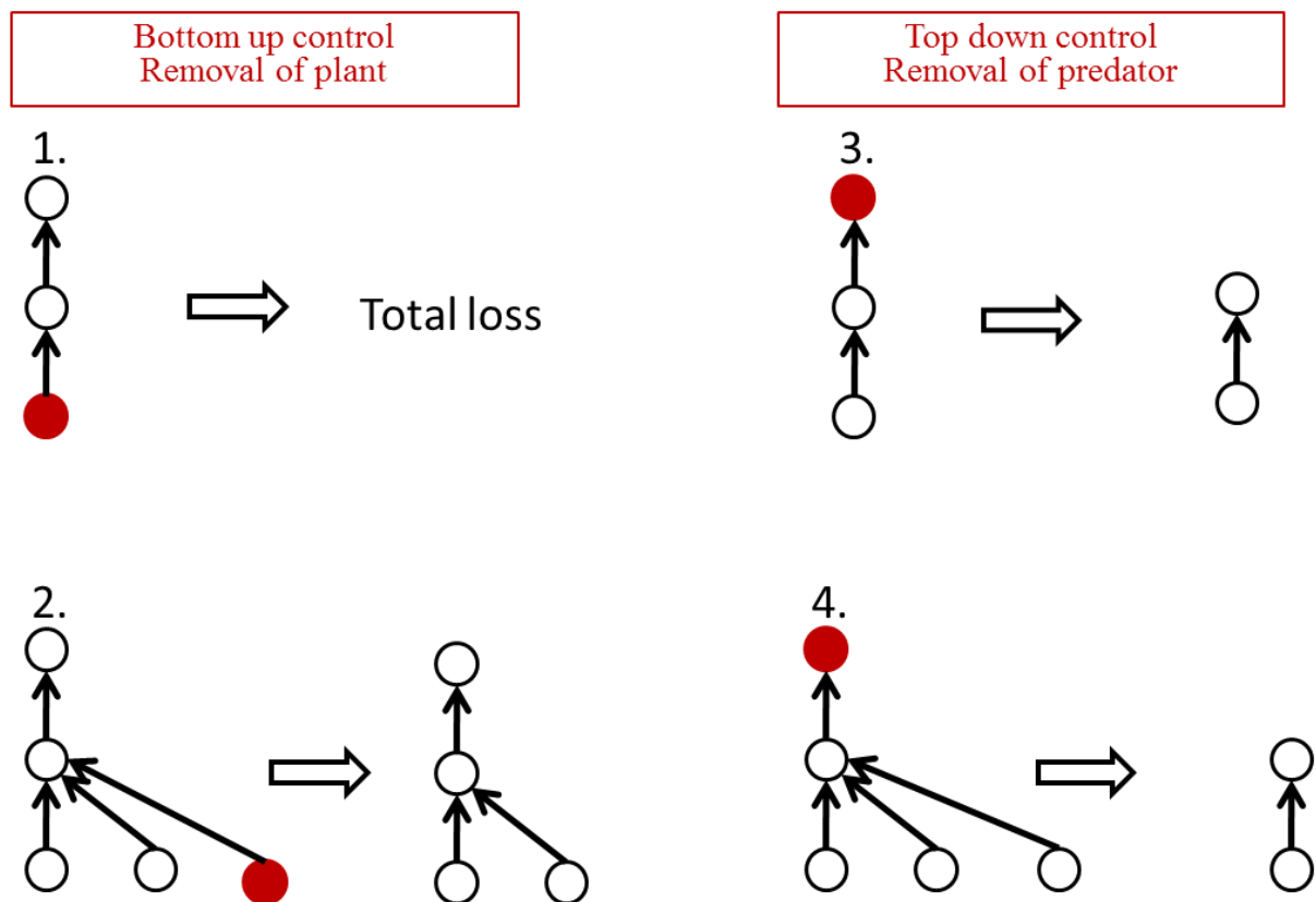
Figure II-3: Diagram representing the variation of food web reaction according to the species removed. Red ring are the removed species. Modified from Pimm, 1991. 1. The autotroph is essential for the chain. 2. The diversity of autotroph species in the consumer diet buffers the extinction of one of them. 3. The extinction of the top predator species leads to a shortening of the chain. 4. The top predator removal leads to an increased pressure of primary consumer, leading eventually to the extinction of some autotrophs.
