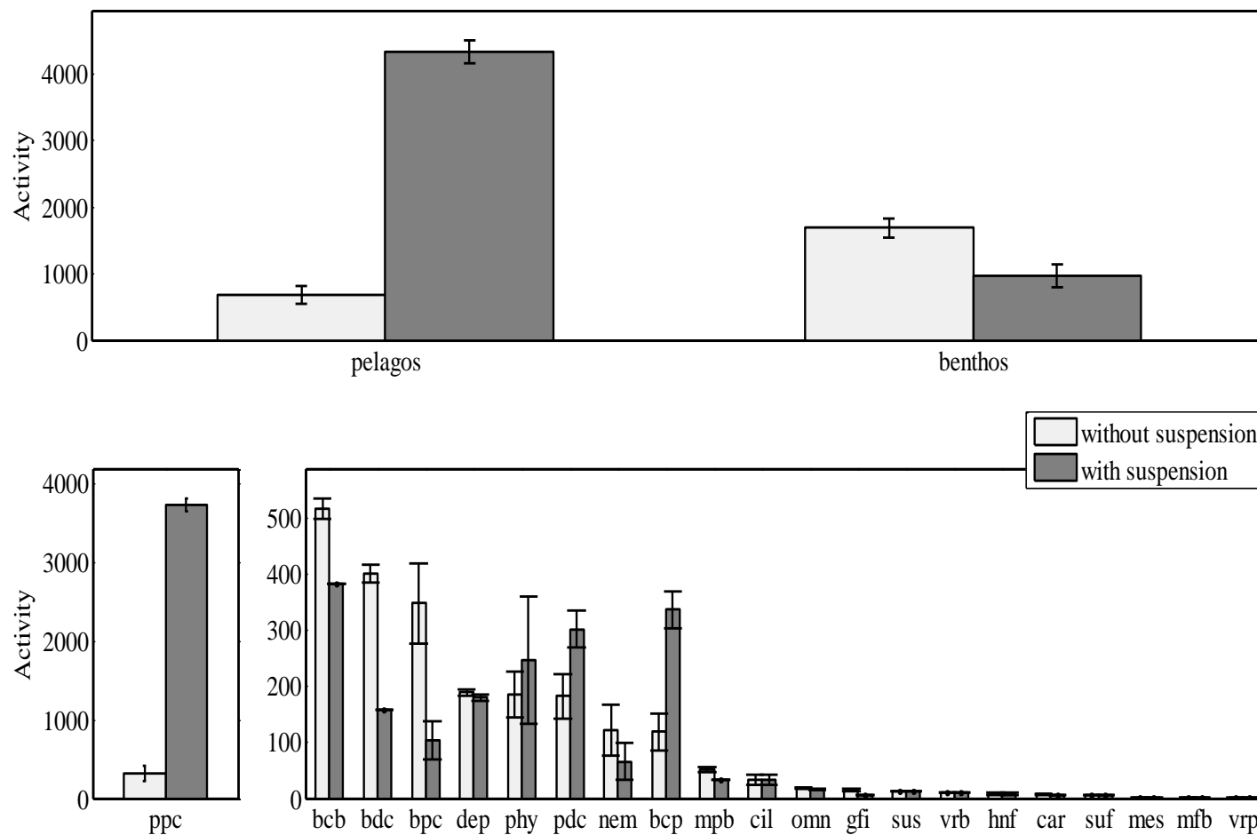
Figure V-2: Histogram presenting the activity of the compartments composing the food web. The activity corresponds to the sum of inflows and is expressed in mgC.m -2 per high tide. A) corresponds to the sum of the activity of all compartments for the benthos and the pelagos according to the 2 modeled situations. B) and C) refer to the activity of each compartment of the benthos and of the pelagos. See table V-1 for the abbreviations of the compartments.
