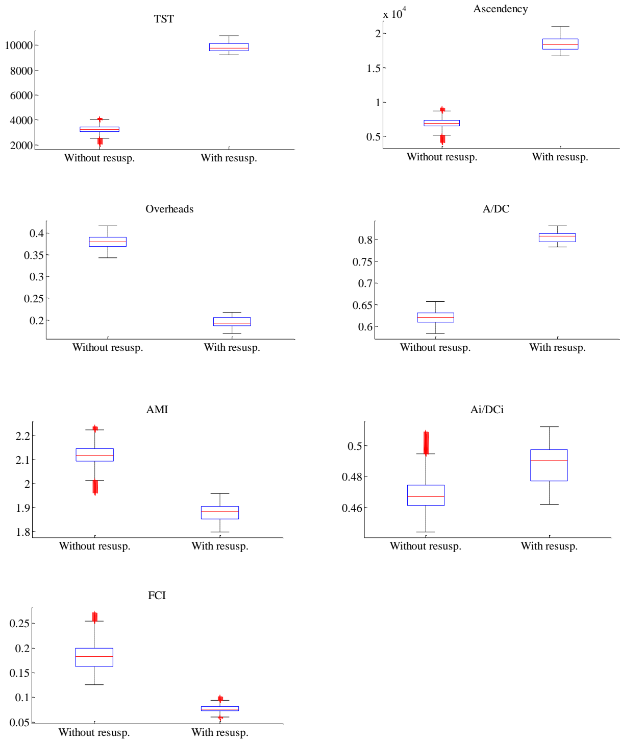
Figure V-5: Boxplots displaying the values of different ENA indices: the total System Throughput (TST), the Ascendency, the overheads, the relative Ascendency (A/DC), the Average mutual Information (AMI), the internal relative Ascendency (Ai/DCi) and the Finn Cycling index (FCI). The indices were calculated from the 500,000 solutions coming from the MCMC-LIM method. Red crosses correspond to outliers. Medians of all these indices were significantly different for the two seasons (Wilcoxon test, H_0 was rejected, p -value < 0.01 ).
