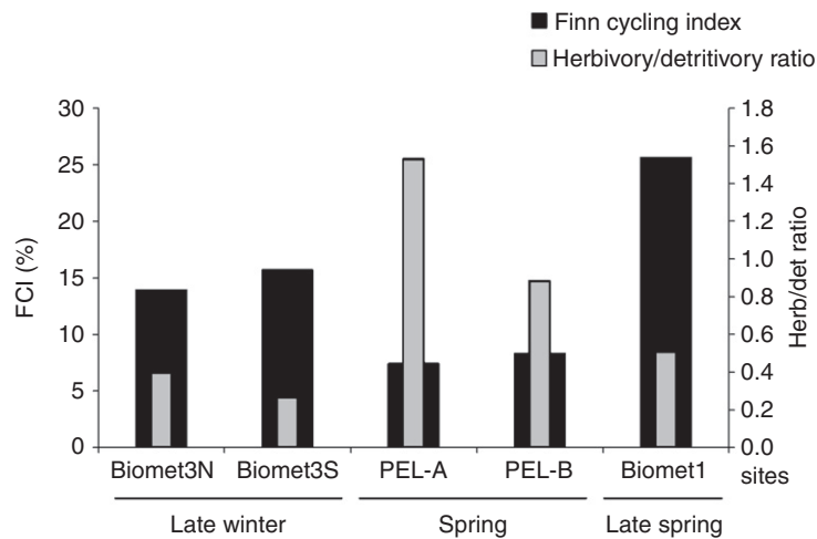
Figure 7 Dynamic of evolution of the Finn cycling index and herbivory/detrivory ratio along the development of the plankton succession in winter/spring in the Bay of Biscay (Marquis et al., 2007).
