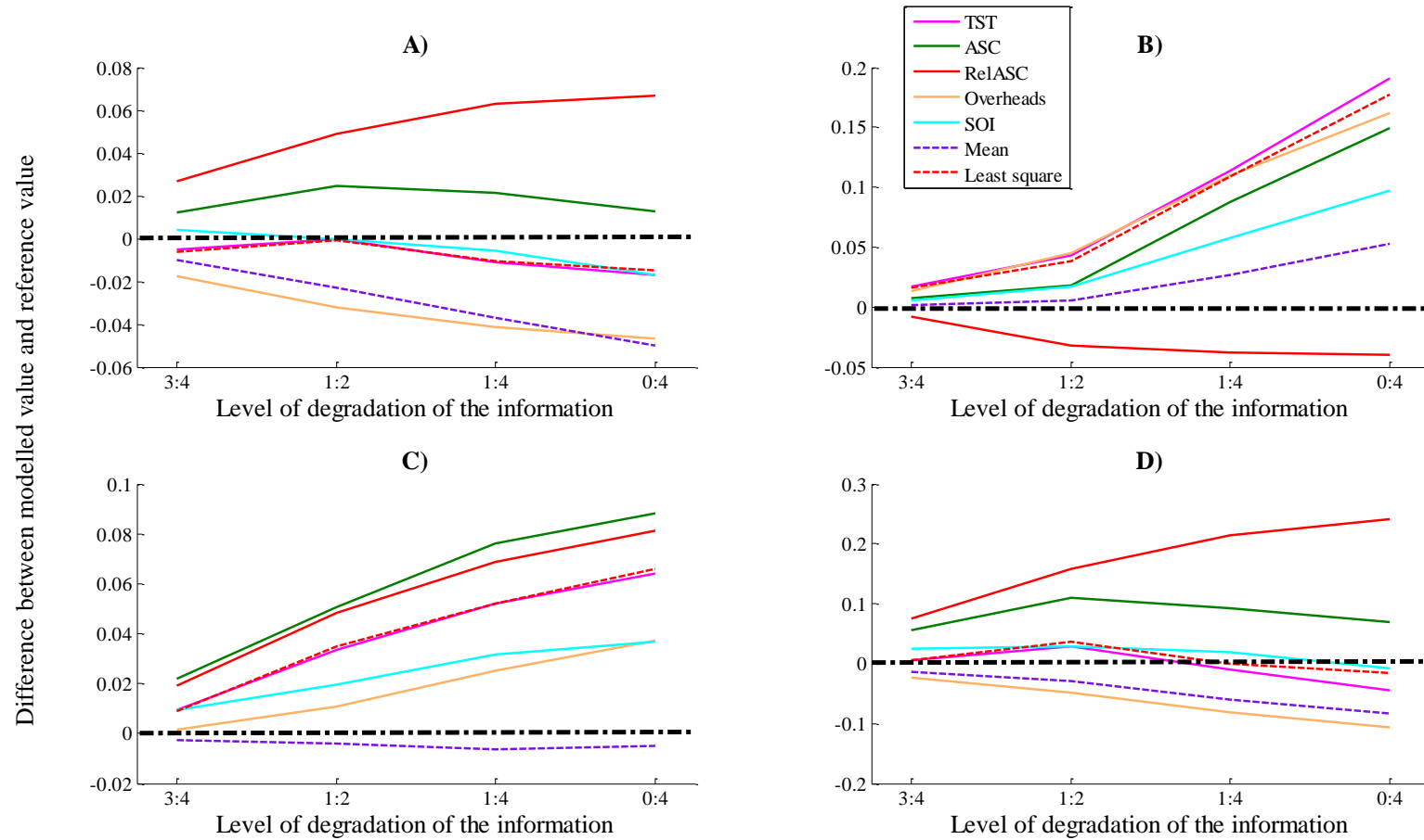
Figure III-5: Plot that represents the absolute difference between the values of 4 indices calculated either from the estimated value of flows or from the reference value of flows. The subplot (A) shows the relative Ascendency index, the second one (B) presents the FCI, the plot (C) presents the internal relative Ascendency index and the last one the AMI index (D). The dash-dot line corresponds to the estimated values of indices, which was equal to the reference value of indices. A curve located above a dash-dot line corresponds to an over-estimation of the considered index.
