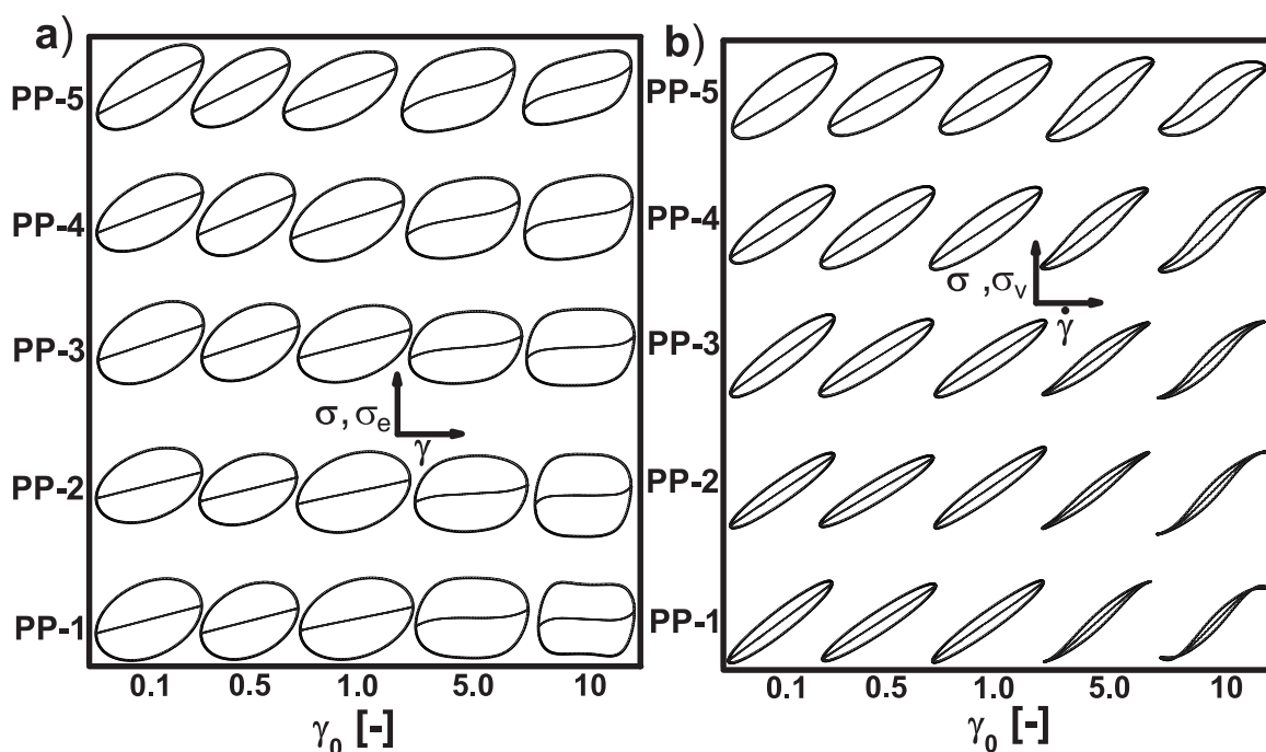
Figure B.3: Lissajous-Bowditch curves along with elastic and viscous stress as a function of applied deformation for PP-blends (a) elastic Lissajous-Bowditch curves (b) viscous Lissajous-Bowditch curves.
