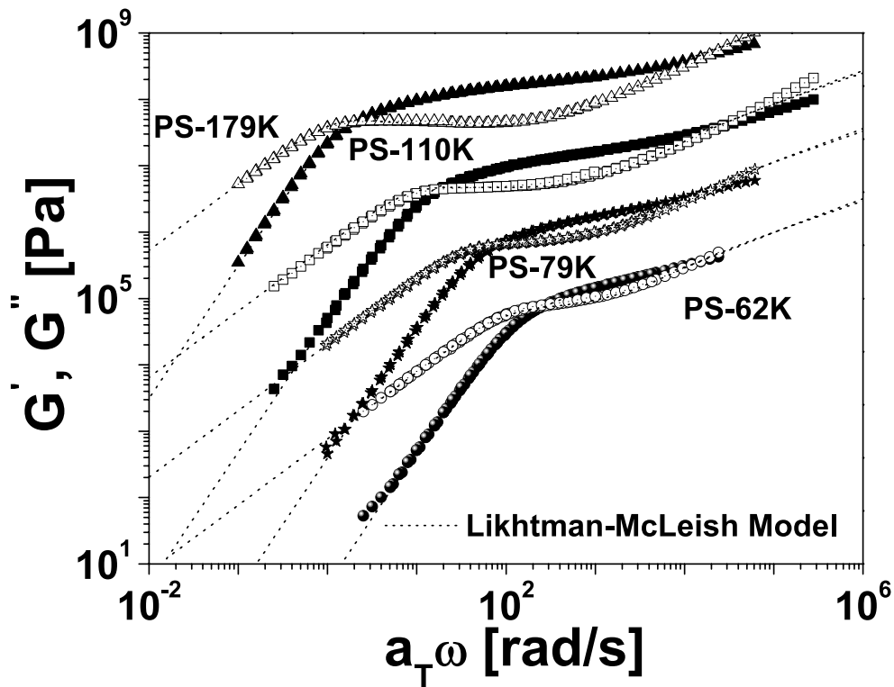
Figure 4.4: The linear master curve of monodisperse PS melts and prediction of Likhthman-McLeish model.
