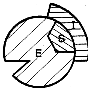
INHIBITION ANTICOMPETITIVE
