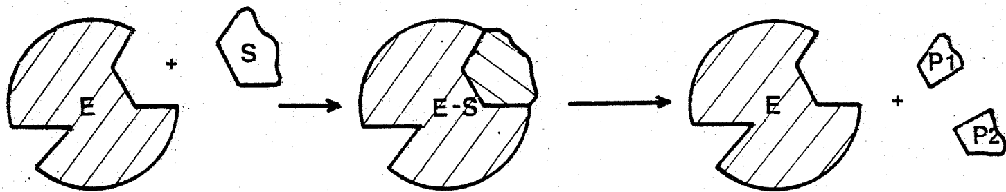
REACTION ENZYMATIQUE
