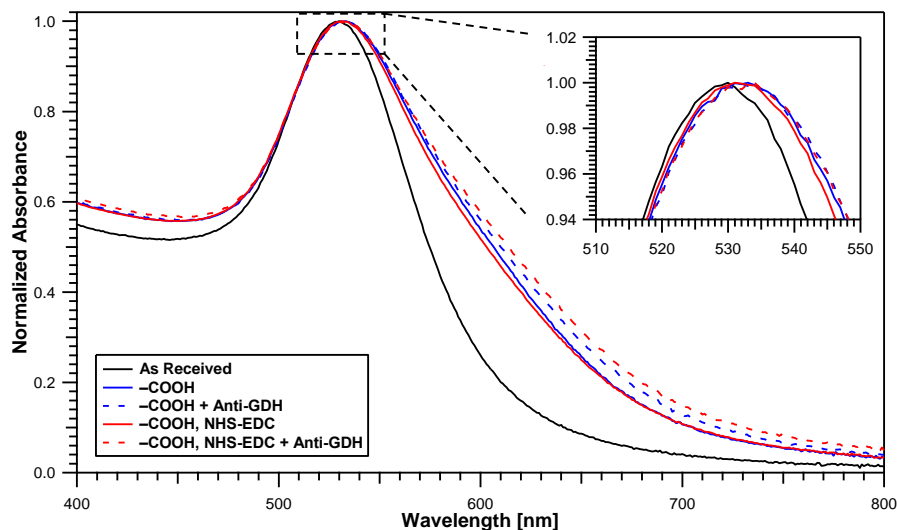
Figure A.1 Typical absorbance spectrum obtained after NPs functionalization with the –COOH thiol and Anti-GDH before and after activation with NHS-EDC. All spectra are re-normalized to their maximum to better see their shape and get rid of differences in height due to concentration only.
