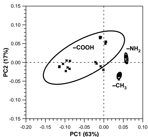
Figure 4.5 Scores plot for PCA calculations performed on ToF-SIMS spectrum after adsorption of \beta\text{LG} on -\text{COOH} -, -\text{CH}_3 - and -\text{NH}_2 -terminated SAMs
