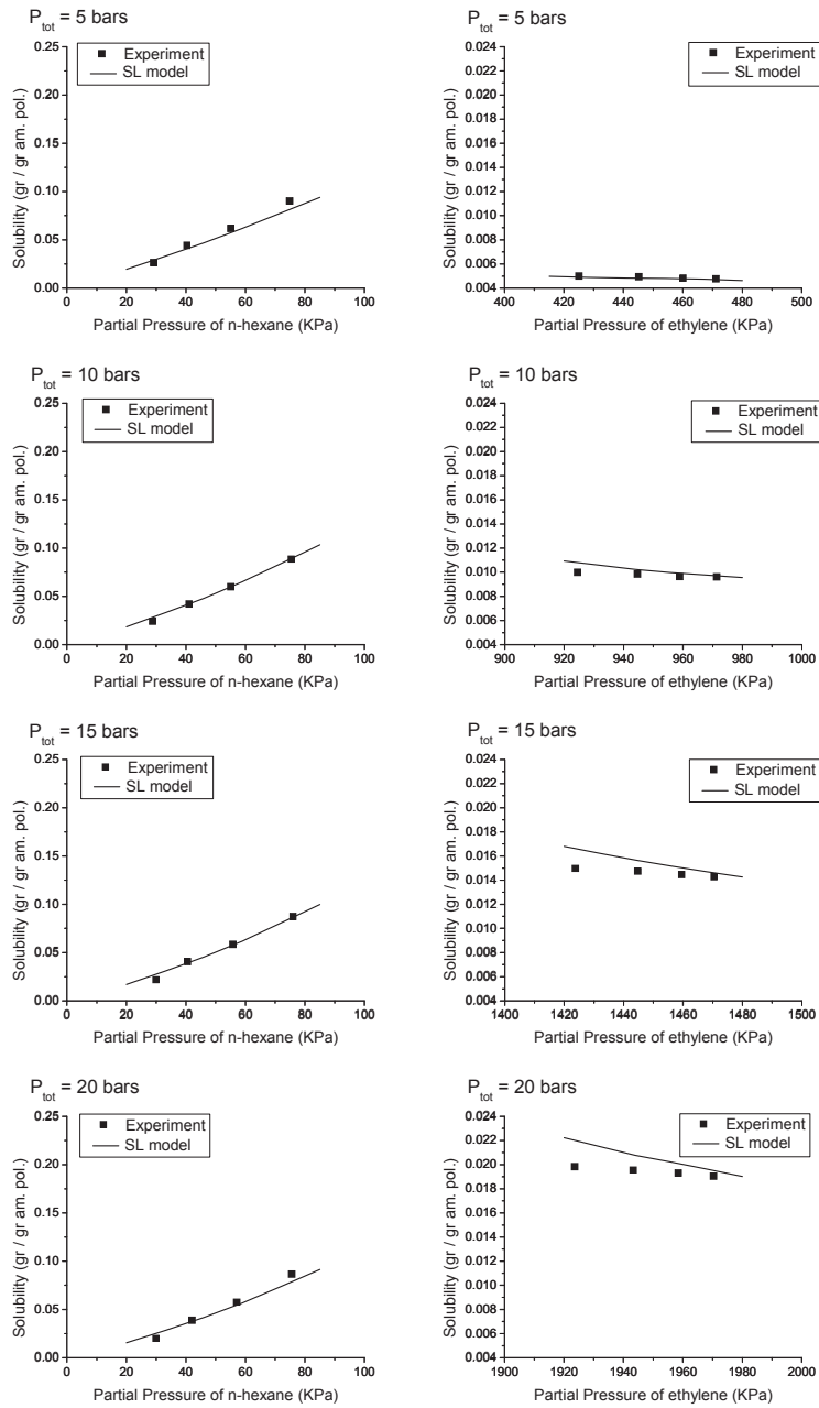
Figure 4.22. The solubility of n -hexane and ethylene in LLDPE in the ternary system of ethylene- n -hexane-LLDPE at 80 °C with P_{tot} = 5, 10, 15, \text{ and } 20 bars and its comparison with the prediction of the ternary Sanchez-Lacombe model with the corresponding binary interaction parameters of k_{12} = 0.00 , k_{13} = -0.022 , and adjusted k_{23} = 0.030 at 80 °C.
