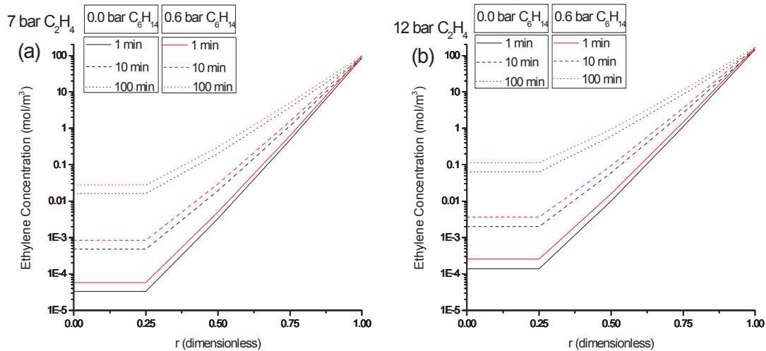
Figure 5.13. The predicted concentration gradient through the growing polymer particle and the effect of n -hexane as the ICA on it during polymerization with (a)7 and (b)12 bars of ethylene, respectively.
