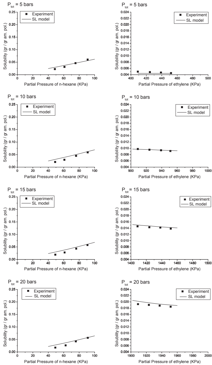
Figure 4.20. The solubility of n -hexane and ethylene in LLDPE in the ternary system of ethylene- n -hexane-LLDPE at 90 °C with P_{tot} = 5, 10, 15, \text{ and } 20 bars and its comparison with the prediction of the ternary Sanchez-Lacombe model with the corresponding binary interaction parameters of k_{12} = 0.00, k_{13} = -0.032, k_{23} = 0.038 at 90 °C.
