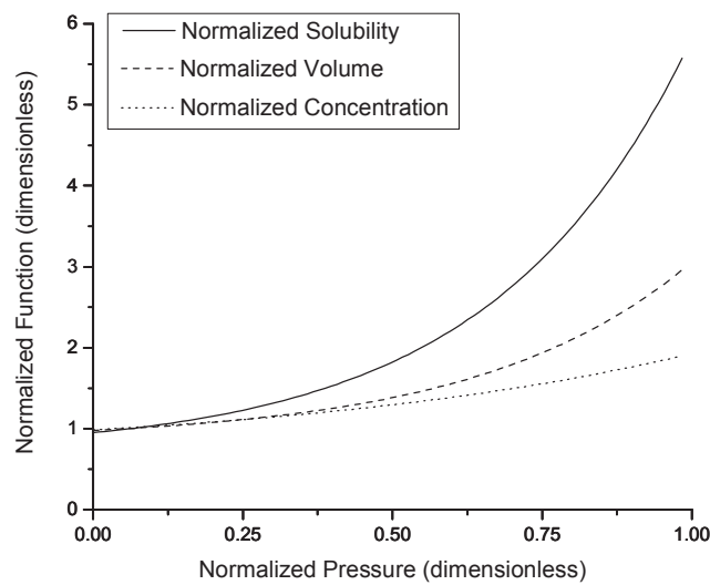
Figure 4.4. A priori simulation on effect of n -hexane on the ethylene solubility, swelling of amorphous phase of LLDPE, and ethylene concentration in the amorphous phase of LLDPE at typical polymerization condition of 80 °C temperature and 10 bars of ethylene partial pressure.
