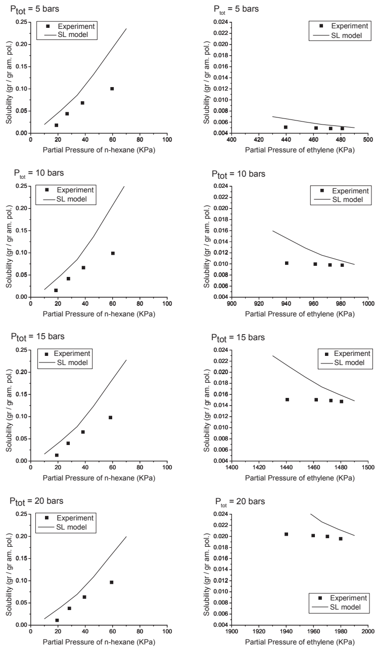
Figure 4.18. The solubility of n -hexane and ethylene in LLDPE in the ternary system of ethylene- n -hexane-LLDPE at 70 °C with P_{tot} = 5, 10, 15, and 20 bars and its comparison with the prediction of the ternary Sanchez-Lacombe model with the corresponding binary interaction parameters of k_{12} = 0.00, k_{13} = -0.014, k_{23} = 0.010 at 70 °C.
