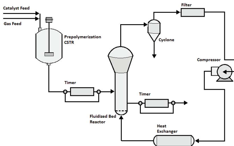
Figure 2.8. Process overview of gas phase ethylene polymerization on supported catalyst inside FBR.
