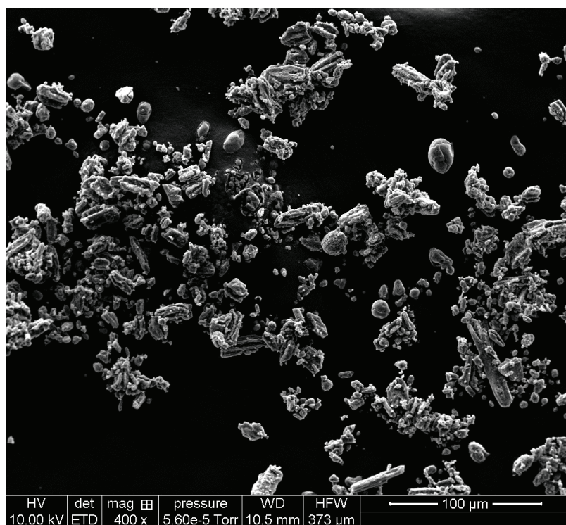
Figure 5.10. SEM image of powder of Ziegler-Natta catalyst supported on MgCl_2 .
