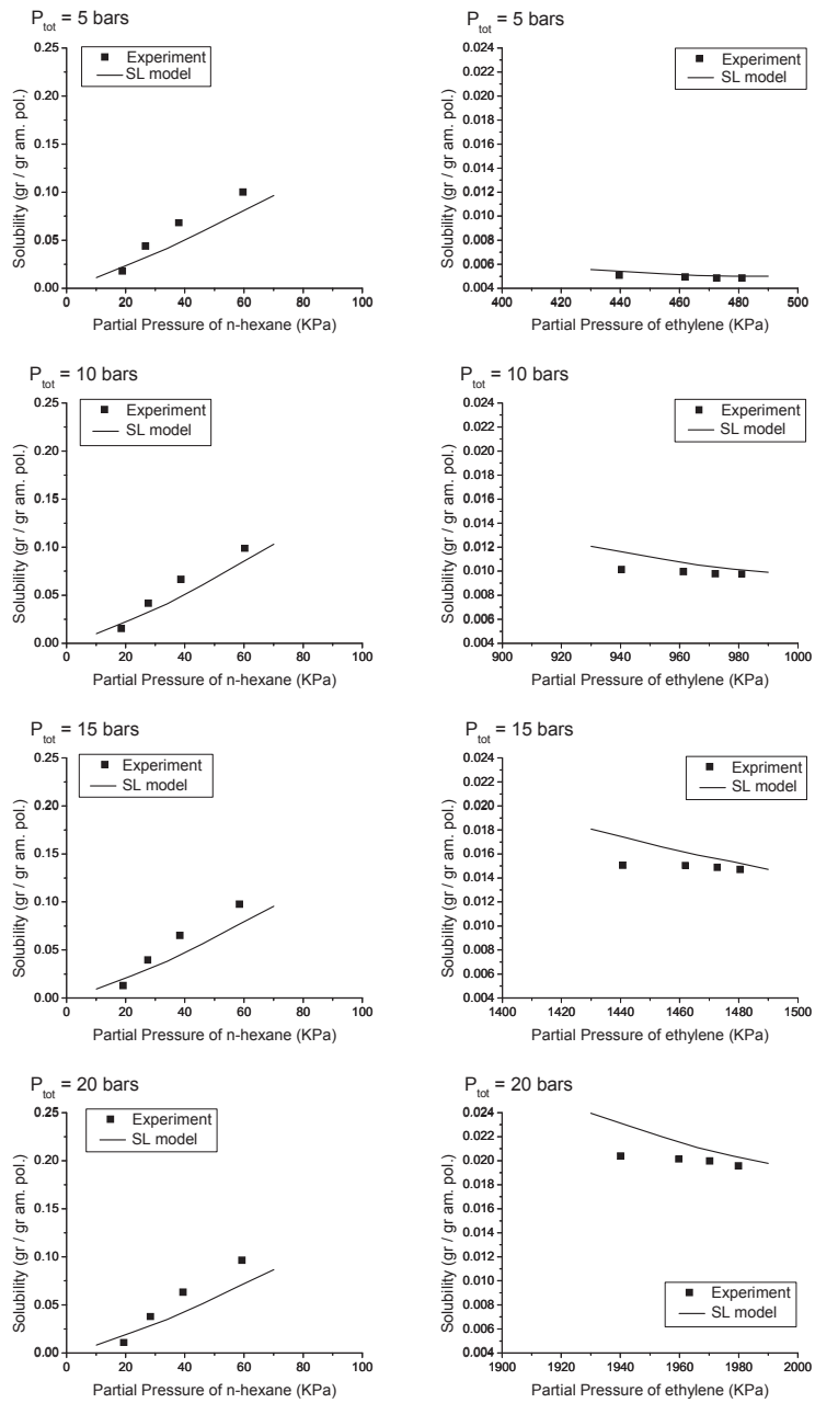
Figure 4.21. The solubility of n -hexane and ethylene in LLDPE in the ternary system of ethylene- n -hexane-LLDPE at 70 °C with P_{tot} = 5, 10, 15, and 20 bars and its comparison with the prediction of the ternary Sanchez-Lacombe model with the corresponding binary interaction parameters of k_{12} = 0.00, k_{13} = -0.014, and adjusted k_{23} = 0.034 at 70 °C.
