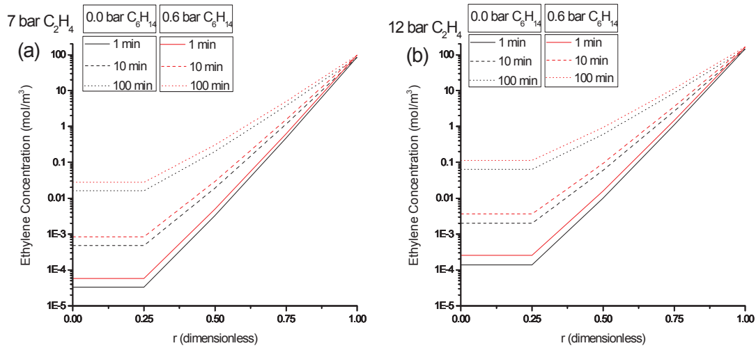
Figure 5.13. The predicted concentration gradient through the growing polymer particle and the effect of n -hexane as the ICA on it during polymerization with (a) 7 and (b) 12 bars of ethylene, respectively.
