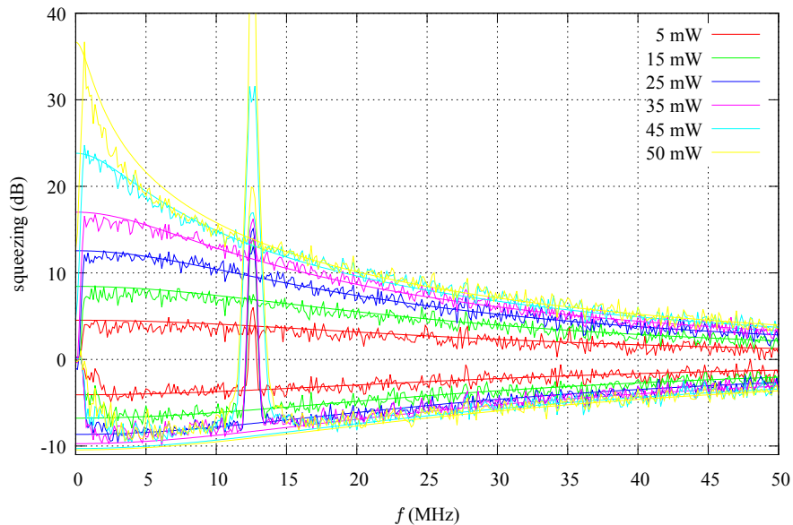
Figure 3.10: Squeezing and anti-squeezing versus frequency for different values of the pump power. The smooth line are theoretical fitting using equations 3.29 and 3.30 (with parameters \eta = 91\% , \omega_c = 65 MHz). All traces are normalized to the shot noise (i.e. S(\omega)/SN(\omega) ).
