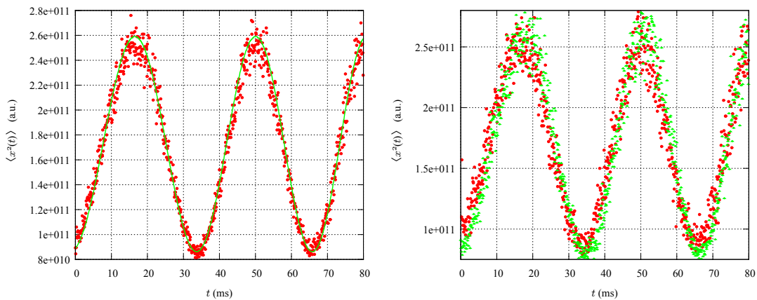
Figure 5.6: Temporal variance of the homodyne signal. Mean values of the variance for 0.1 ms long bins. On the left, the phase sweep is fitted with a second order non-linear model. On the right: two sets of data are represented, the first 15 s in red and in green the last 15 s of the measurement. We can see that the phase drift is very small (a little on the right). This confirms the reliability of the assumption that the phase is stable during one measurement.
