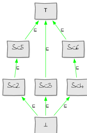
Figure 3.4: Lattice
