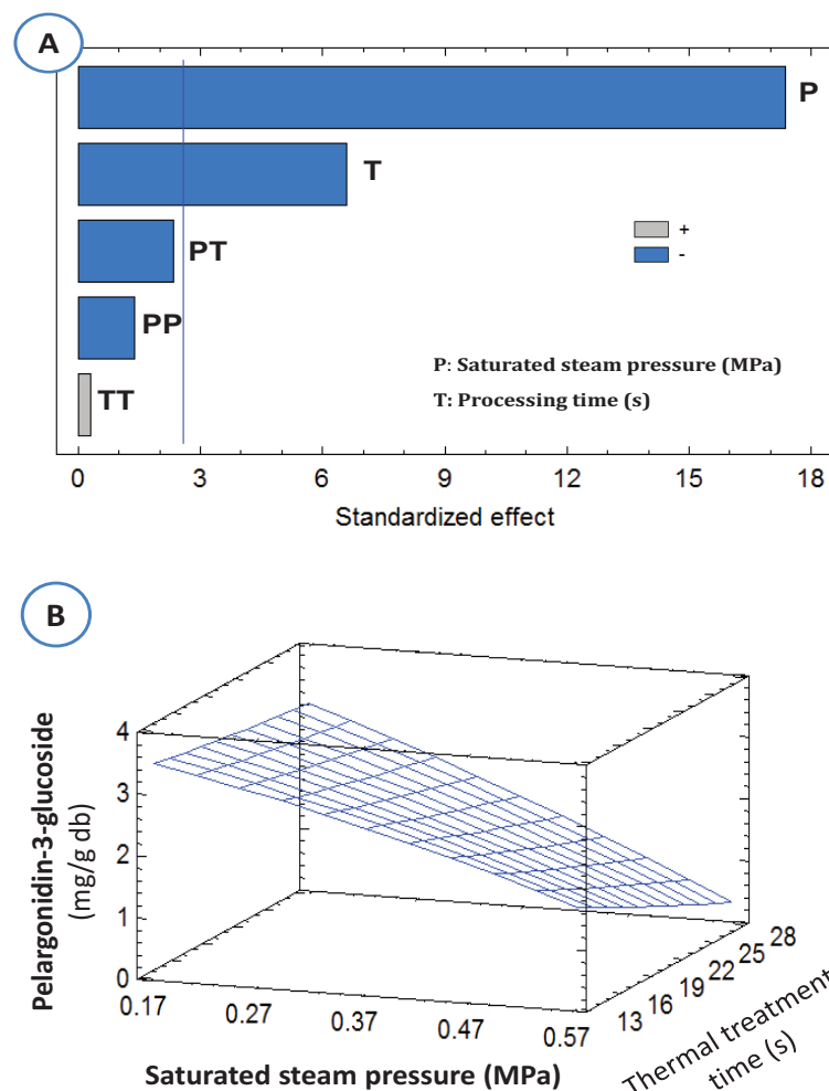
Figure 6. Effects of DIC parameters (saturated steam pressure; MPa and thermal treatment time; s) on the pelargonidin-3-glucoside (Pe-3-Gl; mg/g db) of SD strawberries. A) Pareto Chart and B) Response Surface.
