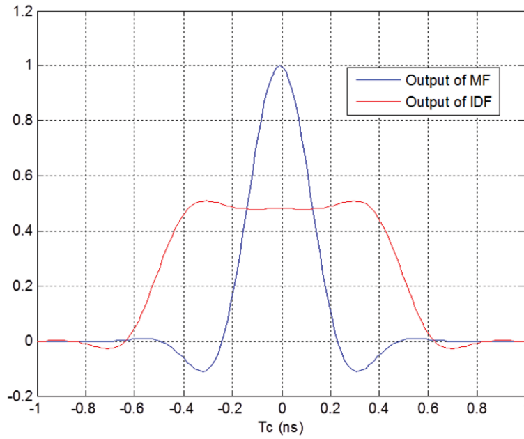
Figure 5.1.1: The output of matched filter (MF) and integrate-and-dump filter (IDF) of raised cosine pulse
