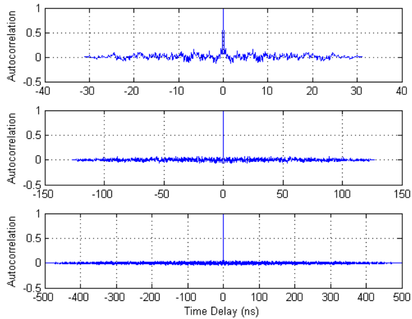
Figure 4.2.2: Autocorrelation function of Lorenz pluses with length T_s = 31ns , T_s = 127ns and T_s = 500ns .
