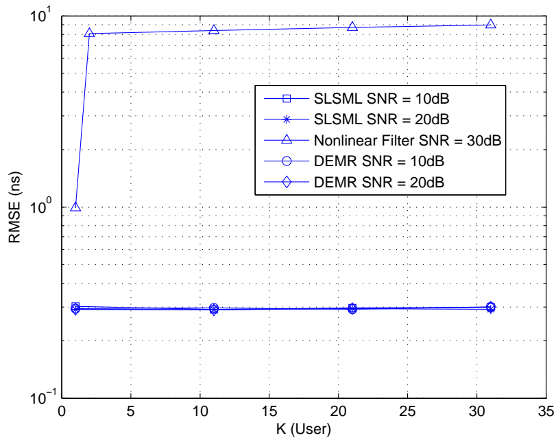
Figure 5.3.13: RMSE versus K for different SNR values with M = 600 , N = 31 , and near-far ratio is 10 dB in DS-UWB system in AWGN channel.
