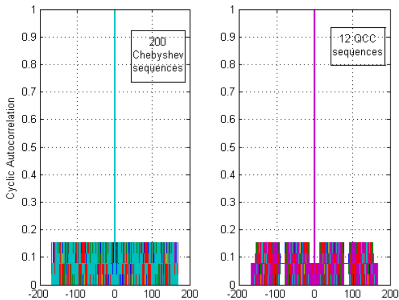
Figure 4.2.15: Cyclic autocorrelation function of selected Chebyshev sequences and QCC sequences with N_h = 13 .
