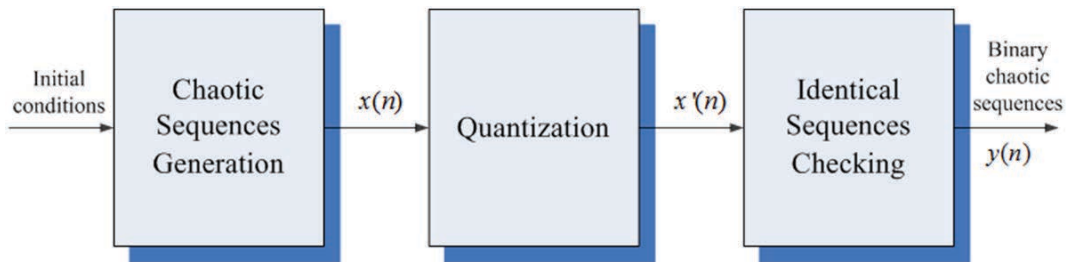
Figure R.9: The procedure of the generation of Binary chaotic sequences.
