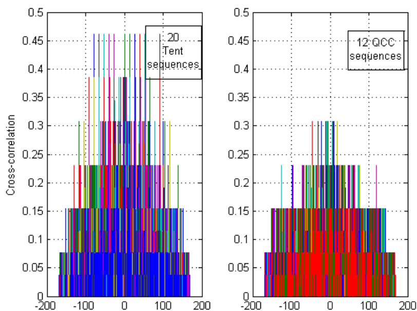
Figure 4.3.10: Cross-correlation function of selected Tent sequences and QCC sequences with N_h = 13 .
