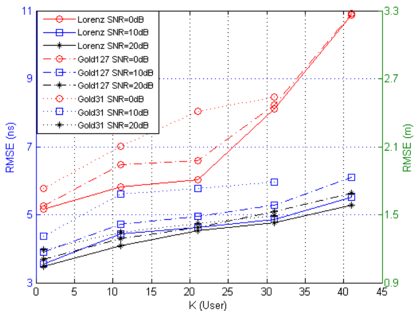
Figure 6.3.4: RMSE versus K for different SNR values with M = 100 , T_s = 127ns , and near-far ratio is 10 dB in CM1 channel.
