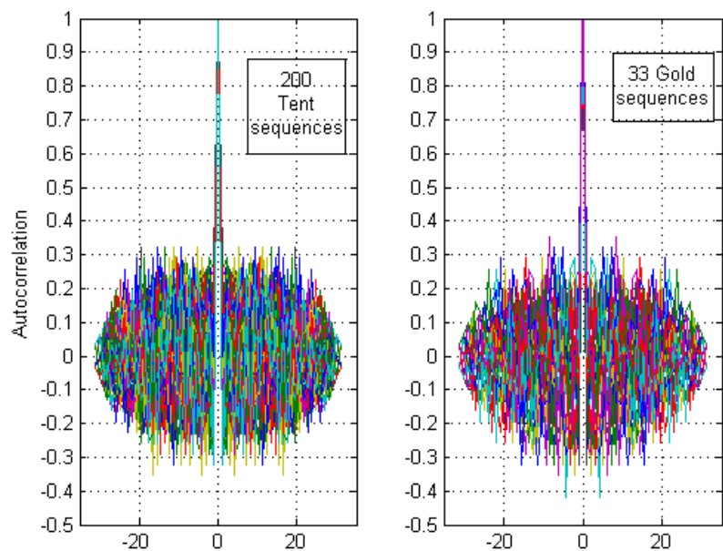
Figure 4.2.12: Autocorrelation function of selected Tent sequences and Gold sequences with length N = 31 .
