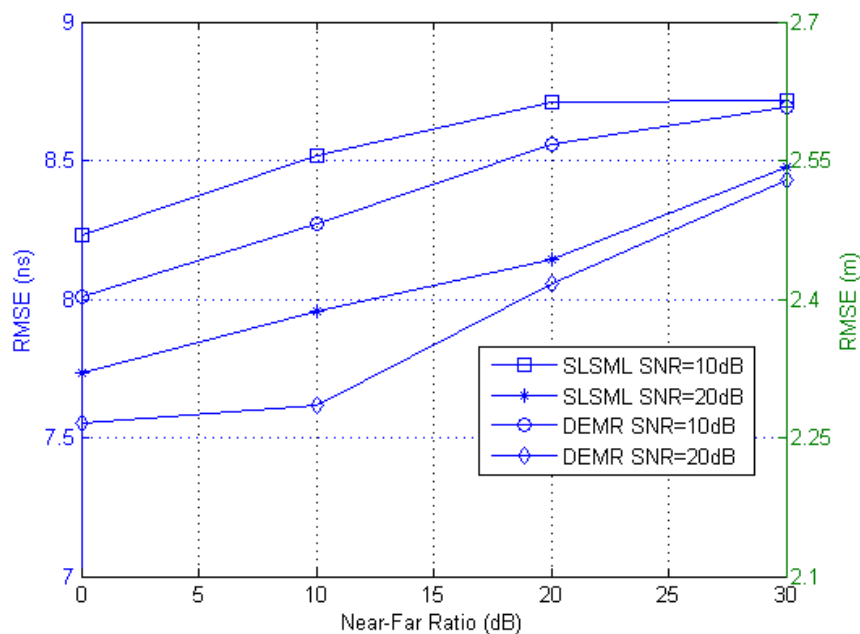
Figure 5.3.19: RMSE versus near-far ratio for different SNR values with M = 200 , N_h = 13 , and K = 10 in TH-UWB system in CM1 channel.
