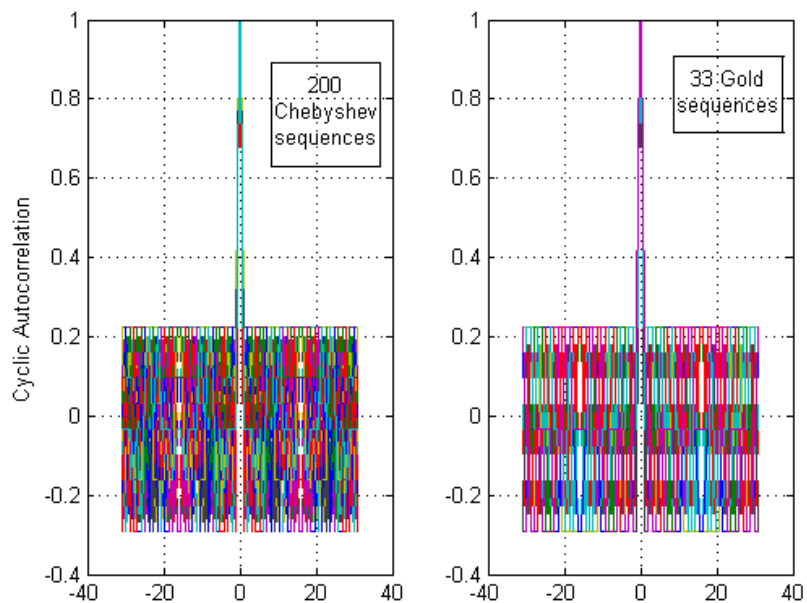
Figure 4.2.11: Cyclic autocorrelation function of selected Chebyshev sequences and Gold sequences with length N = 31 .
