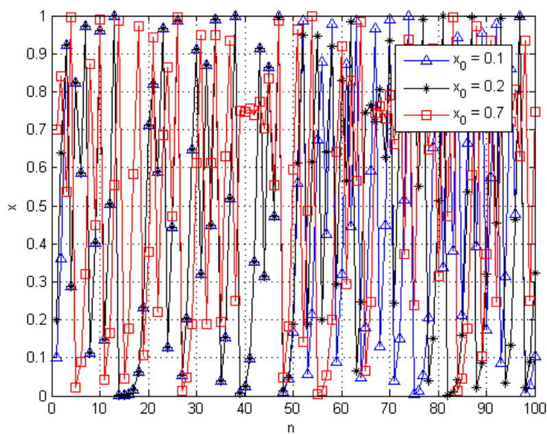
Figure 3.2.3: Trajectories of x_{n+1} = 4x_n(1-x_n) with the initial condition x_0 = 0.1 , x_0 = 0.2 , x_0 = 0.7 .
