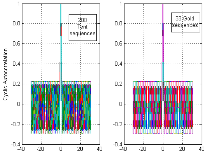
Figure 4.2.13: Cyclic autocorrelation function of selected Tent sequences and Gold sequences with length N = 31 .
