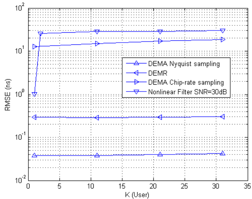
Figure 5.3.3: RMSE versus K for different estimators with M = 100 , N = 31 , SNR = 20dB and near-far ratio is 10 dB DS-UWB system in AWGN channel.
