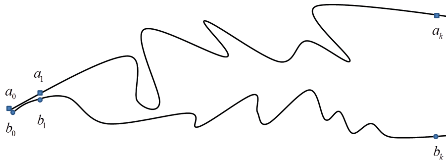
Figure 3.1.1: Schematic diagram of the sensitivity of a chaotic system under different but very close initial conditions a_0 and b_0 .
