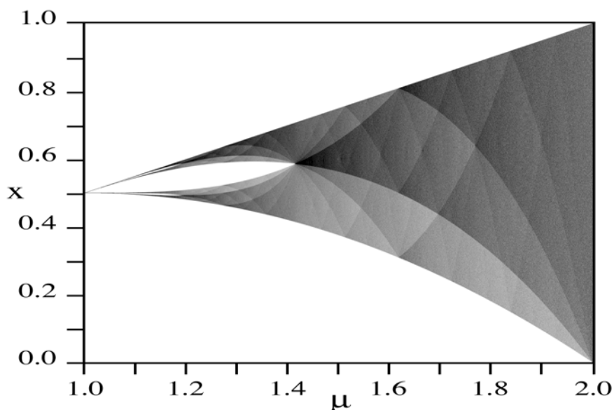
Figure 3.2.6: Bifurcation diagram of Tent map.
