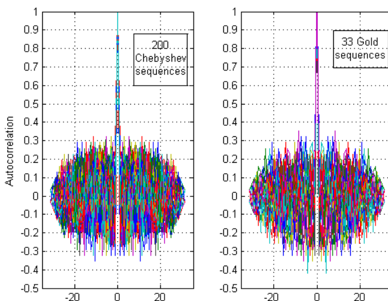
Figure 4.2.10: Autocorrelation function of selected Chebyshev sequences and Gold sequences with length N = 31 .
