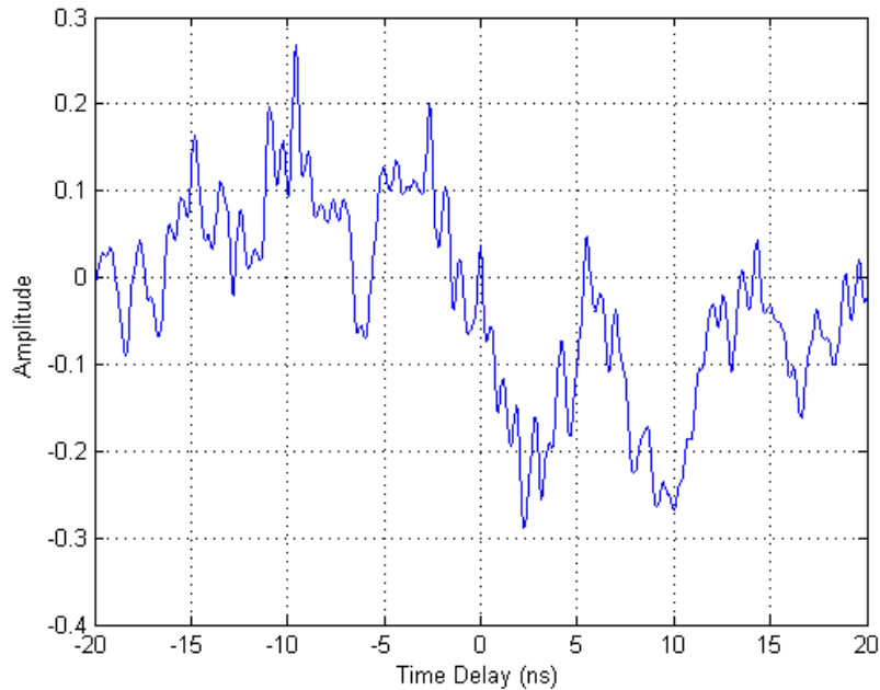
Figure 4.3.1: Cross-correlation function of typical ranging waveform.
