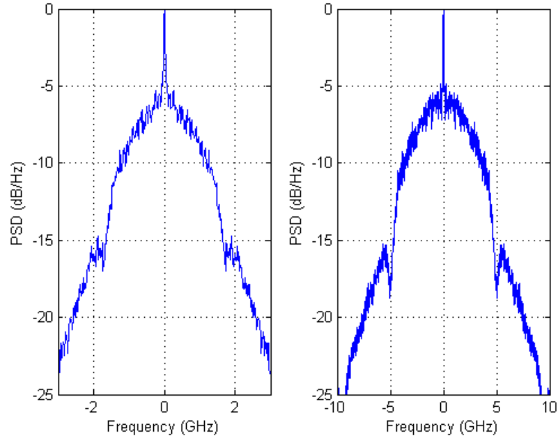
Figure 4.1.2: Power spectrum density of the exact time scaling Lorenz waveforms in the length T_c = 31ns .
