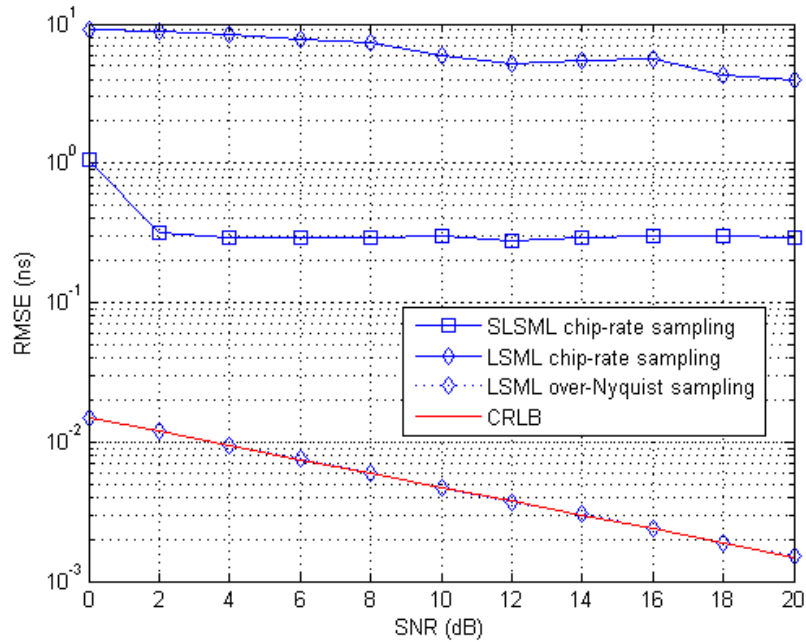
Figure 5.3.11: RMSE of SLSML algorithm as a function of SNR in an AWGN channel with T_a = 30ns .
