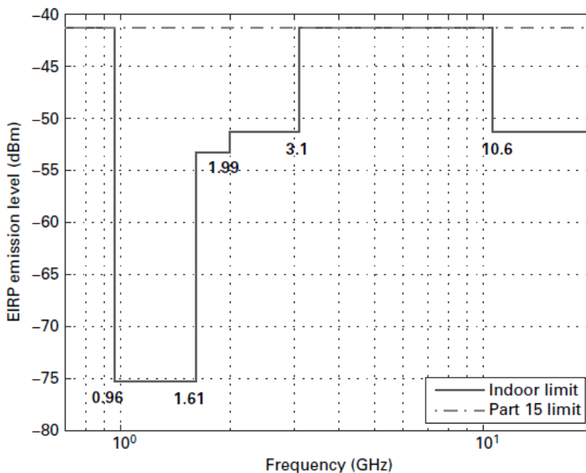
Figure 2.2.3: The FCC Emission limits for indoor UWB systems
