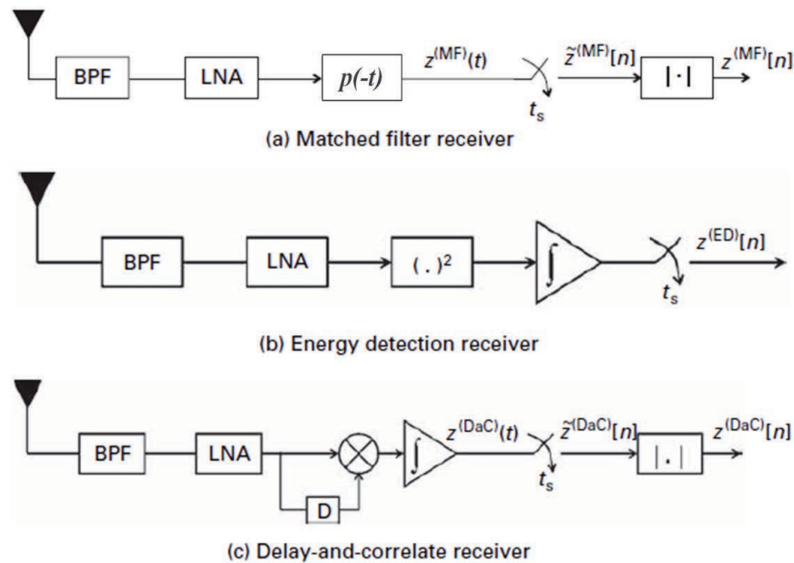
Figure 2.2.5: The different TOA estimator schemes (a). MF-based estimator (b). ED-based estimator (c). DAC-based estimator
