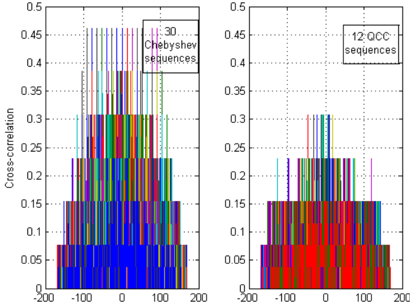
Figure 4.3.8: Cross-correlation function of selected Chebyshev sequences and QCC sequences with N_h = 13 .
