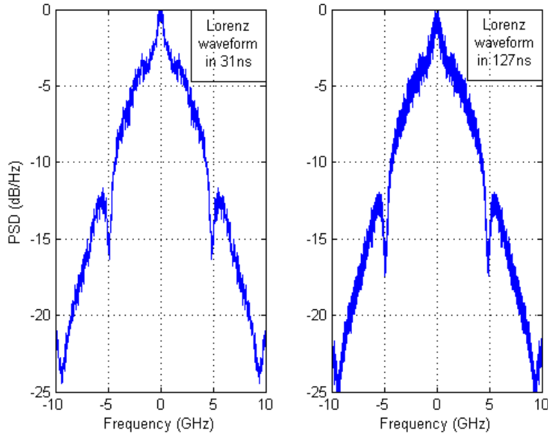
Figure 4.1.1: Power spectrum density of Lorenz waveforms with the same Lorenz parameters in the length T_c = 31ns and T_c = 127ns .
