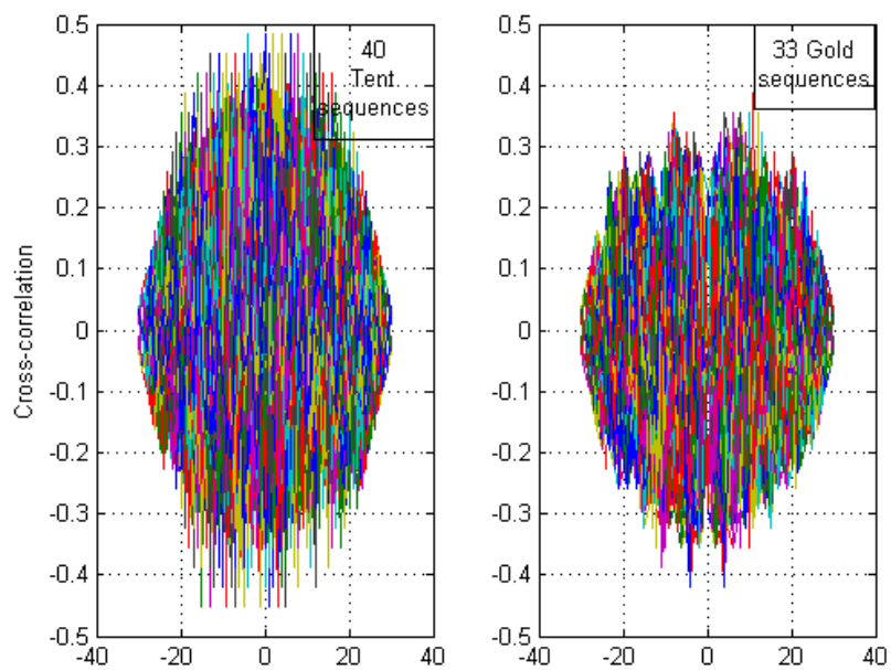
Figure 4.3.7: Cross-correlation function of selected Tent sequences and Gold sequences with N = 31 .
