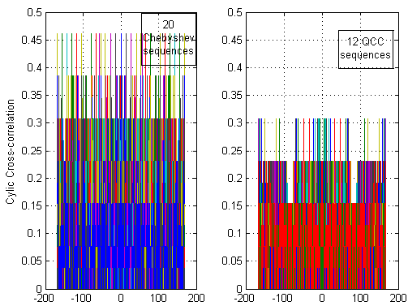
Figure 4.3.9: Cyclic cross-correlation function of selected Chebyshev sequences and QCC sequences with N_h = 13 .
