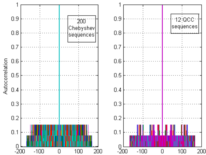
Figure 4.2.14: Autocorrelation function of selected Chebyshev sequences and QCC sequences with N_h = 13 .
