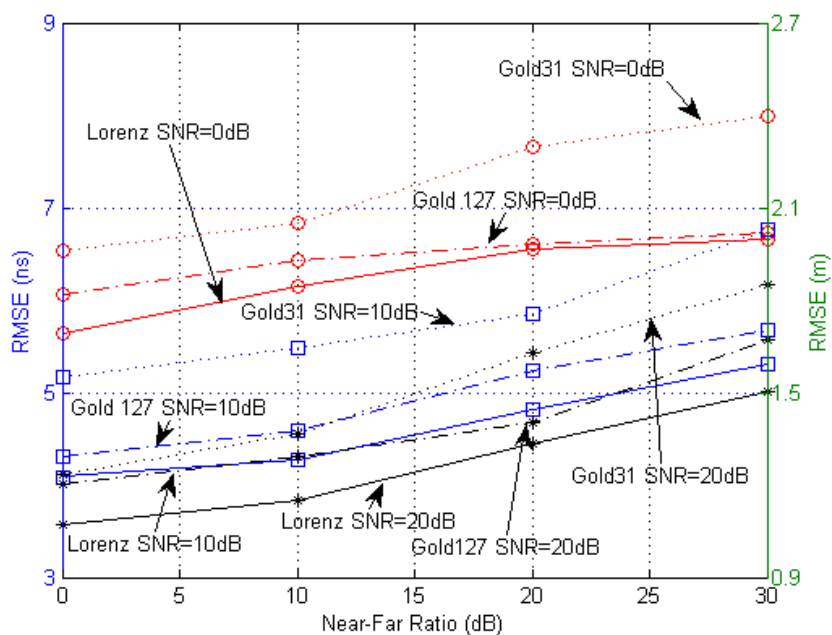
Figure 6.3.3: RMSE versus near-far ratio for different SNR values with M = 100 , T_s = 127ns , and K = 10 in CM1 channel.
