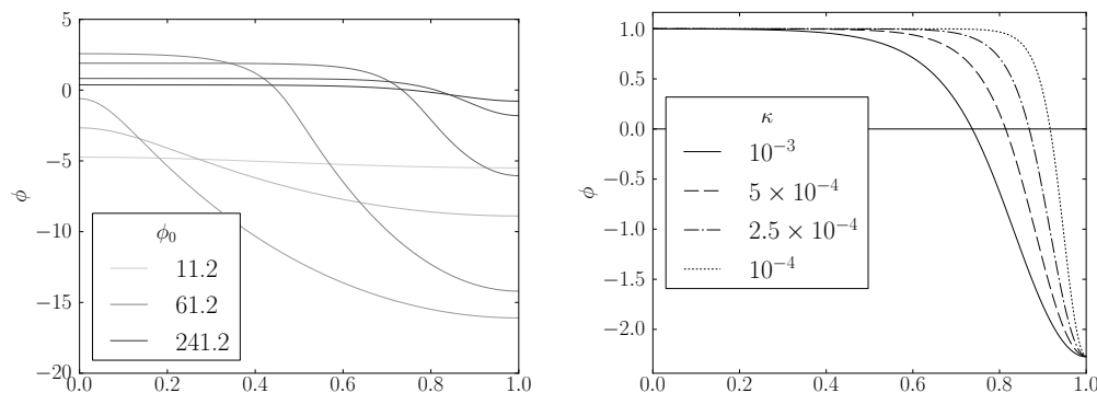
FIGURE V.3 : In the case of Model (I), d = 1 , \delta = 10^{-3} , we consider various profiles for x \mapsto \phi(x) with x \in (0, 1) = \Omega either (left) as \phi_0 varies and \kappa = 5 \times 10^{-4} , or (right) as \kappa varies, with \phi(0) = 1 .
