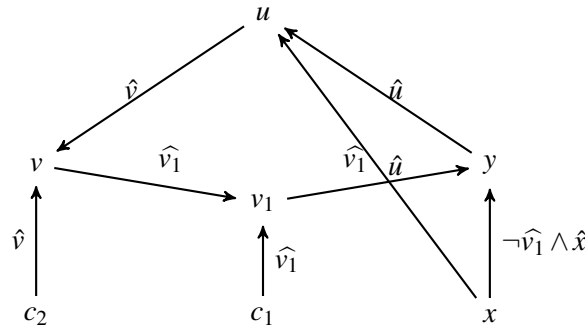
Fig. 5.9 The \text{SDDG}^+ of CycleDependency
