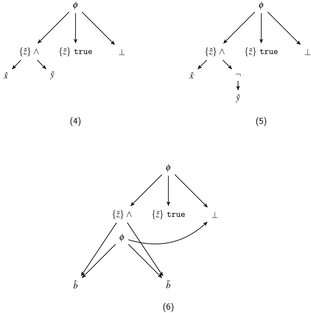
Fig. 6.20 The graphs of (4) z := x \wedge y , (5) z := x \neg y and (6) z := b when b
