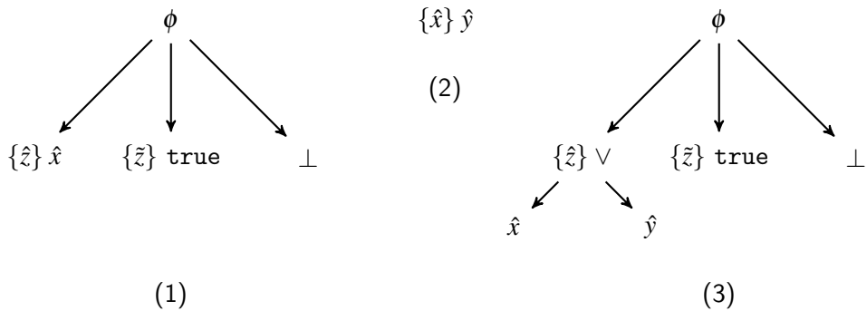
Fig. 6.19 The graphs of (1) z := \hat{x} , (2) x^{\hat{}} = y and (3) z := x^{\hat{}} + y
