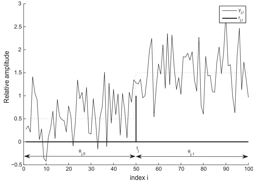
Fig. 1. Example of random experiment y_j and t_j for hypothesis H_1 .
