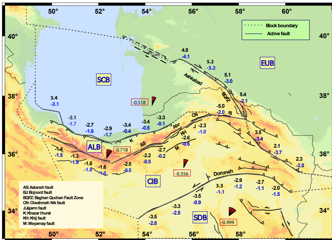
Figure 5.6 – Map showing slip rate variability (mm/yr) along the active faults from rigid block modeling. The upper values show the strike-slip component with (positive indicates right-lateral slip). The lower values indicate the fault-perpendicular slip rates (negative values indicate shortening). Dark gray lines represent active faults and dotted lines show block boundaries. The blocks are ALB: Alborz, CIB: Central Iran, EUB: Eurasian, SCB: South Caspian and SDB: South Doruneh blocks. Numbers inside the red rectangles are GPS block rotation rates in ^{\circ}/\text{Ma} , in the center of each block, calculated from block modeling with locked faults. Counter clockwise rotation sense is positive.
