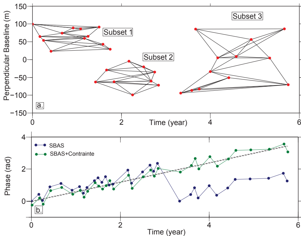
Figure 2.23 – a. Perpendicular baseline of three subsets synthetic interferograms used to compare the inversion methods developed by Bernardino et al. (2002) and Lopez-Quiroz et al. (2009). b. Temporal evolution of the pixel derived from the SBAS inversion method proposed by [Bernardino et al., 2002] and Lopez2009 (After [Jolivet, 2011])
