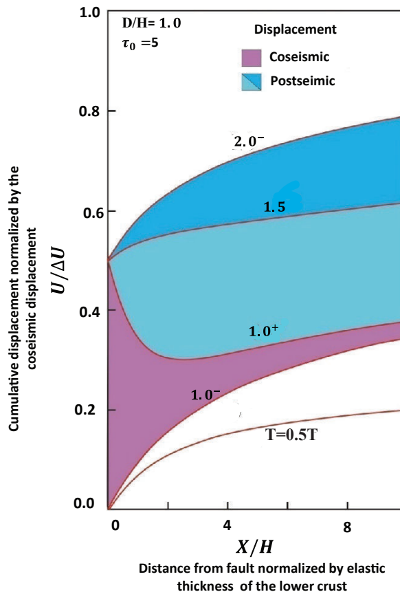
Figure 2.28 – Cumulated displacement with distance from the fault at different times in the earthquake cycle, after Courtesy M. Vergnolle.
