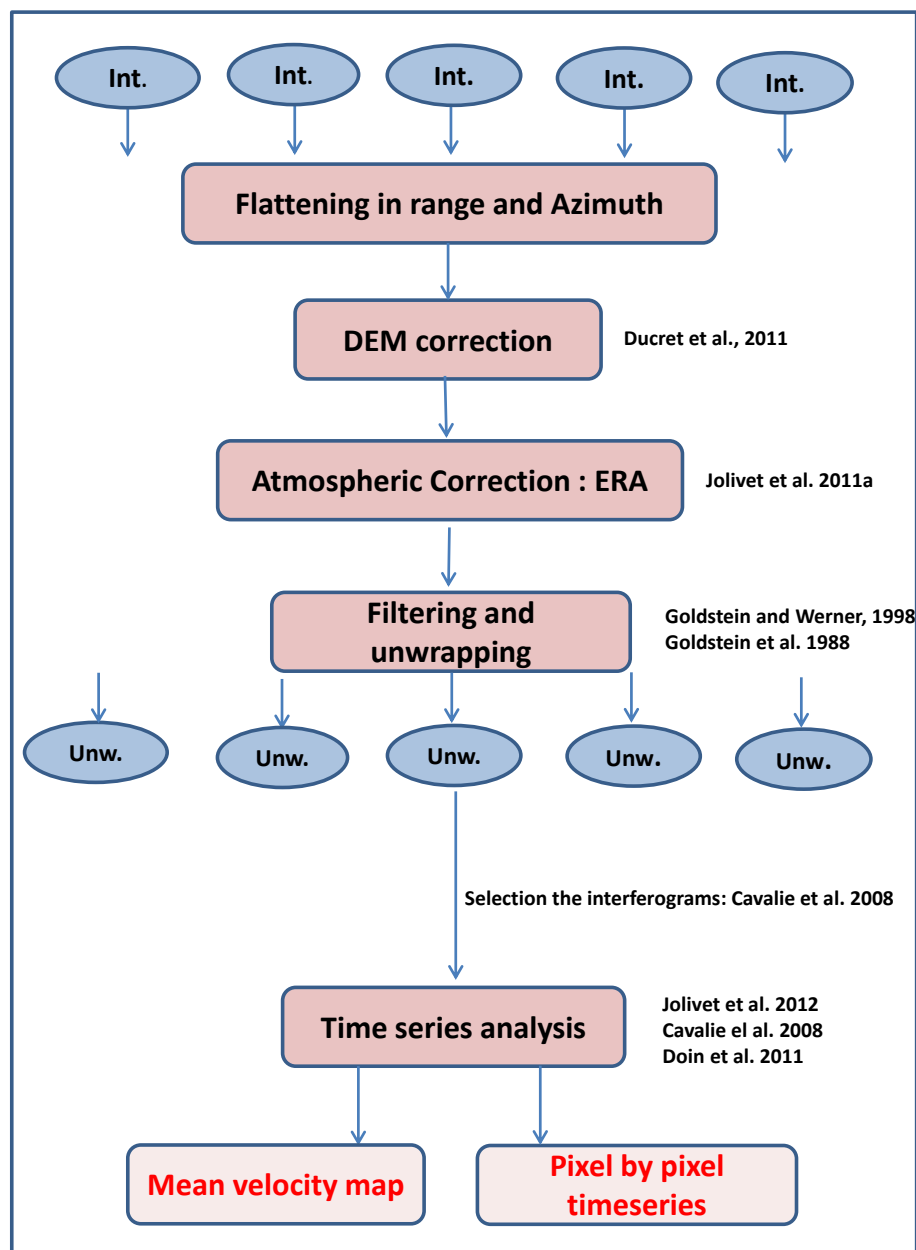
Figure 2.25 – The Schematic view of NSBAS chain processing strategy in this study.
