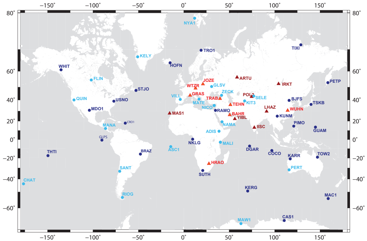
Figure 2.10 – The IGS stations which are used in Iranian daily solutions (triangles) and global daily solutions (circles) in this study. The stations with star are common in regional and global daily solution. The dark color symbols (dark blue circles and brown triangle) are the core stations for estimating the ITRF2008.
