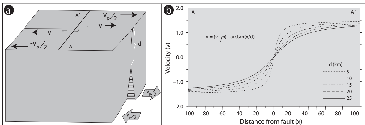
Figure 2.26 – A schematic illustration for elastic interseismic deformation around a plate-bounding, vertical strike-slip fault in a homogenous elastic medium: (a) Block diagram illustrating a right-lateral strike-slip fault locked from the Earth’s surface to a depth of d , below which it freely slips at a constant rate equal to the relative plate motion v_p (i.e., the far field velocity). (b) Profiles of fault parallel velocity along A-A' across the fault for various locking depths. Note the increase in the gradient of the profile around the fault with decreasing locking depth and the difference in the far field velocity on the two sides of the fault [Tatar et al., 2012].
