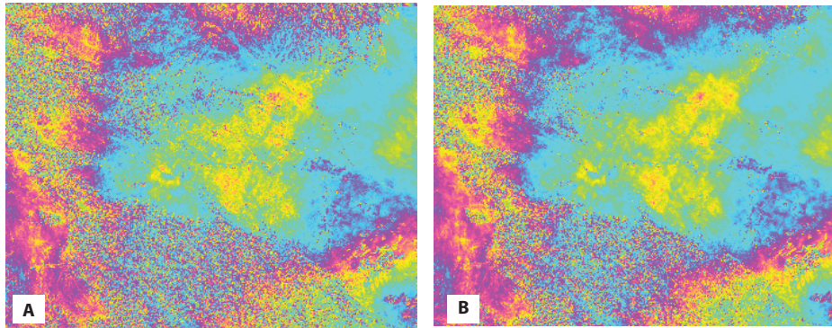
Figure 2.20 – A) The wrapped interferogram before DEM residual correction. B) The wrapped interferogram after DEM residual correction
