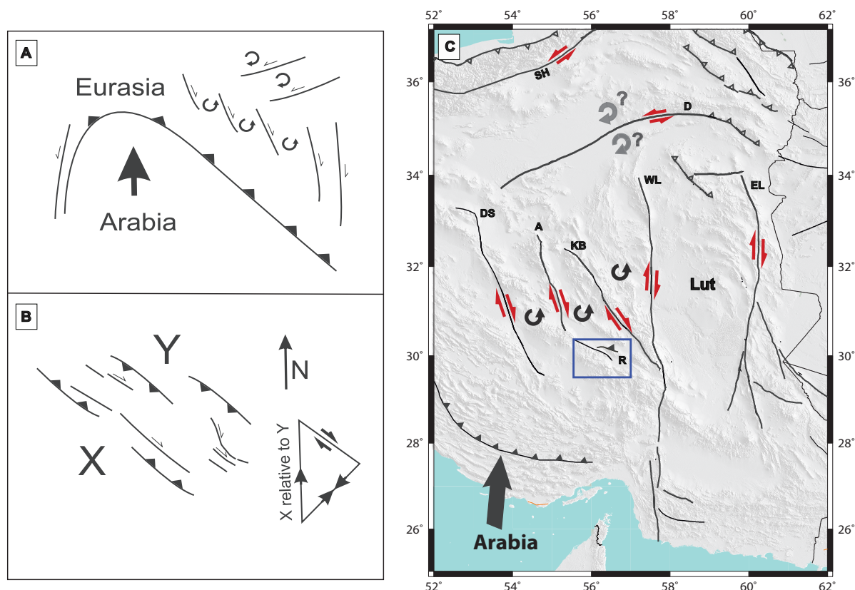
Figure 3.1 – Tectonic models for Central-Eastern Iran. A) The cartoon of the tectonic suggested by Allen et al., 2011 which described two possible models, vertical axis block rotation and indentation. Indentation tectonic results of the Arabian plate northwards motion can be achieved on NNW–SSE right-lateral strike-slip faults. B) Strain partitioning of north–south Arabian–Eurasian convergence via NE–SW shortening on NW–SE thrusts combined with right-lateral strike-slip on NW–SE trending faults. C) It presents the summary of the 3 possible models and simplified active faults. The vertical axis block rotation for right-lateral fault can be constraint by paleomagnetic data and the partitioning behavior may occur in NE–SW right-lateral faults such as Rafsanjan (blue rectangle). Figure A and B are from Allen et al., [2011] and abbreviations are: WL: West Lut fault, EL: East Lut fault, D: Doruneh fault, A: Anar fault, KB: Kuhbanan fault, DS: Dehshir fault, R: Rafsanjan fault and SH: Shahroud fault
