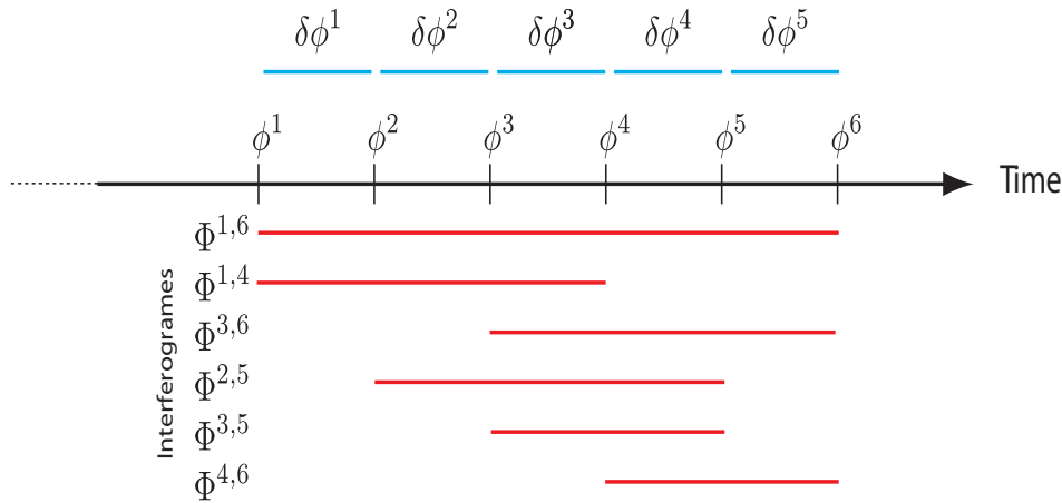
Figure 2.22 – Schematic representation of the inverse problem solution when analyzing time series. Each red line represents the temporal coverage of an interferogram \phi_{(i,j)} with acquisitions between i and j . The blue lines shows the phase increments ( \delta\phi_i and the time axe i present the evolution of the phase \phi_i from a reference phase \phi_1 . (After Jolivet [2011])
