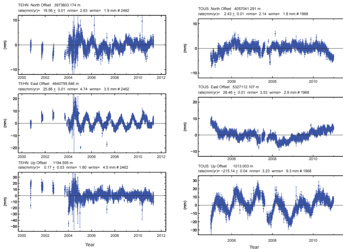
Figure 2.11 – De-trended position time series in NS, EW and UP components. A) 6 years (from 2005 to 2011) time series of TOUS station. B) 11 years (from 2000 to 2011) time series of TEHN station.
