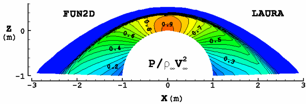
(b) Contours of the scaled pressure \bar{p} = \frac{p}{\rho_\infty V_\infty^2} .
