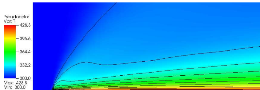
(a) Contours of temperature.
