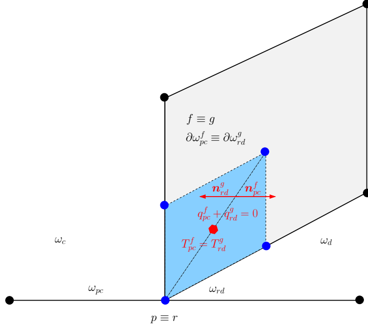
Figure 1.7: Continuity conditions for the sub-face fluxes and temperature on a sub-face shared by two sub-cells attached to the same point. Fragment of a polyhedral grid: quadrilateral face shared by hexahedral cells c and d . Labels p and r denote the indices of the same point relatively to the local numbering of points in cell c and d . The neighboring sub-cells are denoted by \omega_{pc} and \omega_{rd} . They share the sub-face \partial\omega_{pc}^f \equiv \partial\omega_{rd}^g , which has been colored in blue.
