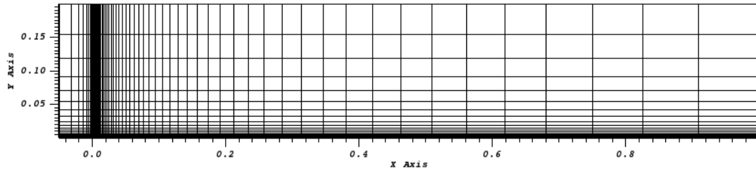
(a) Presentation of the mesh. 50 \times 30 structured mesh. 50 cells along the plate and 30 cells perpendicular to the plate.
