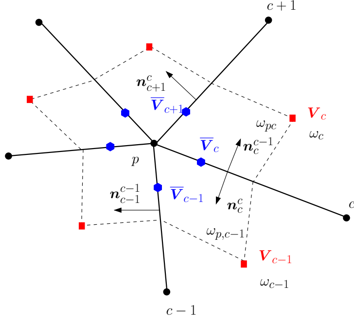
Figure 2.5: Notations employed around a point.
