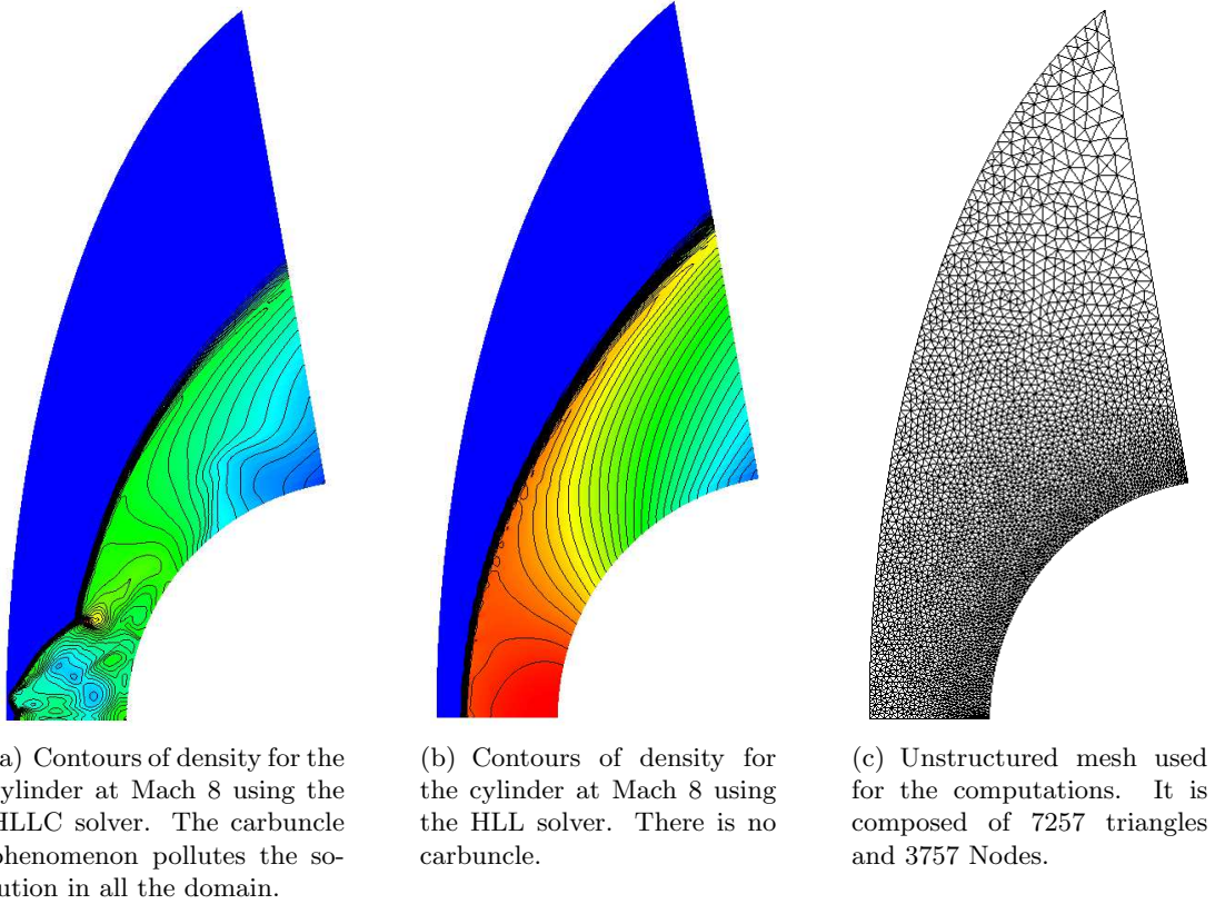
Figure 3.5: Carbuncle around a cylinder at Mach 8
