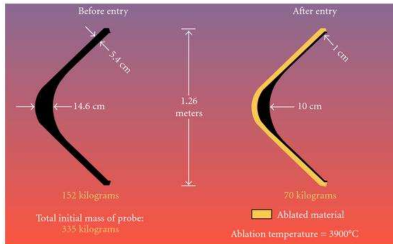
Figure 8: Galileo probe heat shield ablation : taken from www.nasaimages.org .
