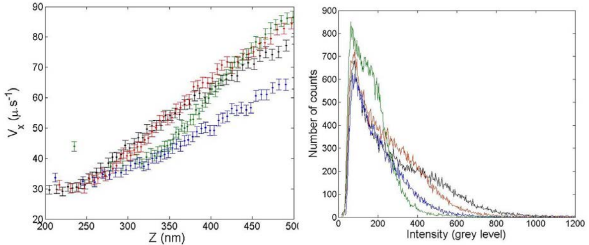
Figure 2.19: Velocity profile (left) and intensity distribution (right) corresponding to different focusing position during experiments (left), correctly focused (black), +200 nm (red), +400 nm (green), -200 nm (blue).
