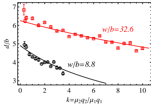
FIG. 9: The diameter of the droplets, d/b , produced by step-emulsification in the HS cells with two aspect ratios: w/b = 8.8 (black circles) and w/b = 32.6 (red squares). The solid lines are the prediction in Eq. (17) multiplied by 1.85 and 2.15 respectively.
