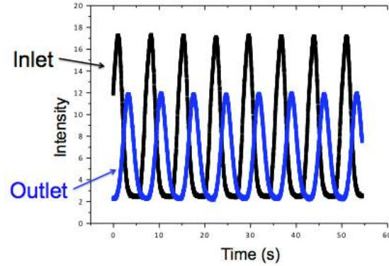
Figure 2.8: At the entry and the outlet of the micro system, intensity measurements are carried out, detecting blobs of fluorescent particles injected in the micro model (black) and going out of it (blue). The injection impulsion is short, so that there is no plateau visible on the diagram. The intensity at the outlet is lower than that at the entry, because dilution of water or brine.
