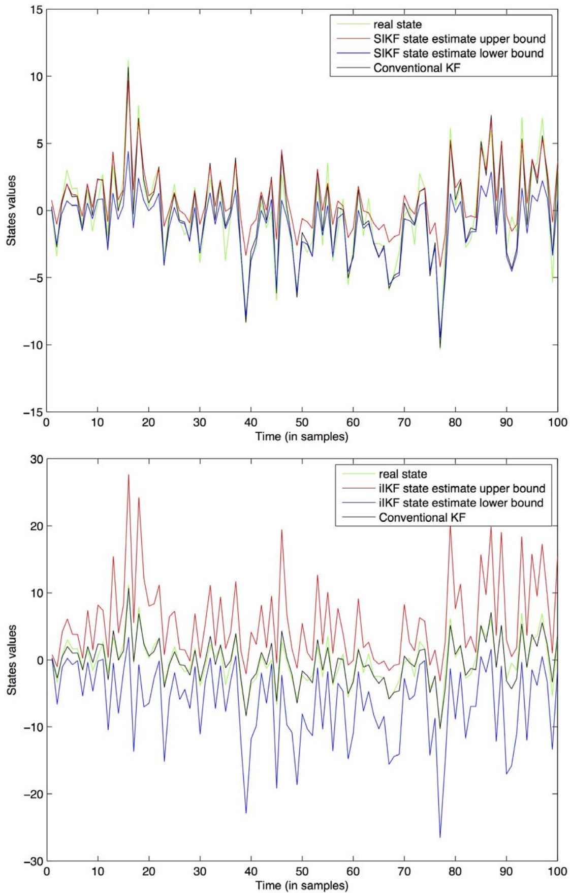
Figure 3.7: Simulation results from sIKF (up) / Simulation results from iIKF with \epsilon = 0.05 (down).
