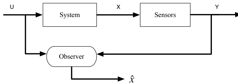
Figure 1.2: State observer structure
