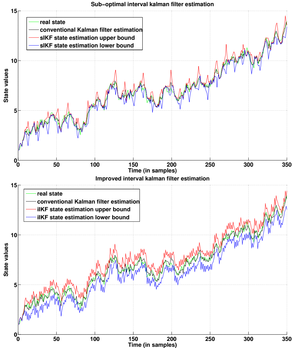
Figure 3.5: Result of estimation from sIKF (up) / Result of estimation from iIKF (down).
