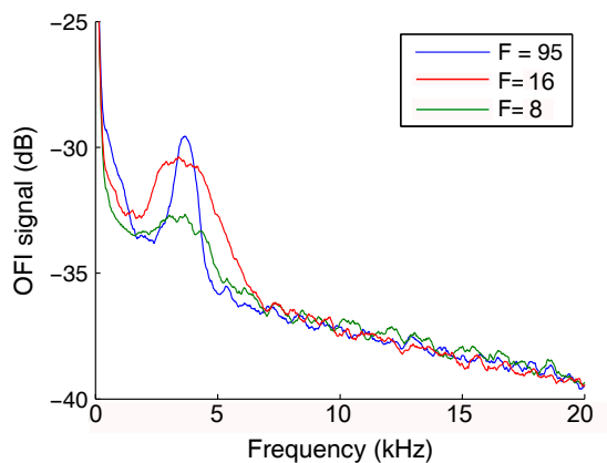
Figure III.20: OFI spectra for various optical set-ups (single lens scheme).
