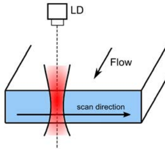
Figure IV.20: OFI sensing scheme in the 20 \mu\text{m} \times 100 \mu\text{m} flowchannel
