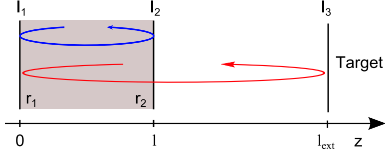
Figure II.2: Schematic arrangement for a LD under optical feedback, known as the three-mirrors cavity configuration.
