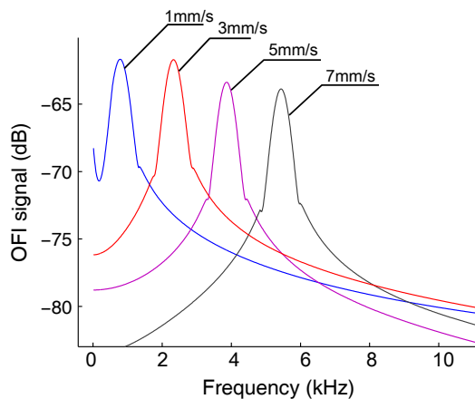
Figure III.6: Simulated OFI spectrum for various measured velocities V_{\max} [1, 3, 5, 7] mm/s. The sensing volume is small compared to the flowchannel's radius. The Doppler peak is proportional to the velocity value
