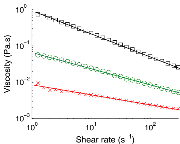
Figure IV.12: Experimental rheograms for various concentrations of xanthan gum (0.25 (cross) 1 (circle) and 3 g/L (square)). The viscosity of each solution as a function of the shear rate applied are plotted in logarithm scale.
