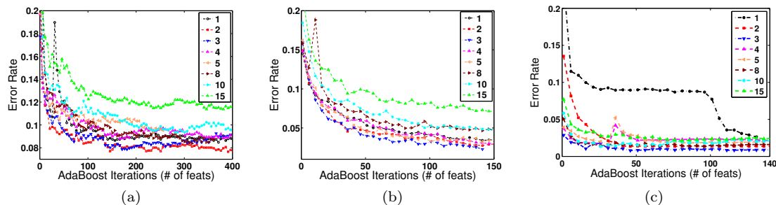
Figure 4.8: Decision tree depth validation for (a) Haar like features, (b) EOH features, and (c) CS-LBP features.
