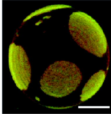
Figure 1.20 – Confocal fluorescence microscopy in ternary mixture DOPC/DPPC/Chol in which fluid-ordered/fluid-disordered (round domains) phases coexist [23].
