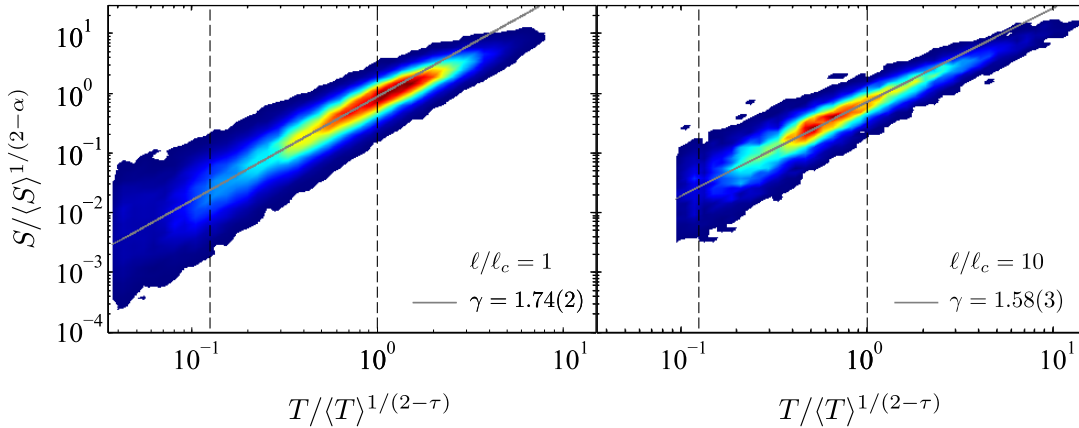
FIGURE 6.19: Probability density plots of the joint distribution of rescaled variables S^* and T^* for l/\ell_c = 1 (left) and 10 (right). Vertical dashed lines show the scaling regime chosen to extract the power-law exponent \gamma . The solid straight lines are the best fits S^* \sim (T^*)^\gamma (statistical error of the fit quoted in the figure). The probability density of points increases from blue to red.
