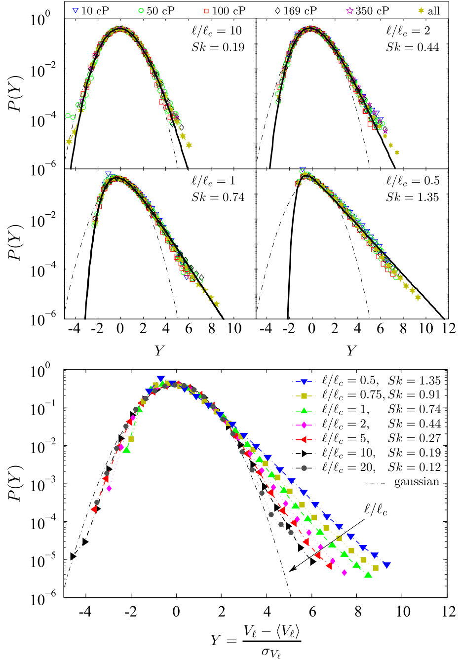
FIGURE 6.4: Statistical distributions of the normalized global velocity Y = (V_\ell(t) - \langle V_\ell \rangle) / \sigma_{V_\ell} for various values of l/l_c . Top panels show P(Y) for all the experiments with different (\mu, \nu) compatible with l/l_c = 10, 2, 1, and 0.5 . Distributions for each experiment separately, and for data sets containing data from all experiments are shown. Solid lines correspond to Generalized Gumbel distributions with the value of Sk of the experimental distributions. The bottom panel displays P(Y) for data sets containing data from all experiments compatible with l/l_c from 0.5 to 20 . Dashed-dotted lines in all plots correspond to the normal distribution.
