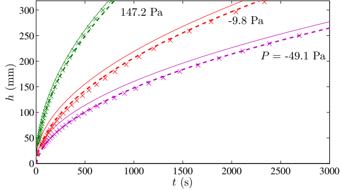
FIGURE 3.5: Mean position of the imbibition fronts vs time, measured in displacements in the D^* cell in the absence of gravity (horizontal cell) at different imposed pressures. Experimental results are represented by crosses, and compared to LW predictions (solid lines) and to our own prediction (3.6) that accounts for viscous dissipation in the preparation zone (dashed lines).
