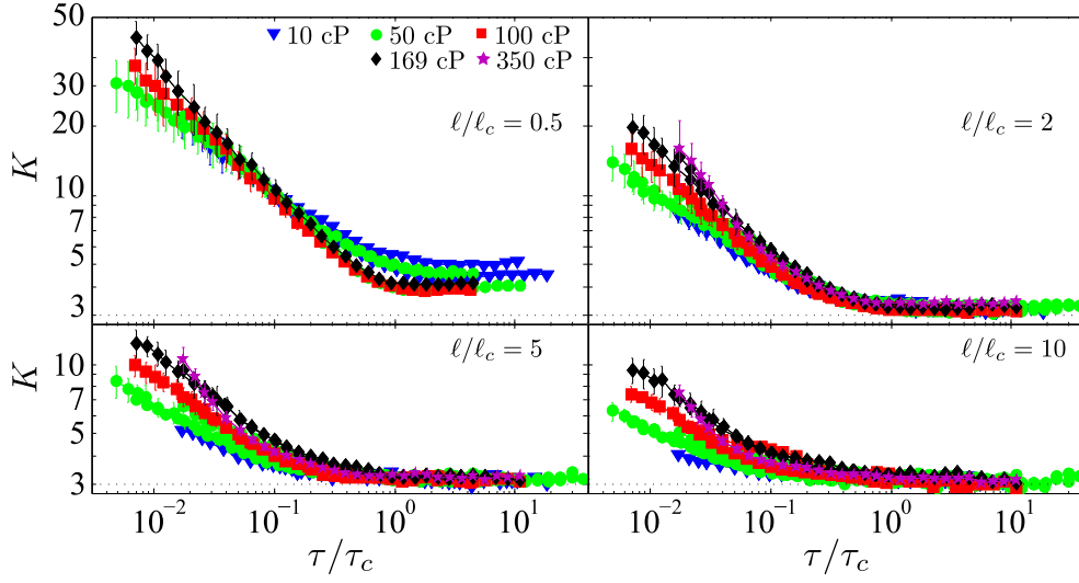
FIGURE 7.11: Double-logarithmic plots of the kurtosis corresponding to all experiments compatible with \ell/\ell_c = 0.5, 2, 5, 10 as functions of the rescaled \tau/\tau_c . Different symbols correspond to different viscosities –different velocities ranging from 0.036 < v < 0.55 mm/s are not distinguishable.
