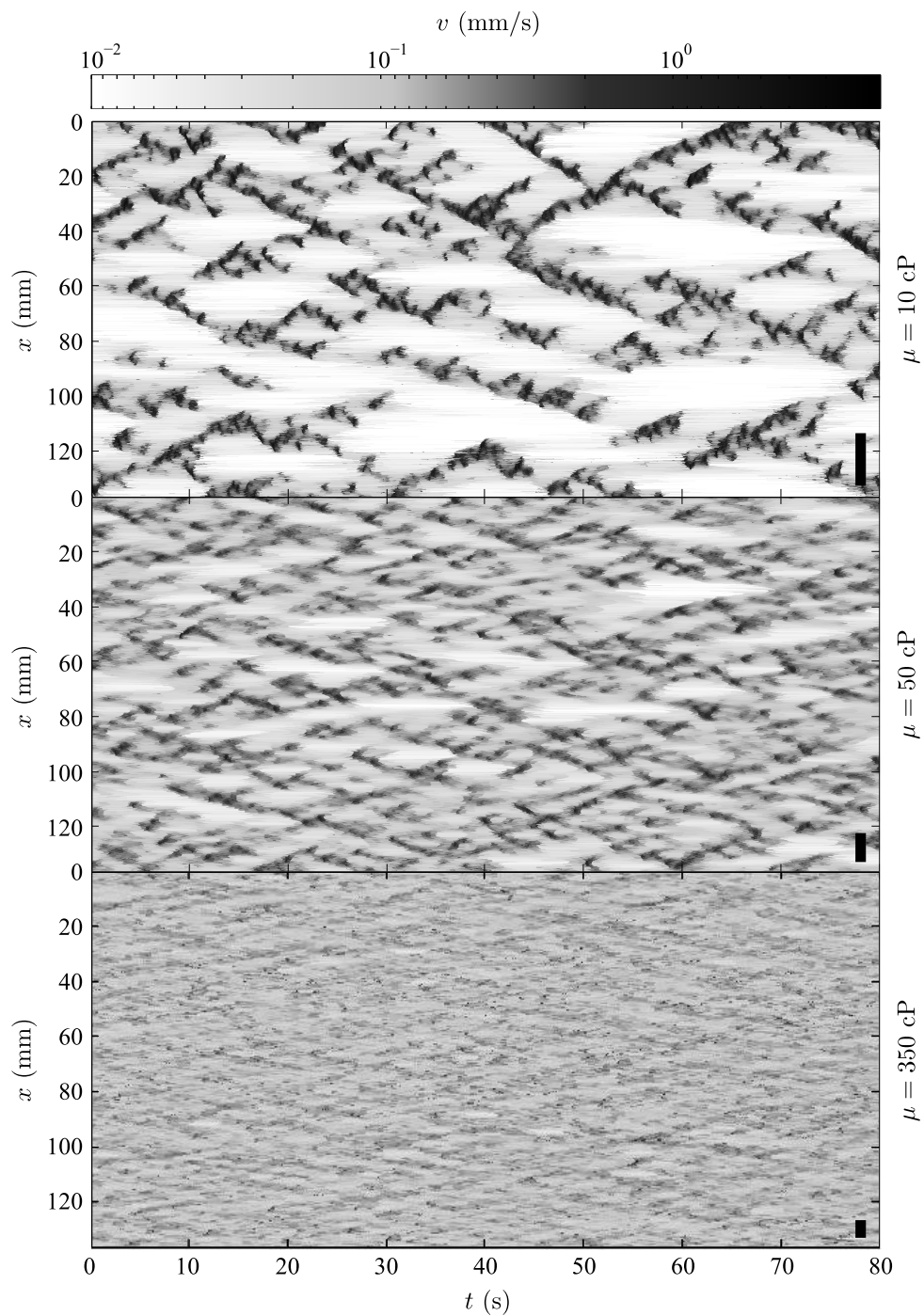
FIGURE 5.3: Spatio-temporal (activity) maps of the same three experiments shown in Fig. 5.2. v = 0.13 mm/s in all cases but \mu = 10, 50, 350 cP (top, middle, bottom). The greyscale for v(x, y) is the same in all cases. The bottom-right black vertical line gives the nominal correlation length \ell_c = 15.3, 6.7, 2.6 mm for each experimental condition.
