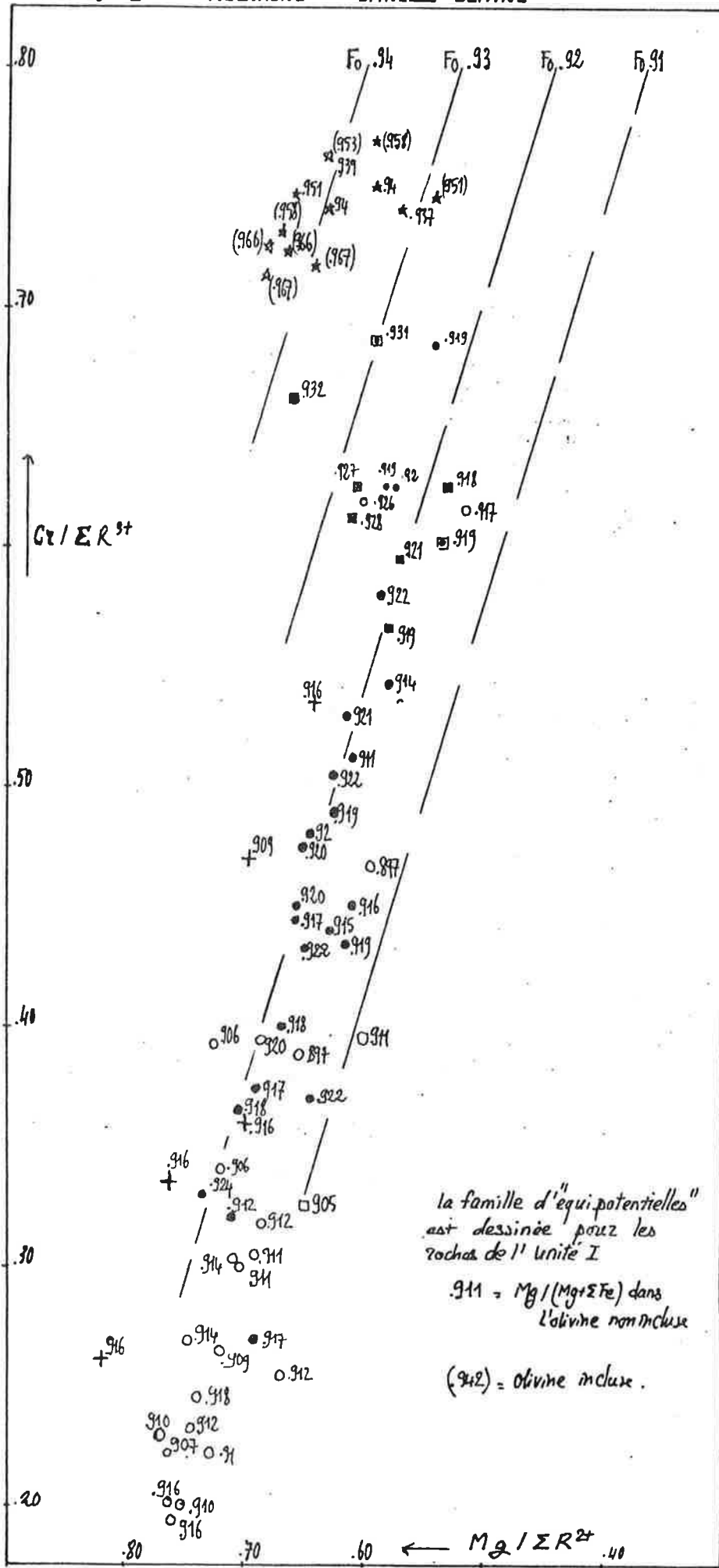
Fig. 65 - RELATIONS SPINELLE-OLIVINE
