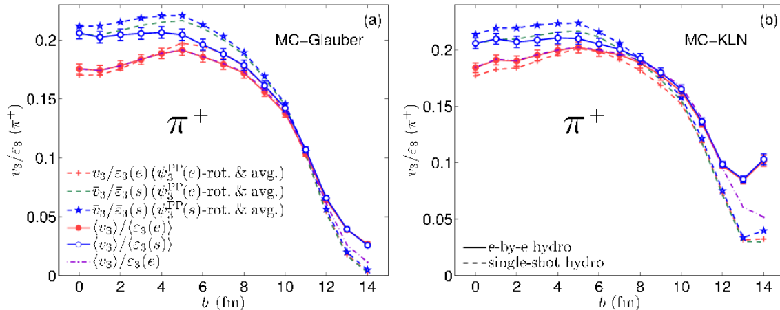
Figure 4.4: v_3/\varepsilon_3 dependence on impact parameter for pions. Solid lines correspond to event-by-event hydrodynamics, dashed lines correspond to single-shot hydrodynamics. Left: for MC Glauber initial state model, right: MC-KLN initial state model [18].
