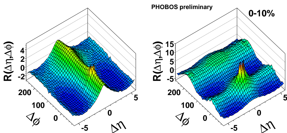
Figure 1.17: Two-particle correlations for pp ( 200 GeV) and AuAu ( 200 GeV) collisions at RHIC [11].
