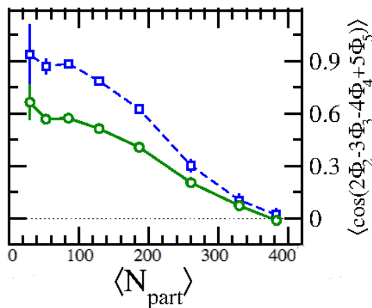
Figure 5.8: Prediction of \langle \cos(2\Phi_2 - 3\Phi_3 - 4\Phi_4 + 5\Phi_5) \rangle(N_{part}) from the AMPT model, from [20] (blue squares: calculations made with SP method, green circles: calculations made with EP method)
