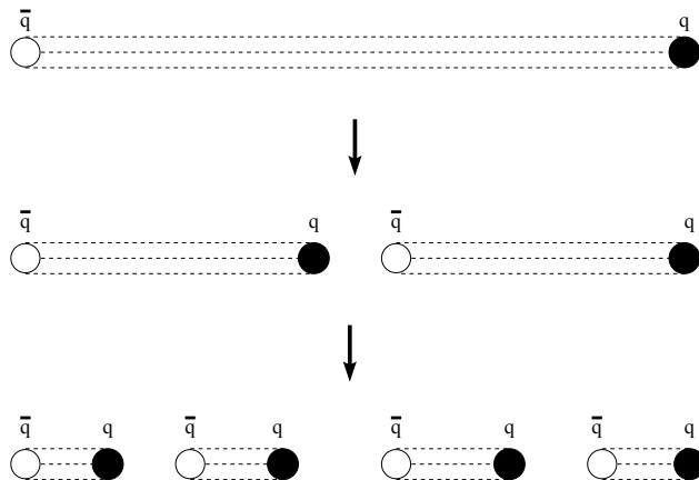
Figure 1.5: Schematic picture of the confinement. The pair q\bar{q} stretches the string and breaks into two pairs of q\bar{q} [2].
