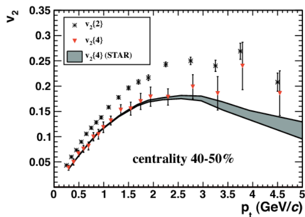
Figure 1.15: v_2(p_t) by ALICE collaboration compared [72], 40–50% centrality range.
