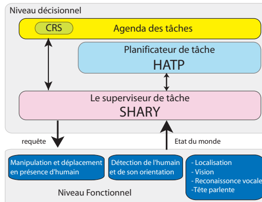
FIGURE 6.11 – Architecture logicielle
