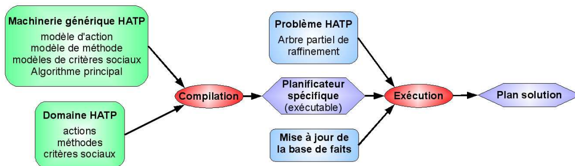
FIGURE 6.1 – Principe de compilation de HATP
