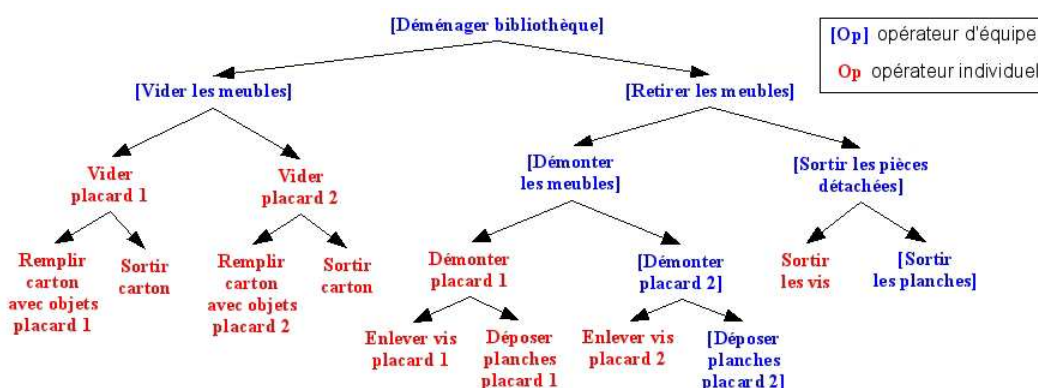
FIGURE 2.4 – Exemple de Team Oriented Plan.
