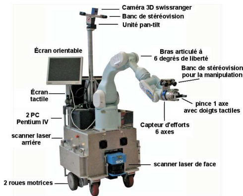
FIGURE 6.10 – Le robot Jido
