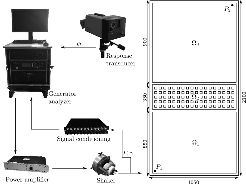
Figure 4.1: Layout of FRF measurement system. P_1 is the force input position, while P_2 used for a representative single-point transfer mobility measurement.
