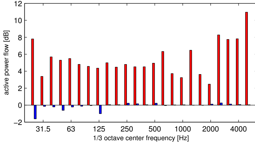
Figure 4.9: 1/3 octave band averaged and time averaged real power flow into the plate: (red) control on case 1; (blue) control on case 2.
