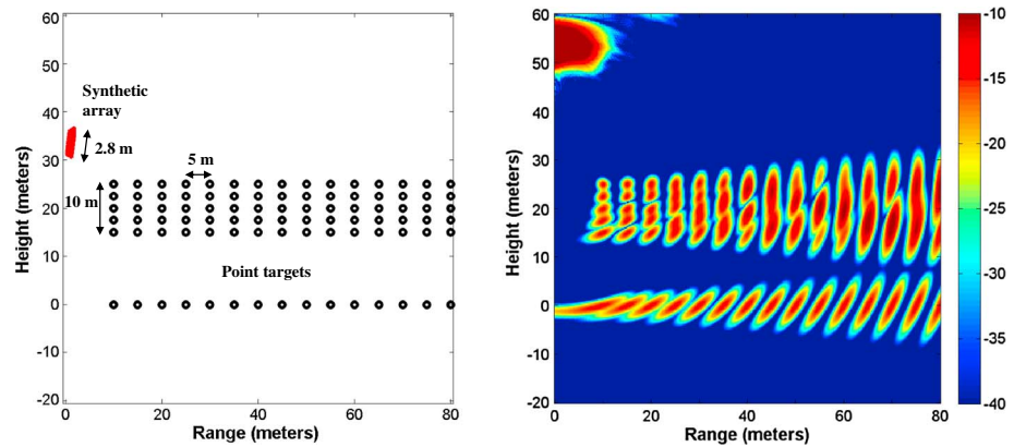
Figure 4. (left) Description of a 25 m high forest simulated with point targets uniformly distributed and (right) the tomogram obtained with the simulated raw data.
