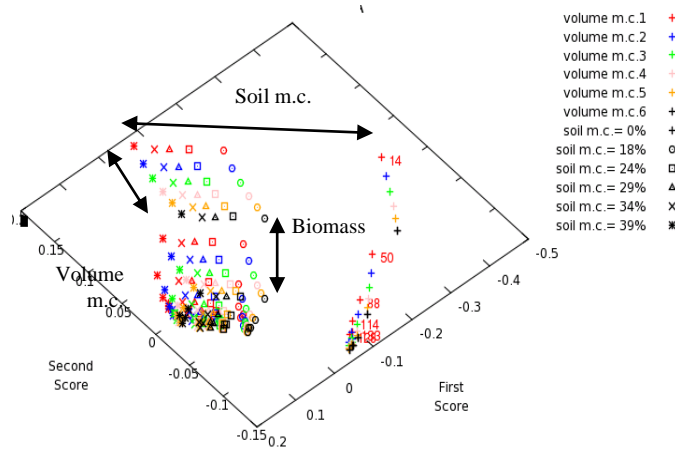
Fig. 11. Result of a PCA on radar HH, HV, VV radiometry and optical NINSOL index for forest without leaves.
