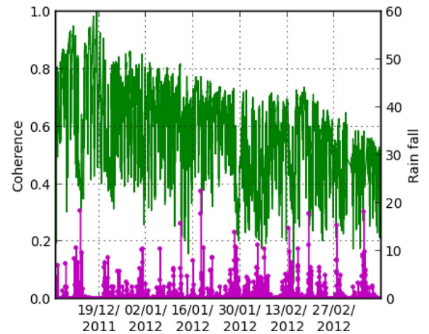
Fig. 8. Temporal coherence for HV polarization over three months (full forest during the rainy season). The x -axis corresponds to the time. Rainfall (mm) is in purple.
