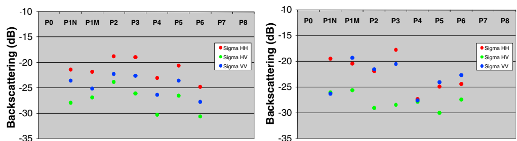
Figure 12. (left and right) Polarimetric relative energy backscattered by the volume and the soil, respectively, for all sites.
