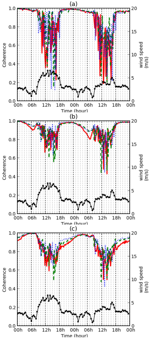
Fig. 2: Temporal variation of the coherence during the dry period (a) for the „volume only’ computed with the reference for the coherence computation taken the first day at midnight, (b) for the „full forest’ computed with a reference at midnight and (c) for the „full forest’ computed with a reference at 6:00 AM. The red full curve corresponds to the polarization HH, the blue dotted one to VV and the green dashed one to HV. The thick black curve represents the wind speed. The temporal baseline is the time minus the reference time of the first day.
