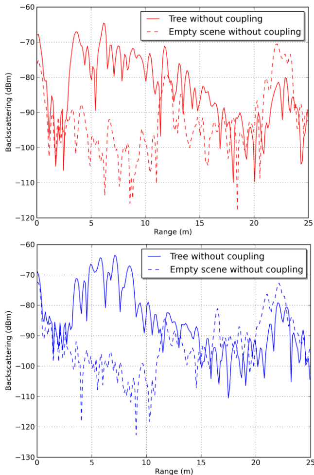
Fig. 4. Impulse response of the scene with and without the tree, with subtraction of the sky measurement, for polarization HH (top) and VV (bottom).
