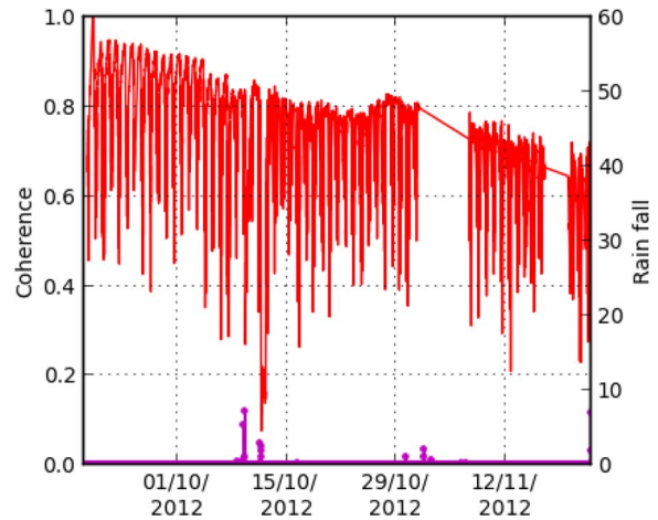
Fig. 11. Temporal coherence for HH over two months (full forest during the dry season). The x -axis corresponds to the time. Rainfall (mm) is in purple.
