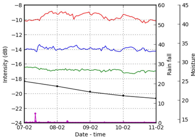
Fig. 16. Time series of the backscattering coefficient computed over the full forest (zoom of Fig. 15). The red curve corresponds to HH polarization, the blue curve to VV, and the green to HV. The black curve corresponds to the soil moisture at 10-cm depth, and the purple one corresponds to the rainfall (mm).
