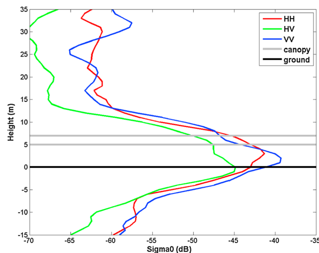
Figure 10. Polarimetric backscattering profiles for P7. The black solid line corresponds to the soil location, and the gray solid lines correspond to the measured height of the canopy.
