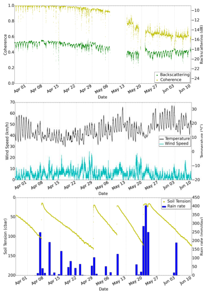
Fig. 9. RCS and coherence (top), temperature and wind speed (middle), Soil tension and rain rate (bottom) for TS-SPRING.
