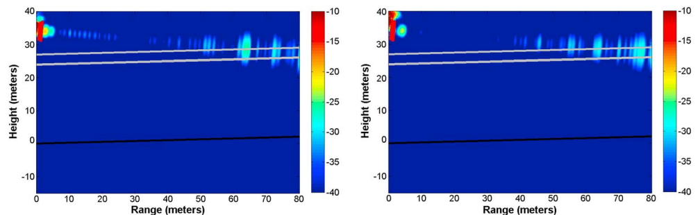
Figure 5. Tomograms made from sky measurements to determine the effect of SWR in (left) HH and (right) VV polarizations. The black line is located at the ground and the gray ones at the highest possible height for the canopy.
