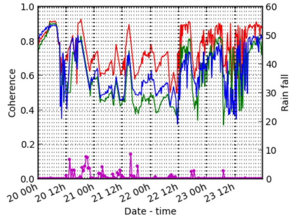
Fig. 10. Temporal coherence over four days during a rainy period (full forest in the rainy season). HH, VV, and HV are in red, blue, and green in the upper curves, and rainfall (mm) is in the bottom.
