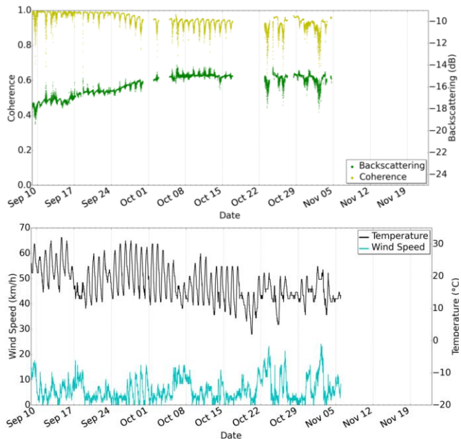
Fig. 7. RCS and coherence (top) and temperature and wind speed (bottom) for TS-AUTUMN.
