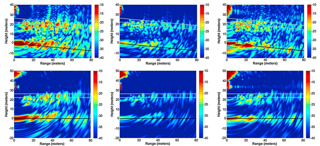
Figure 8. Vertical tomogram for (left) HH, (middle) HV, and (right) VV reconstructed with the measurements performed on P1M. (top) Initial images and (bottom) images with slope correction and apodization. The black line corresponds to the soil location, and the gray lines correspond to the measured minimum and maximum height of the canopy.
