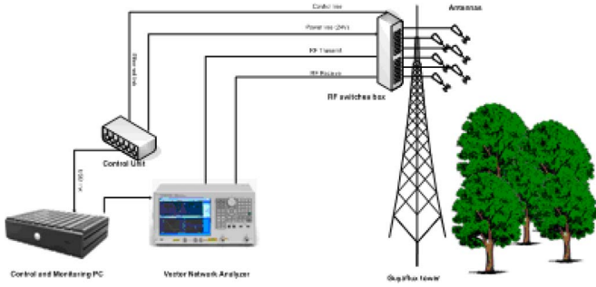
Fig. 1. TropiSCAT instrument architecture.
