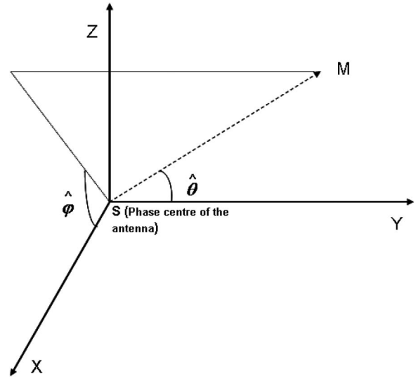
Fig. 3. Coordinate system of the antenna.
