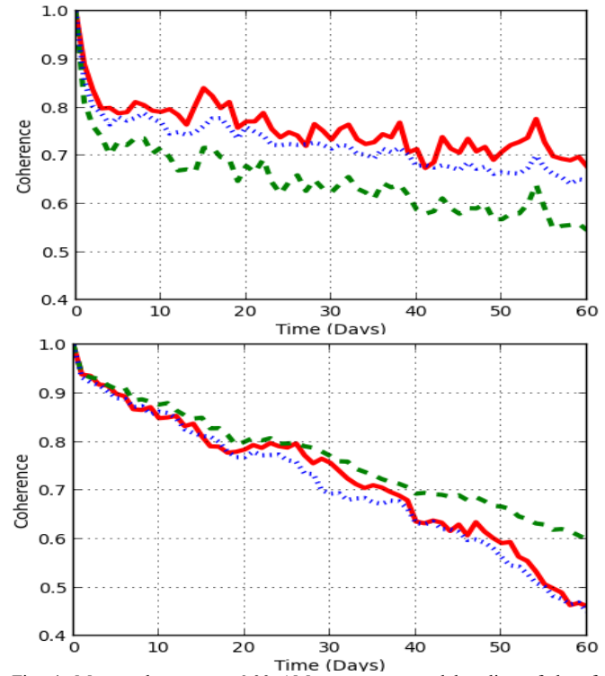
Fig. 4: Mean coherence at 6:00 AM versus temporal baseline of the „full forest’ for the HH (red-full), HV (green-dashed) and VV (blue-dotted) polarizations during the rainy period (top) and during the dry period (bottom), averaged over 30 days.
