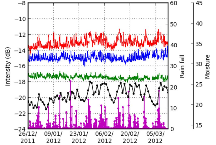
Fig. 14. Time series of the Backscattering coefficient computed over the canopy ("volume only") during the rainy period. The red curve corresponds to the HH polarization, the blue to the VV, and the green to the HV one. The black curve corresponds to the soil moisture (%) at 10-cm depth, and the purple one corresponds to the rainfall (mm).
