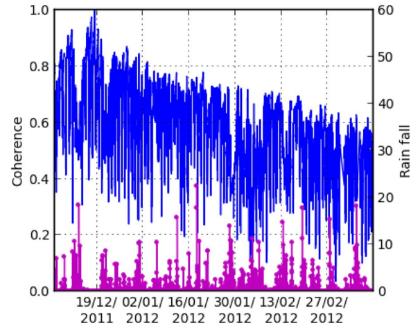
Fig. 7. Temporal coherence for VV polarization over three months (full forest during the rainy season). The x -axis corresponds to the time. Rainfall (mm) is in purple.
