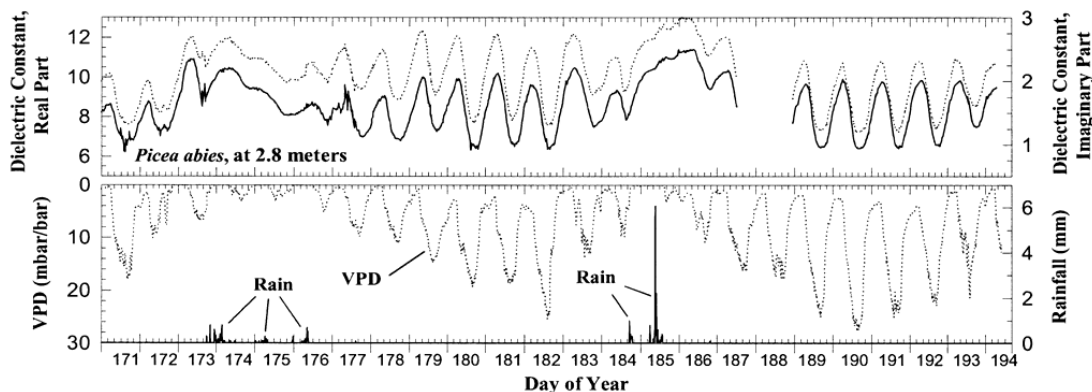
Fig. 12. Plot of \text{Re}(\epsilon_r) and \text{Im}(\epsilon_r) at P-band for a Norway spruce ( Picea Abies ) at 2.8 m height and concurrent Vapor Pressure Deficit (VPD) and rainfall (millimeters of rainfall in 10-min intervals) plotted for time periods extending over a total of 23 days of 1995. As the VPD and dielectric constant tend to be negatively correlated, VPD is plotted with the zero reference placed at the top of the y axis to allow easier comparison with dielectric variability. VPD (mbar/bar) is the measured vapor pressure deficit (in mbar) normalized to standard atmospheric conditions at sea level (1013 mbar) - Reprint from [15].
