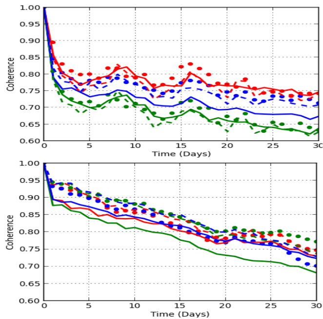
Fig. 6: Mean coherence versus temporal baseline of the „full forest” for the HH (red), HV (green) and VV (blue) polarizations. Top: during the rainy period. Bottom: during the dry period. Full circle: time observation at 6:00 AM, full curve: time observation at 6:00 PM and dashed curve: time observation at midnight.
