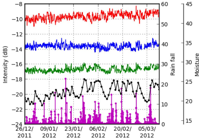
Fig. 15. Time series of the backscattering coefficient computed over the full forest during the rainy period. The red curve corresponds to the HH polarization, the blue to the VV, and the green to the HV one. The black curve corresponds to the soil moisture (%) at 10-cm depth, and the purple one corresponds to the rainfall (mm).
