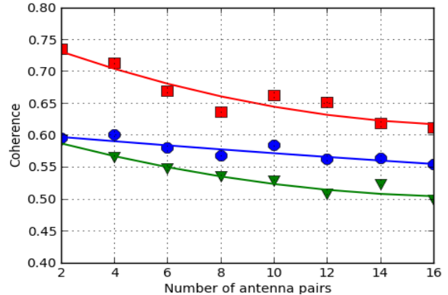
Fig. 1: Average coherence versus the number of antenna pairs for the HH (red-square), HV (green-triangle) and VV (blue-circle) polarization.
