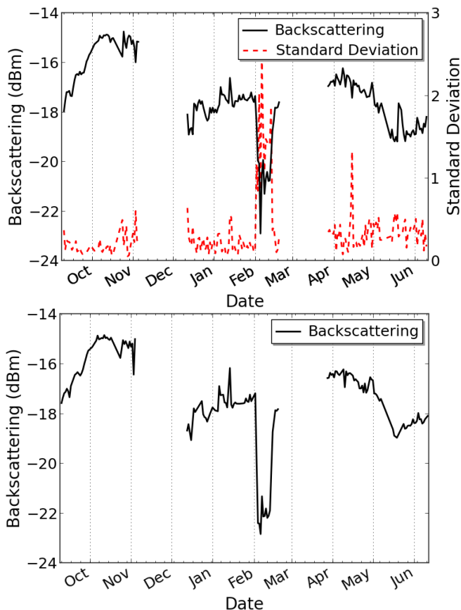
Fig. 13. Daily average RCS (top) and average RCS of the tree between 6:30 and 7:30 a.m. (bottom), for the three periods.
