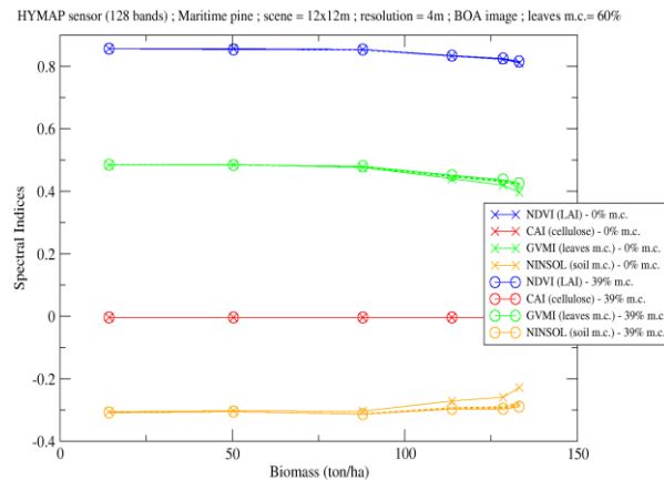
FIG. 10 SENSITIVITY OF SPECTRAL INDICES FOR SEVERAL BIOMASS AND SOIL MOISTURE CONTENT.
