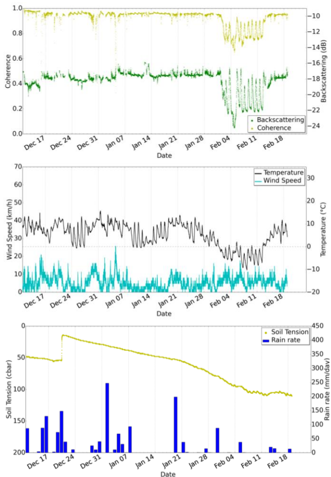
Fig. 8. RCS and coherence (top), temperature and wind speed (middle), Soil tension and rain rate (bottom) for TS-FALL.
