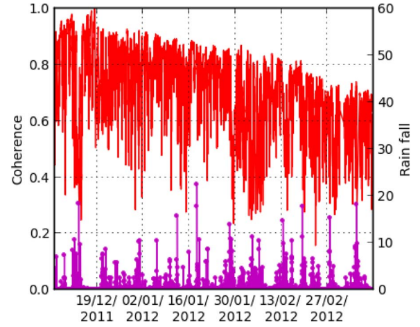
Fig. 6. Temporal coherence for HH polarization over three months (full forest during the rainy season). The x -axis corresponds to the time. Rainfall (mm) is in purple.
