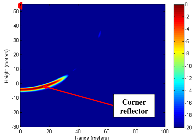
Fig. 5. Tomographic HH response for a trihedral reflector.
