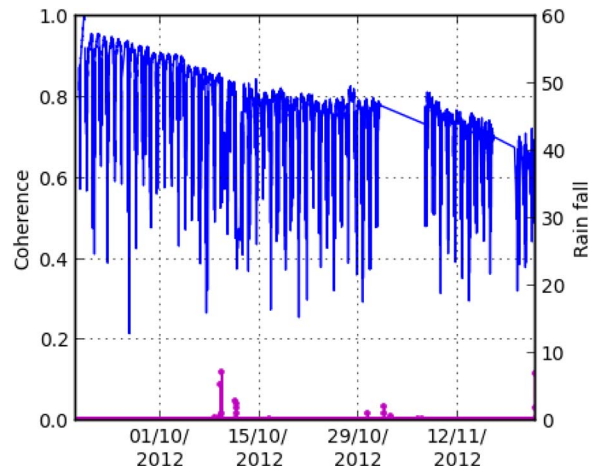
Fig. 12. Temporal coherence for VV over two months (full forest during the dry season). The x -axis corresponds to the time. Rainfall (mm) is in purple.
