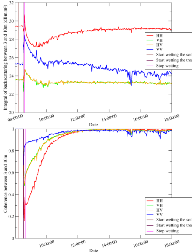
Fig. 6. Evolution of polarimetric RCS (top) and coherence (bottom) of the canopy (3 - 10 m range) for STS after the watering of the tree. Water was continuously project on the whole tree between the brown and the pink vertical lines.
