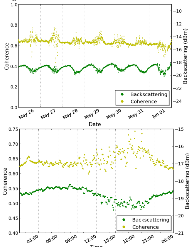
Fig. 11. Focus of RCS and coherence for a week without rain of TS-SPRING (top), with zoom on May the 29th (bottom).
