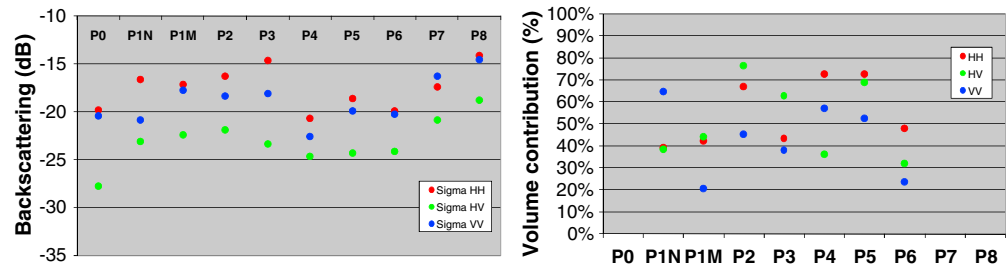
Figure 13. (left) Polarimetric energy backscattered by the total scene and (right) the share in percentage of the volume energy upon the total response.
