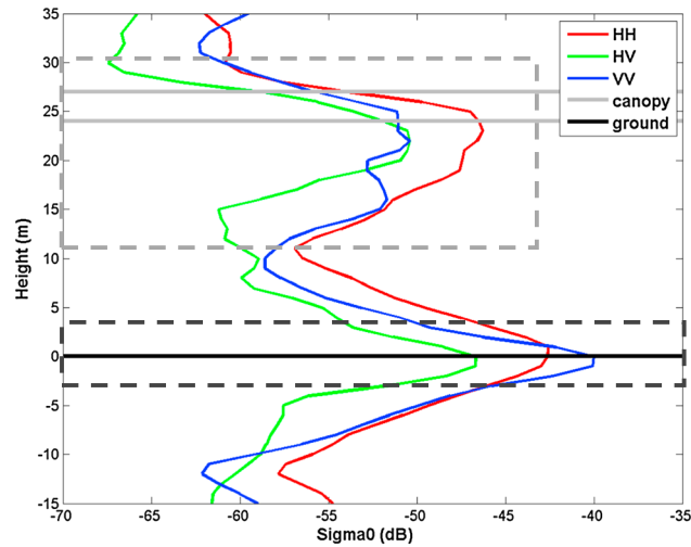
Figure 9. Polarimetric backscattering profiles for P1M. The black solid line corresponds to the soil location, and the gray solid lines correspond to the minimum and maximum measured height of the canopy. The dotted lines show the vertical limits of the integration for the computation of backscattered energy by the volume and by the soil, respectively, in gray and black.
