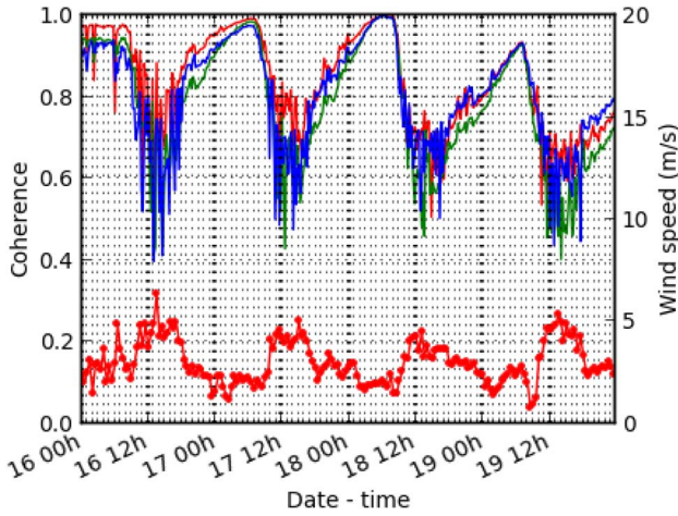
Fig. 9. Temporal coherence over four days during a dry period (full forest in the rainy season). HH, VV, and HV are in red, blue, and green in the upper curves, and wind speed is in the bottom.
