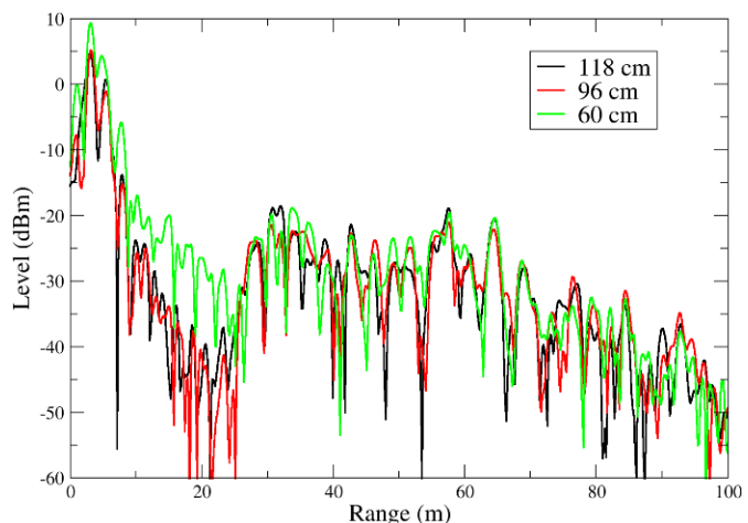
Fig. 4. Backscattering profiles from the tower top toward the West, for 3 spacing between antennas: 60 cm, 96 cm and 118 cm. The frequency band is 400-600 MHz, the antennas depression is 30°, the polarization is HH, and the corner reflector is at a range of 57 m.
