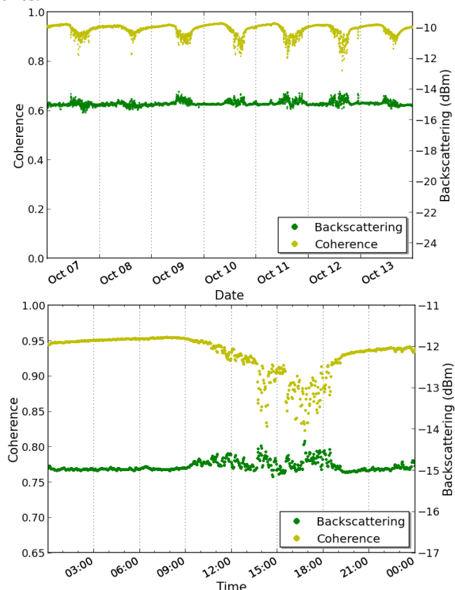
Fig. 10. Focus of RCS and coherence for a week without rain of TS-AUTUMN (top), with zoom on October the 10th (bottom).
