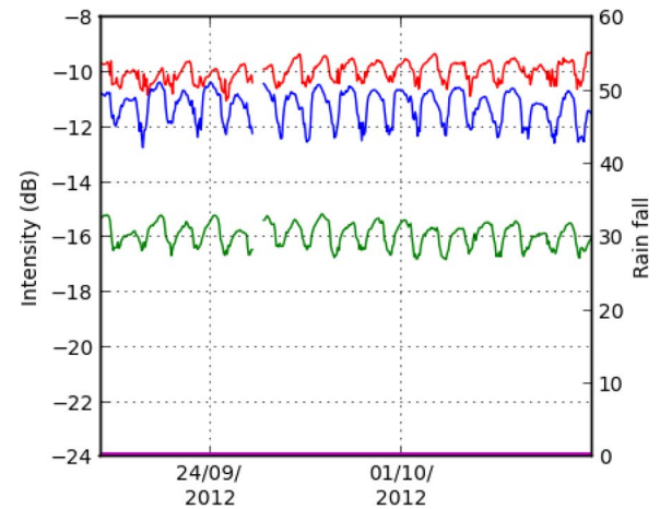
Fig. 18. Time series of the backscattering coefficient computed over the full forest during the dry period. The red curve corresponds to the HH polarization, the blue to the VV, and the green to the HV one. The purple curve corresponds to the rainfall (mm).
