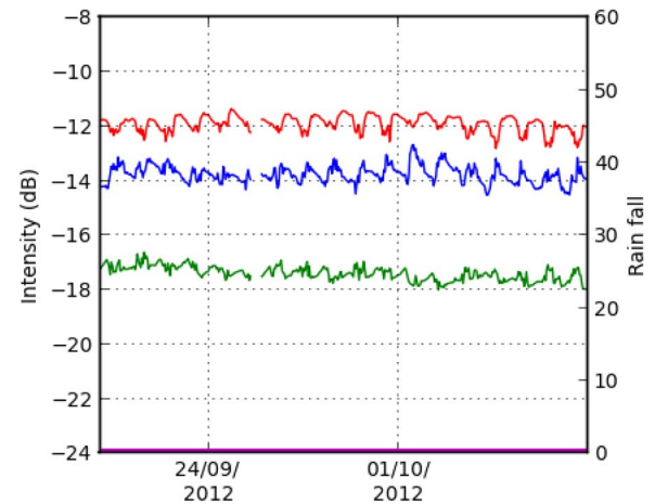
Fig. 17. Time series of the backscattering coefficient computed over the canopy (“volume only”) during the dry period. The red curve corresponds to the HH polarization, the blue to the VV, and the green to the HV one. The purple curve corresponds to the rainfall (mm).
