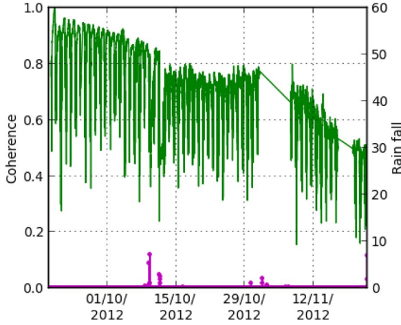
Fig. 13. Temporal coherence for HV over two months (full forest during the dry season). The x -axis corresponds to the time. Rainfall (mm) is in purple.
