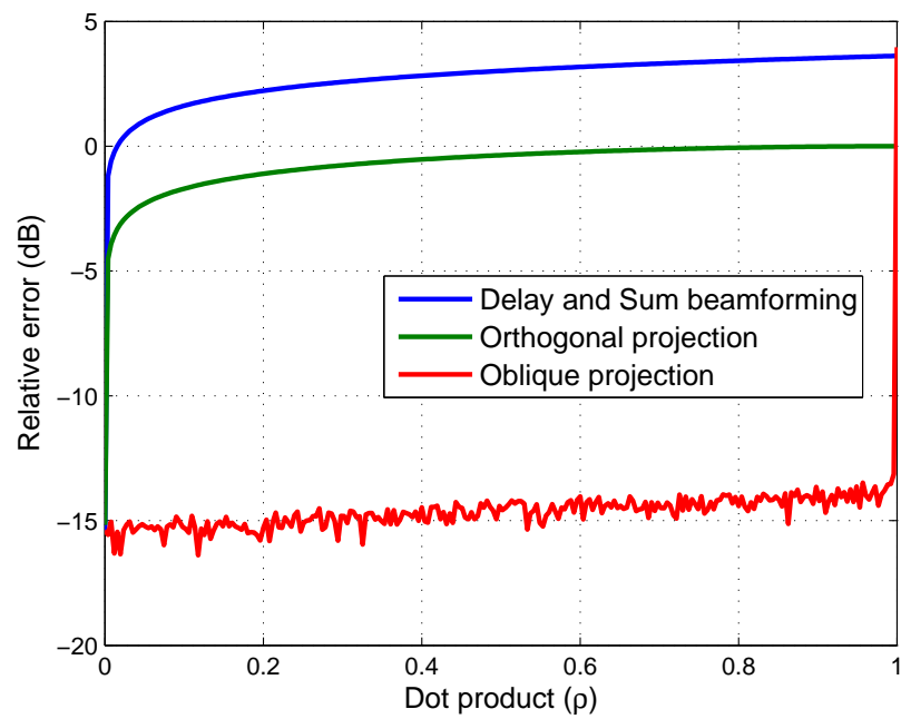
Figure 3.10: Relative error of the Delay and Sum beamforming, Orthogonal and Oblique projection beamforming techniques. M = 60 randomly distributed antennas, noise-free model, one cosmic source (power = -5 dB), one interference (Interference to Signal Ratio = +30 dB), averaged over 512 trials.
