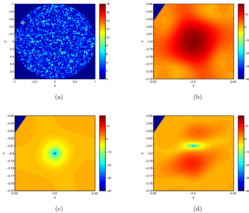
Figure 4.12: Impact of interference subspace estimation error on a skymap. Skymaps are given in dB. (a) Simulated skymap containing one interference. (b) Zoom on the interference location. (c) Zoom on the interference location after orthogonal projection based on the true interference steering vector. (d) Zoom on the interference location after orthogonal projection based on the (badly) estimated interference steering vector.
