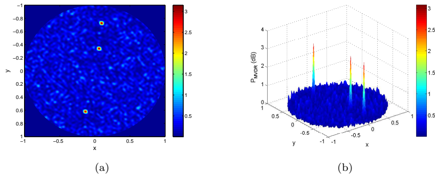
Figure 4.11: Minimum Variance Distortionless Response. Skymaps are given in dB. (a) Simulated skymap with three interferences impinging a 48-antenna array (INR = 0 dB). (b) MVDR constraint function. Three peaks can be found and represent the directions of arrival of the three impinging interferences.
