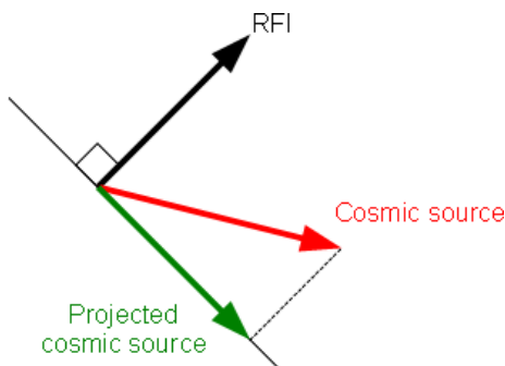
Figure 3.8: Illustration of the orthogonal projection applied to a 2-dimensional data vector space
