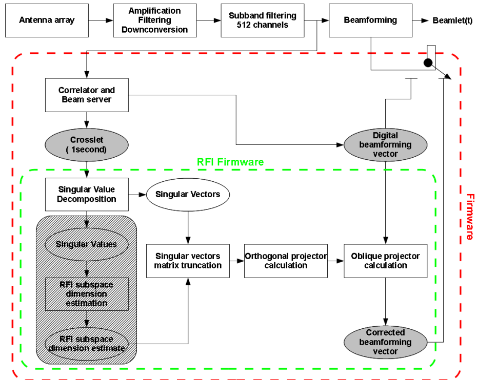
Figure 5.31: RFI mitigation algorithm implementation. The EMBRACE back end provides a crosslet matrix each second and calculates a digital beamforming vector to be applied after the analog beamforming stage. The oblique projection algorithm is based on both data and provides a corrected beamforming vector.
