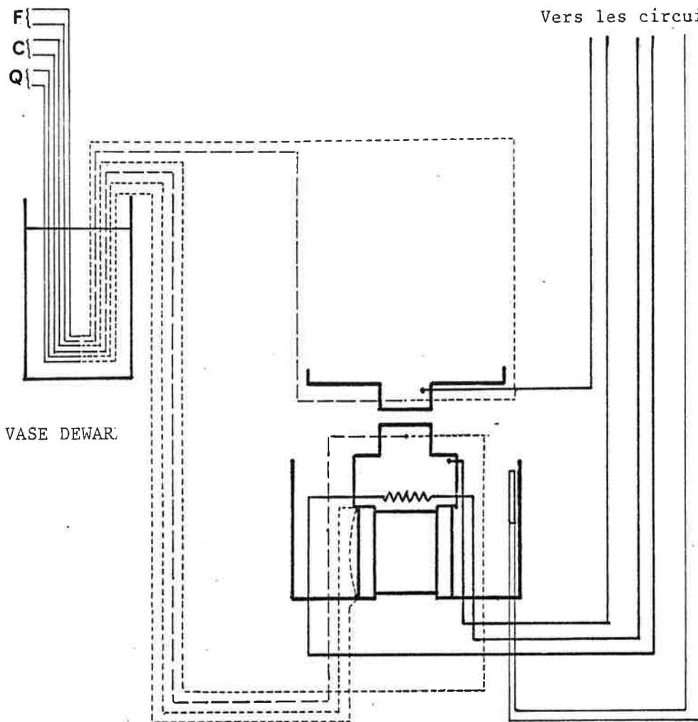
SCHEMA ELECTRIQUE
