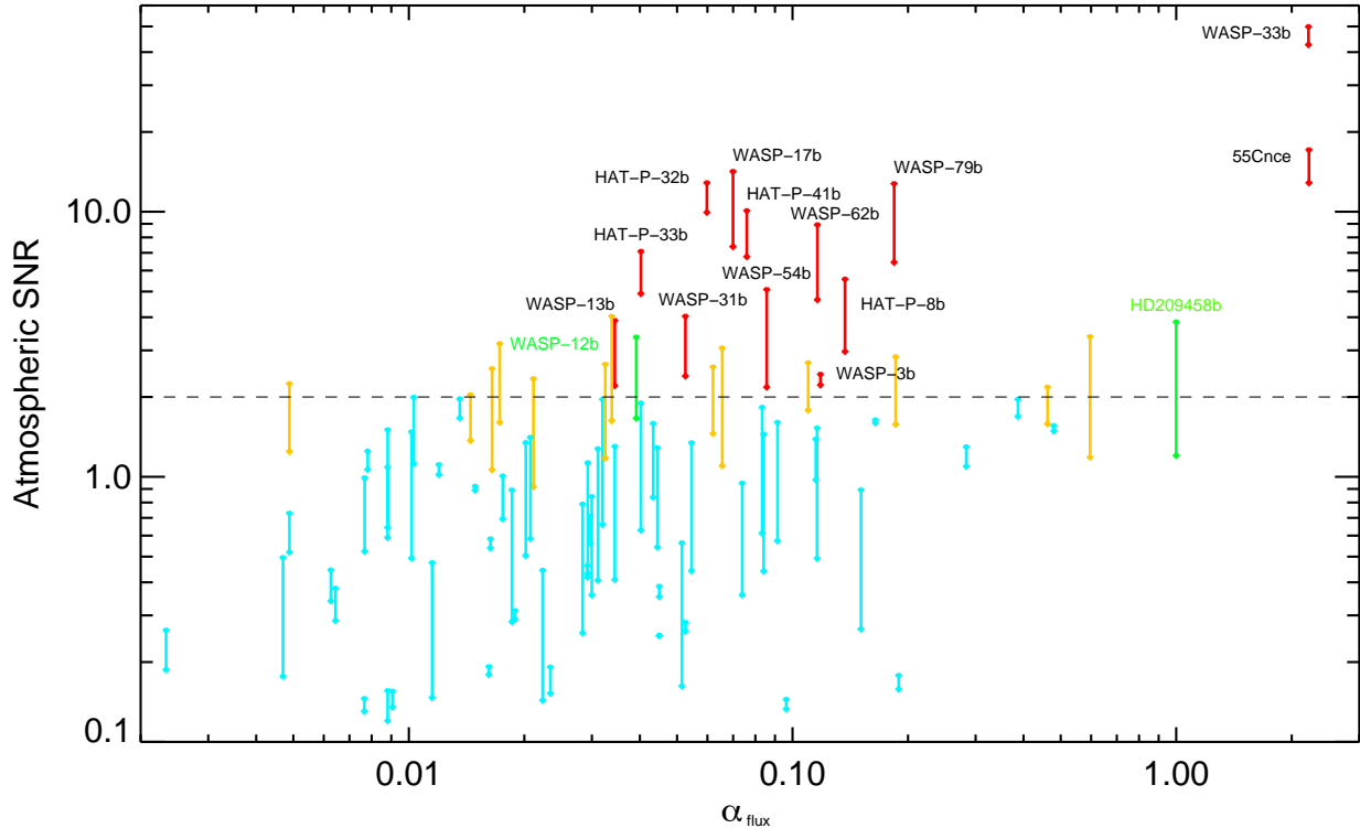
Fig. 5. SNR of absorption signatures generated by neutral magnesium in the atmospheres of transiting exoplanets, as a function of the brightness of their host-stars in the Mg I line seen from Earth. For each planet the lower (resp. upper) SNR value corresponds to a heating efficiency \eta=30\% (resp. 100\% ). Planets with SNR greater than 2 for \eta=30\% are plotted in red, and planets with SNR greater than 2 for higher heating efficiencies are plotted in orange. Other planets are plotted in blue, except for the specific hot-Jupiters HD 209458 b and WASP-12 b in green.
