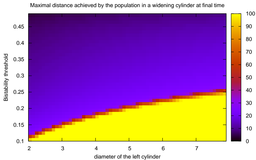
Figure 4.30 – Maximal distance \mathcal{M}_d(t) , at t = 200 , for each diameter \varepsilon \in [2; 7.8] and each bistability threshold \theta \in [0.1; 0.5] .
