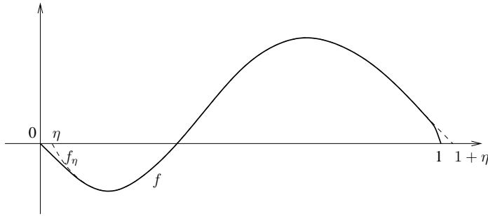
Figure 3.5 – Example of function f_\eta that satisfies (3.17).
