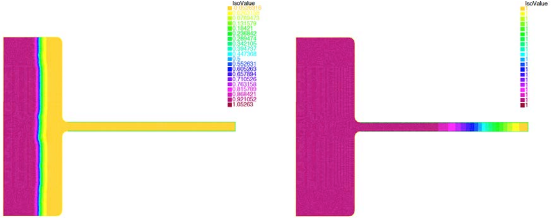
FIGURE 17 – In the case of a narrowing cylinder, the wave propagates in the entire domain. From left to right : value of the solution u for increasing values of t . In yellow areas the solution is close to 0 and in purple areas the solution is close to 1
